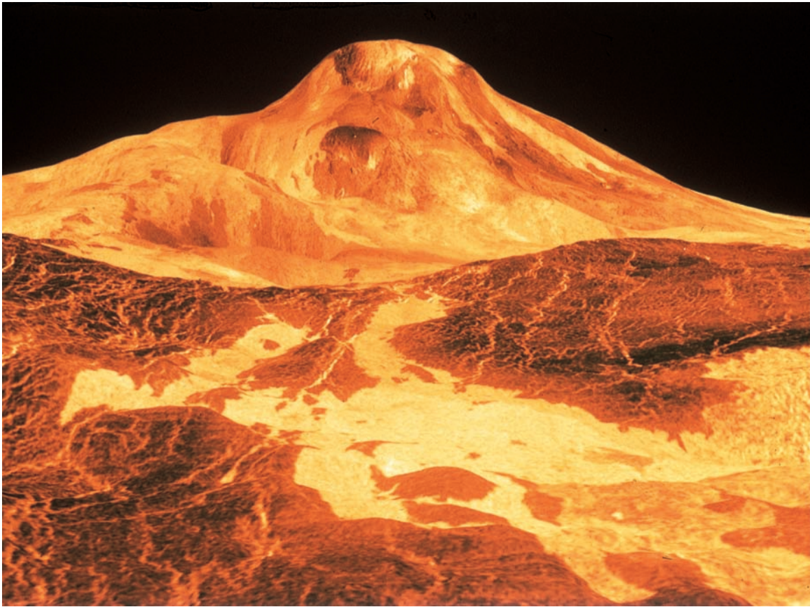
Fig. 2.30 Maat Mons, a volcano on Venus This three-dimensional perspective of Maat Mons on Venus was obtained from radar data taken from the Magellan spacecraft in October 1991. The volcano is 8 kilometers high, the second highest peak on the planet. Fresh, dark lava extends for hundreds of kilometers in the foreground, perhaps flowing from a relatively recent eruption. Maat Mons is a giant shield volcano similar in size and shape to the big island of Hawaii. Maat is the name of the ancient Egyptian goddess of truth and justice, and Mons is the Latin term for “mountain”. The orange tint simulates the color of sunlight at ground level after filtering by the dense, thick atmosphere of Venus. (Courtesy of NASA/JPL)
