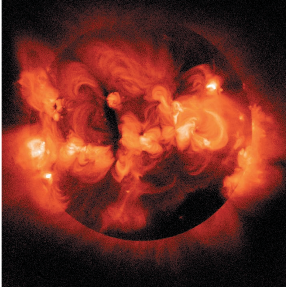
Fig. 4.25 The Sun in X-rays The bright glow seen in this X-ray image of the Sun is produced by ionized gas at a temperature of a few million kelvin. It shows magnetic coronal loops that thread the corona and hold the hot gas in place. The brightest features are called active regions and correspond to the sites of the most intense magnetic field strength. The Soft X-ray Telescope (SXT) aboard the Japanese Yohkoh satellite recorded this image of the Sun's corona on 1 February 1992, near a maximum of the 11-year cycle of solar magnetic activity. Subsequent SXT images, taken about five years later near activity minimum, show a remarkable dimming of the corona when the active regions associated with sunspots have almost disappeared, and the Sun's magnetic field has changed from a complex structure to a simpler configuration. (Courtesy of Gregory L. Slater, Gary A. Linford, and Lawrence Shing, NASA, ISAS, the Lockheed-Martin Solar and Astrophysics Laboratory, the National Astronomical Observatory of Japan, and the University of Tokyo.)
