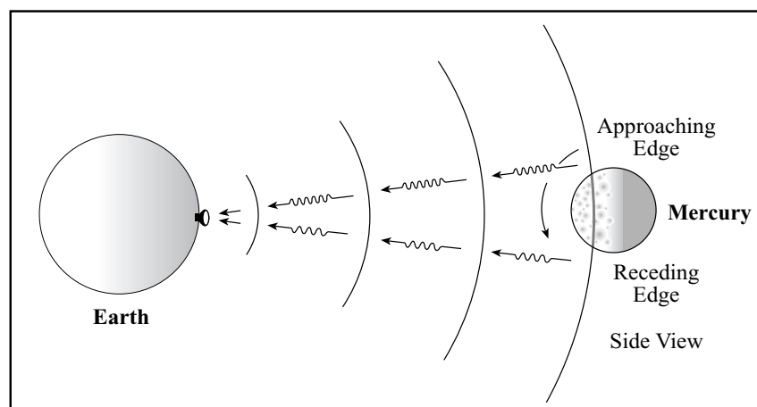
Fig. 6.3 Radar probes of Mercury A radio signal spreads out as a spherical wave, and Mercury intercepts only a small fraction of them. As the wave sweeps by the planet, it is reflected in spherical wavelets whose wavelengths are Doppler-shifted by the rotational motion of Mercury's surface. The waves from the receding side are red-shifted towards longer wavelengths and those from the approaching side are blue-shifted to shorter wavelengths. The total amount of wavelength change, from red to blue, reveals the speed of rotation, and the rotation period can be obtained by dividing the planet's circumference by this speed.
