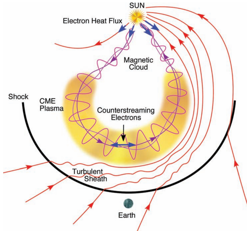
Fig 4.27 Magnetic cloud from the Sun hits the Earth When a coronal mass ejection travels into interplanetary space, it can create a huge magnetic cloud containing bidirectional, or counterstreaming, beams of electrons that flow in opposite directions within the magnetic loops that are rooted at both ends in the Sun. The magnetic cloud also drives an upstream shock ahead of it. Magnetic clouds are only present in a subset of observed interplanetary coronal mass ejections. (Courtesy of Deborah Eddy and Thomas Zurbuchen.)
