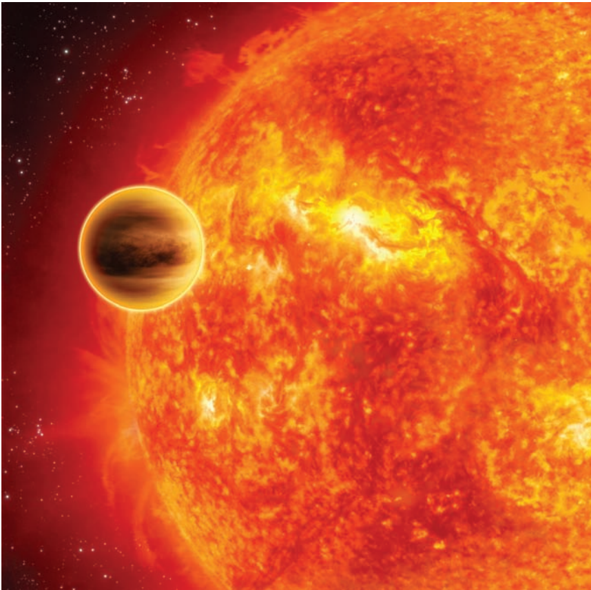
Fig. 16.11 Alien world with an atmosphere An artist's portrayal of a giant Jupiter-size planet passing in front of the star HD 189733b, which lies about 63 light-years away. It is so close to its parent star that it takes just over two days to complete an orbit. In 2007, the spectral signatures of water vapor were observed in the atmosphere of the hot, transiting exoplanet using an instrument aboard the Spitzer Space Telescope , and confirmed by observations from the Hubble Space Telescope , which also revealed molecules of methane and carbon dioxide. Also in 2007, a spectrograph on the small ground-based InfraRed Telescope Facility, with a mirror diameter of just 3.0 meters, was used to detect carbon dioxide and methane in the atmosphere of HD 189733b. Although these organic molecules are also found in living things on Earth, the planet is so massive and so hot that it is considered an unlikely habitat for life. (Courtesy of ESA/C. Carreau.)
