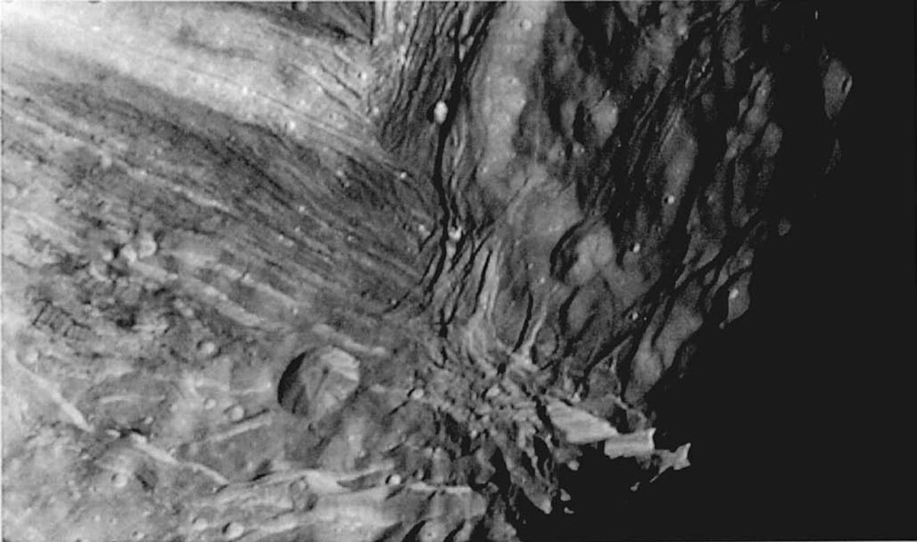
Fig. 11.12 Miranda The innermost large moon of Uranus, Miranda, is seen at close range in this Voyager 2 image, which was taken on 24 January 1986. The great variety and directions of the fractures and troughs, and the different densities of impact craters on them, signify a long, violent history for Miranda. Two distinct types of terrain are visible. They are rugged, higher-elevation terrain, disappearing into the shadows ( upper right ), and the lower-elevation, striated terrain ( upper left ). The light gray cliff ( bottom right ) is 20 kilometers high; the larger crater ( lower middle ) is about 25 kilometers across. (Courtesy of NASA/JPL.)
