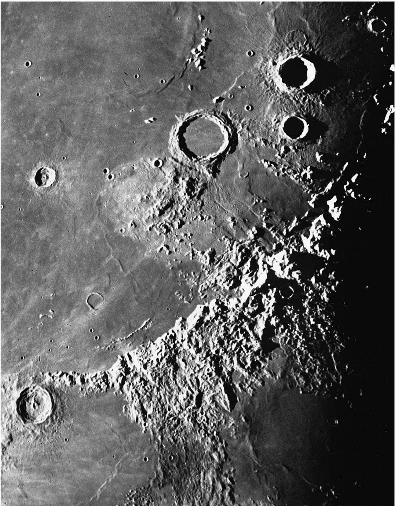
Fig. 2.21 The Moon's Apennine mountains The radial structure and steep inner slopes of these mountains ( lower right ) mark a section of the outer rim of the Imbrium Basin. The huge excavation was subsequently filled with lava to form the smooth Mare Imbrium and partially submerge the inner ring of mountains ( upper left ). The smaller circular craters include Timocharis, which is also shown in Fig. 2.19 and is about 34 kilometers in diameter ( center left ) and the largest round structure Archimedes ( upper center ) with a diameter of 83 kilometers. (Photo courtesy of UCO/Lick Observatory.)
