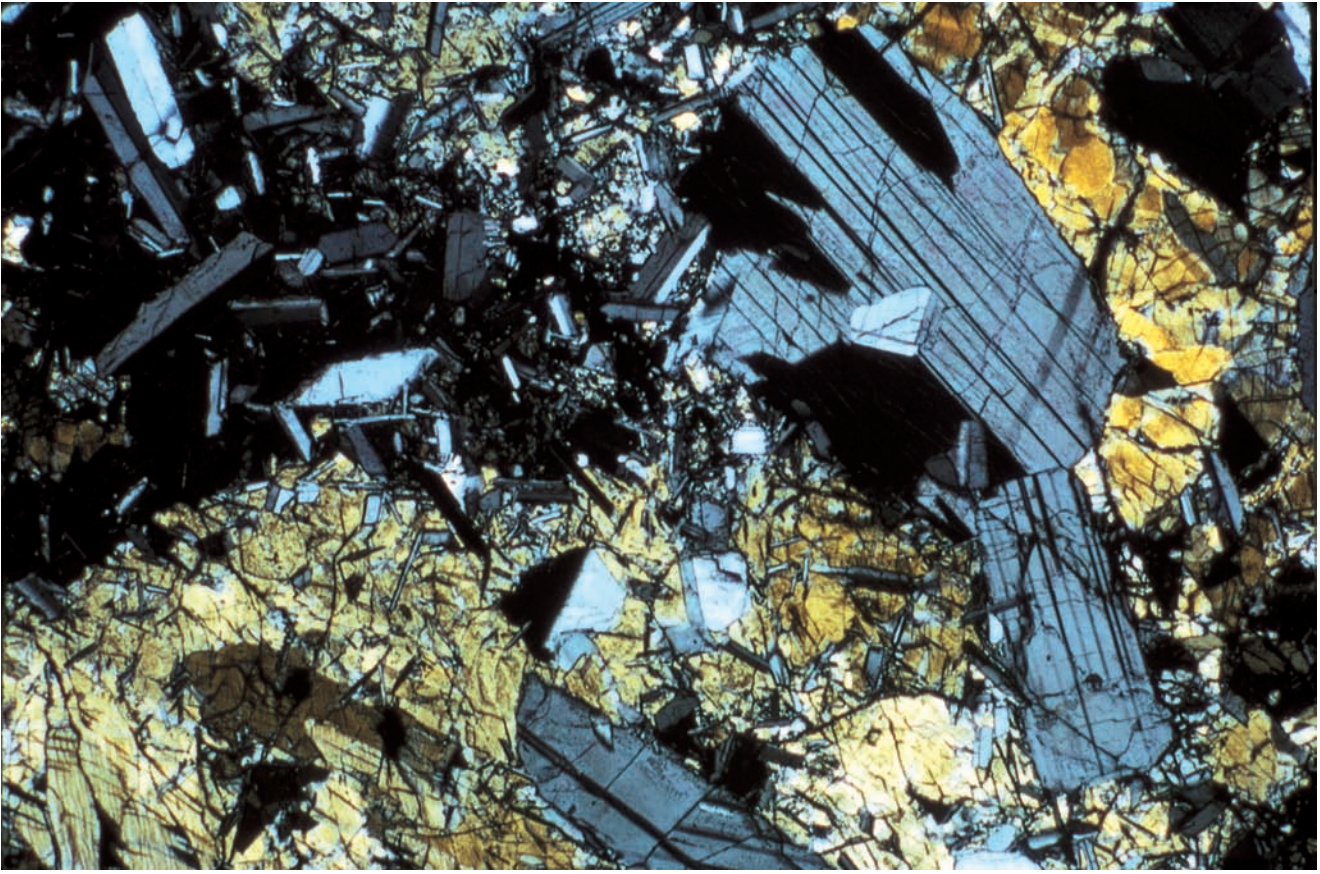
Fig. 12.22 Achondrite meteorite A photomicrograph of the achondrite meteorite that fell near Juvinas, France, on 15 June 1821. It contains basalt, resulting from the melting and separation of material inside an asteroid-size parent body. The section shown here is 0.0032 meters across. (Courtesy of Martin Prinz, American Museum of Natural History.)
