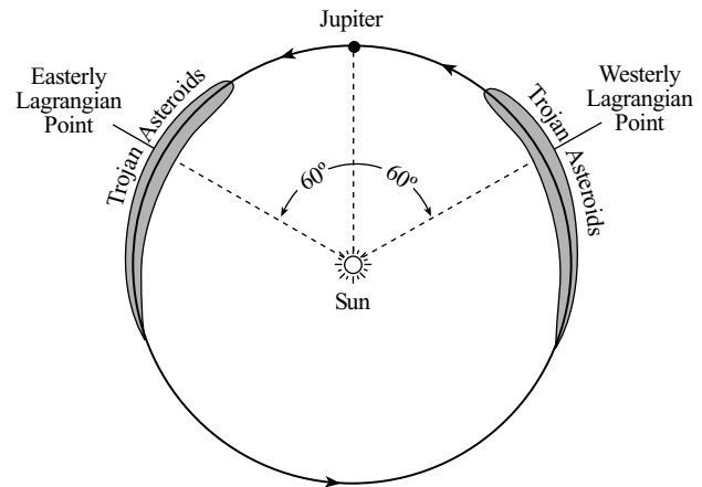
Fig. 12.1 Trojan asteroids Asteroids that share Jupiter's orbit are known as the Trojan asteroids. They are located near the point where the gravitational force of Jupiter and the Sun are equal. The gravitational perturbations of the inner planets produce slight swinging motions, so the Trojan asteroids oscillate within the two shaded regions. Some of the Trojan asteroids may occasionally move close enough to be captured by Jupiter's gravity, thereby accounting for the planet's unusual outer satellites.
