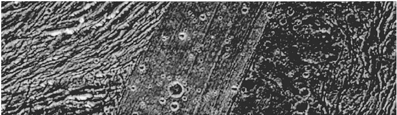
Fig. 9.22 Ganymede close up The bright icy crust on Jupiter's moon Ganymede contains both young and old terrain with bright grooves, caused by internal stress, and craters due to external impact. The youngest terrain ( center ) is finely striated and relatively lightly cratered. The oldest terrain ( right ) is rolling and relatively heavily cratered. The highly deformed grooved terrain ( left ) is of intermediate age. This image, approximately 89 kilometers across, was taken from the Galileo spacecraft on 20 May 2000. (Courtesy of NASA/JPL.)
