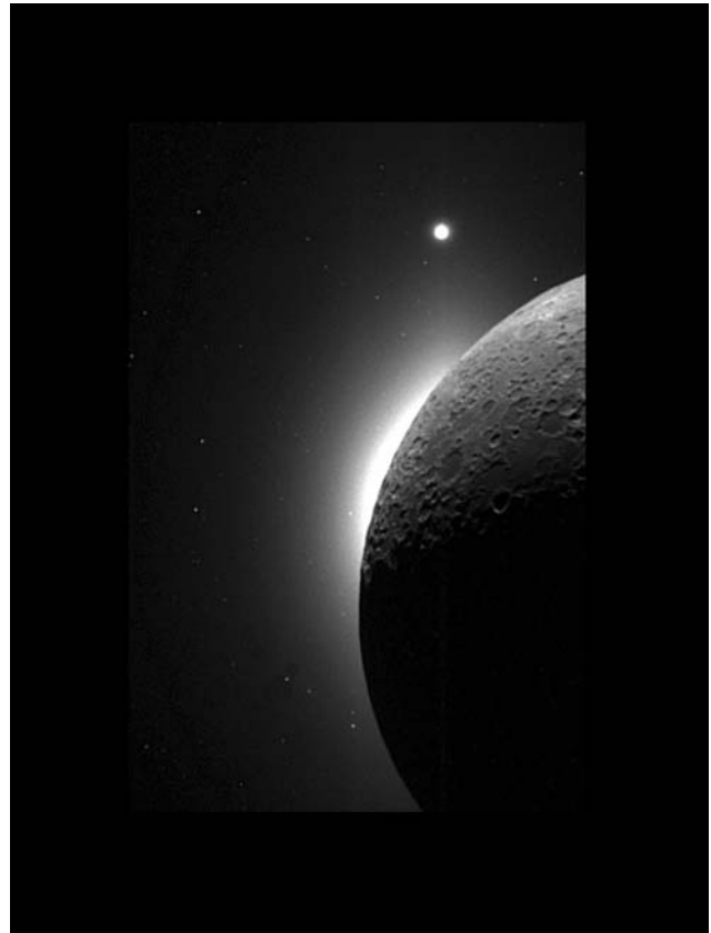
Fig. 5.24 Clementine observes the Moon, Sun, and Venus In this image, taken from the Clementine spacecraft in 1994, the Sun is just behind the Moon's limb, or edge, so most of the lunar surface is illuminated by light reflected from the Earth, known as Earthshine. Light from the Sun's outer atmosphere, the solar corona, produced the bright glow on the lunar horizon. The planet Venus is seen at the top of the frame. (Courtesy of NASA/JPL/USGS.)
