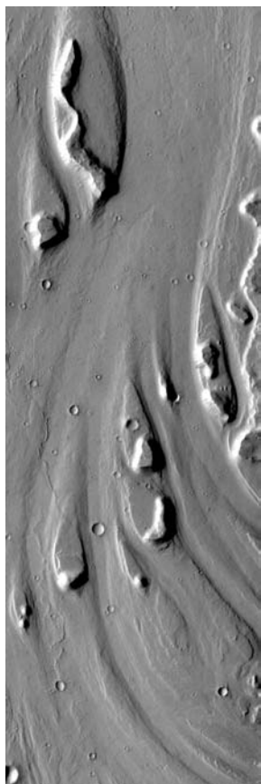
Fig. 2.42 Ancient water flow in Mars' Ares Vallis As shown in this image, obtained from an instrument aboard the 2001 Mars Odyssey orbiter, large quantities of water were diverted around pre-existing craters in Ares Vallis. As the water made its way downstream, the interference with the flow was reduced, and the water flow reformed at the narrow ends of the islands. The orientation of the islands therefore indicates the direction of flow, with the narrow end of the island pointing downstream. In this case, the flow is from the lower right to upper left. Ares Vallis is an outflow channel opening on to the Chryse Planitia, landing site of Mars Pathfinder (see Figs. 2.14 and 2.15). Ares is the Greek god of war, and possibly connected with the Roman god Mars. (Courtesy of NASA/JPL/ASU.)
