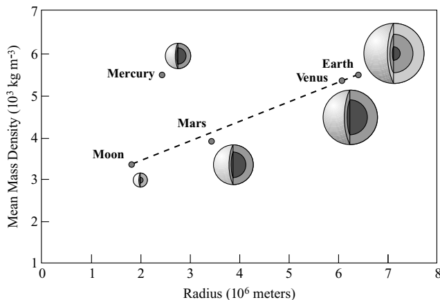
Fig. 6.17 Radius, mass density and interior structure of terrestrial bodies Mercury is an anomaly in this comparison of size and mean mass density. Mercury is just slightly bigger than the Moon and a little smaller than Mars, but its mean mass density is comparable to that of the larger terrestrial planets, Earth and Venus. As shown in the internal cross-sections, Mercury's unexpectedly large mass density is due to a large dense core extending up to 75 percent of its radius. The Moon's core occupies just 20 percent of its radius. The Earth's inner and outer core take up 55 percent of its radius, while that of Mars is smaller.
