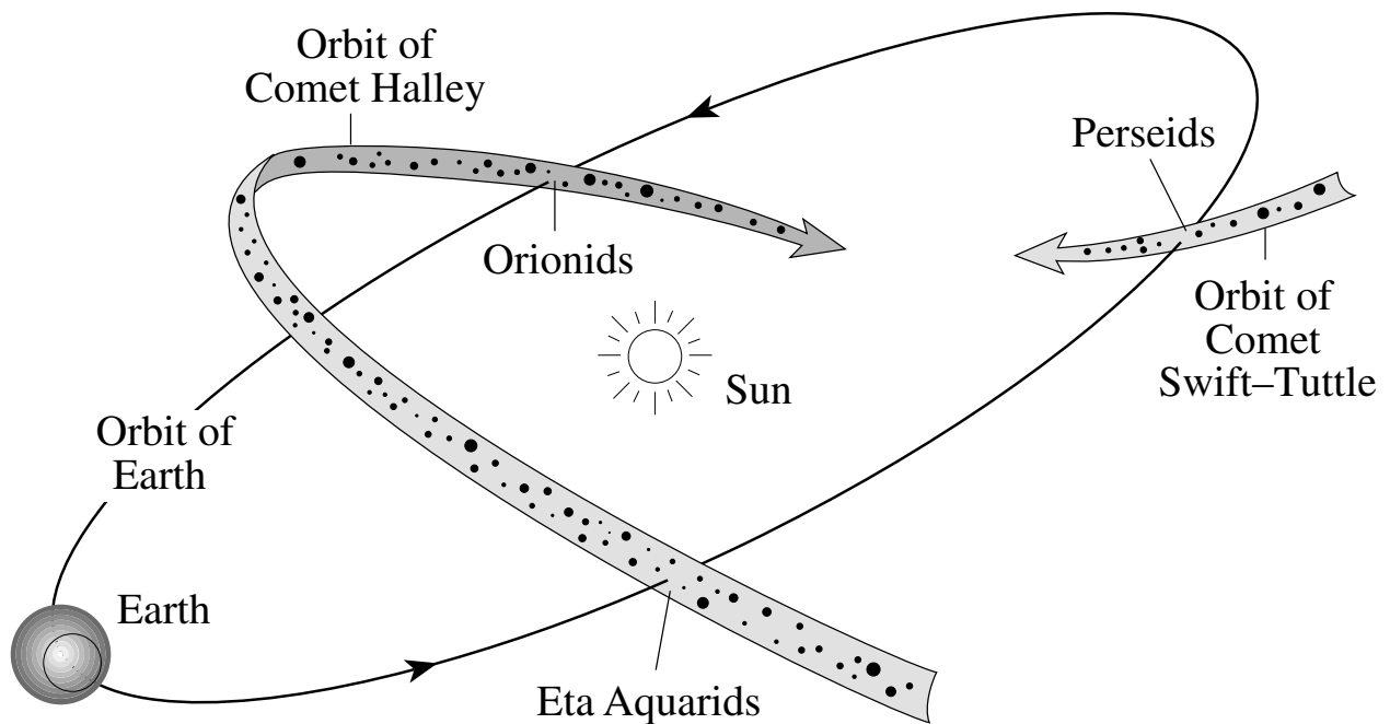
Fig. 14.27 Comets produce meteor showers The Earth's orbit intersects a stream of meteoric material left along the orbit of comet Halley, producing two meteor showers, the Eta Aquarids in May and the Orionids in October. Other comets intersect the Earth's orbit just once during their trip around the Sun. Annual meteor showers are created when the Earth enters the intersection point, such as the August Perseids produced by debris from comet Swift-Tuttle. The orbit of comet Halley is inclined by 162 degrees with respect to the ecliptic, the plane of the Earth's orbit, while the orbit of comet Swift-Tuttle has an inclination of 114 degrees.
