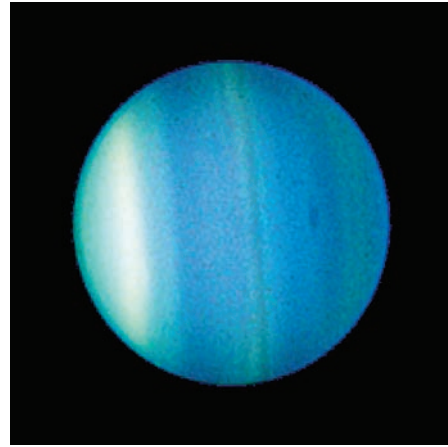
Fig. 11.2 Bands and vortex in the atmosphere of Uranus
