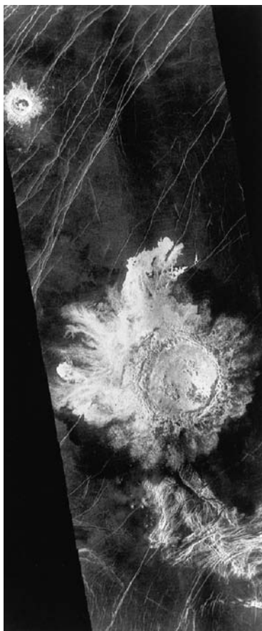
Fig. 7.14 Stuart Crater This beautiful crater exhibits asymmetric radar-bright ejected material attributed to an oblique impact and interaction with the dense, thick atmosphere of Venus. The crater's rim, which is 67 kilometers in diameter, encircles a bright floor that may have unique physical properties. This impact crater's name honors Mary Stuart, Queen of Scots (1542–1587). (Courtesy of NASA/JPL.)
