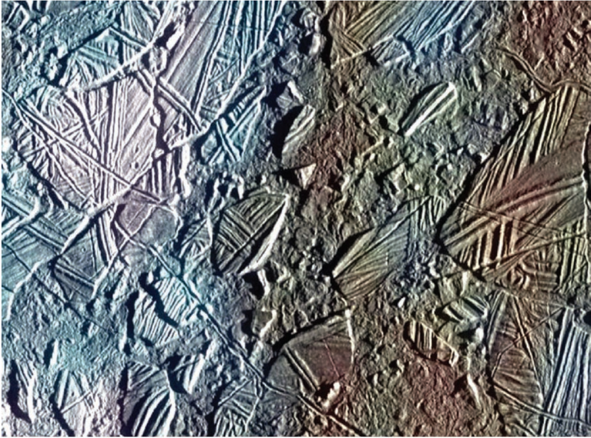
Fig. 9.20 Jupiter's moon Europa under stress This mosaic of the Conamara Chaos region on Europa indicates relatively recent resurfacing of the moon. Many sets of parallel and crosscutting ridges and fractures are detected. They are the frozen remnants of surface tension and compression, probably produced by heating and upwelling from below. The break-up and movement of the existing crust have formed irregularly shaped blocks of water ice. The blocks have been shifted, rotated, and even tipped and partially submerged within some lubricating material at the time of disruption, most likely soft ice or liquid water, or an ice-and-water slush below the surface. Some of the blocks have acted like rafts, separating and moving into new positions, somewhat like pack ice in the Earth's polar seas. The presence of young fractures cutting through this region indicates that the surface froze again after the resurfacing, forming solid, brittle ice. This image was taken from the Galileo spacecraft in February 1997. (Courtesy of NASA/JPL)
