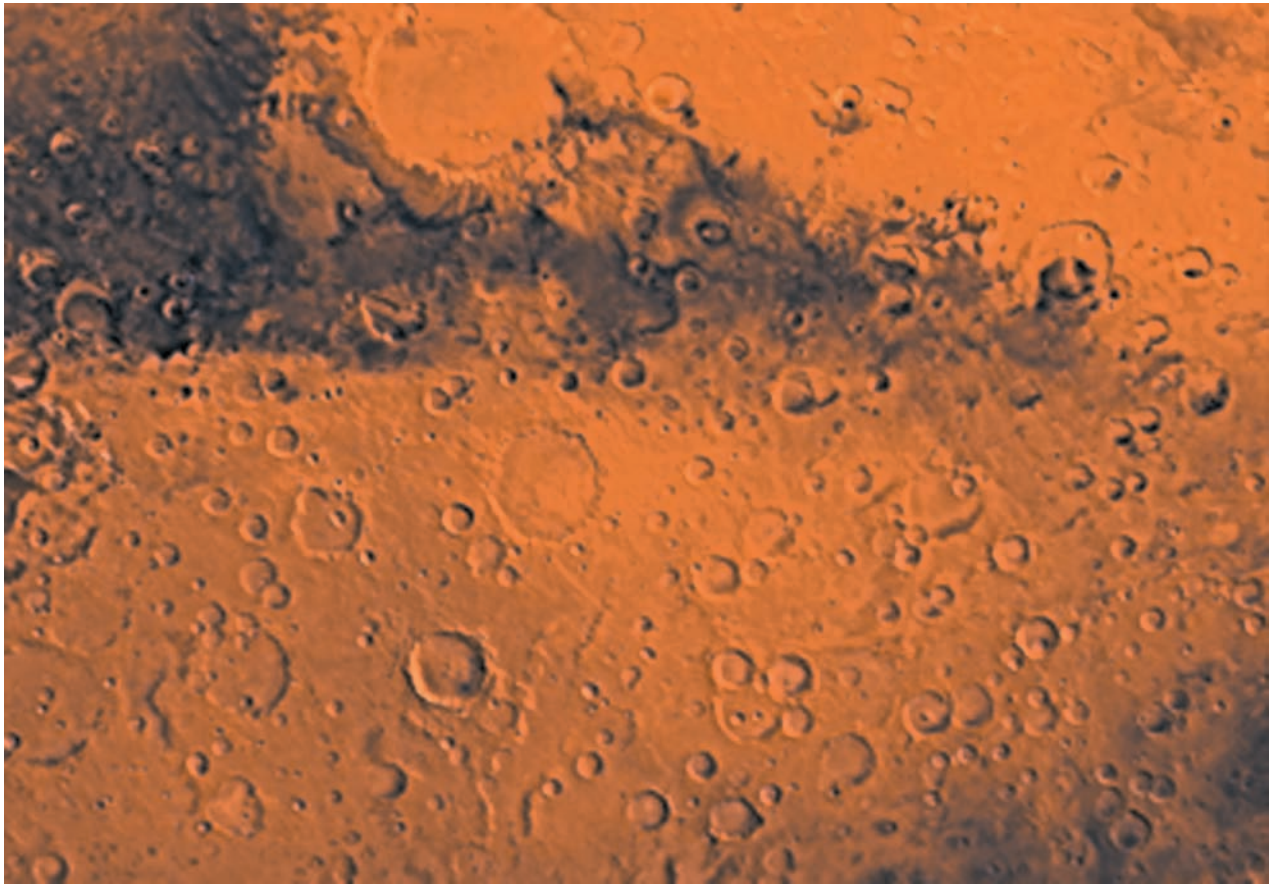
Fig. 8.14 Mars' Sinus Sabeus quadrangle Heavily cratered highlands dominate the Sinus Sabeus region of Mars, located just south of the equator between 0 and -30 degrees latitude. A large impact crater named after the Italian astronomer Giovanni Schiaparelli (1835-1910) marks the northern part of this mosaic image, taken from the a Viking orbiter. (Courtesy of NASA/JPL/USGS.)
