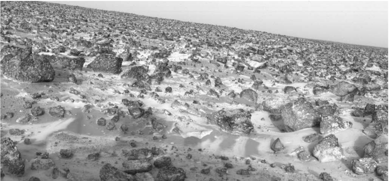
Fig. 8.6 Frost on Mars Atmospheric water vapor freezes onto the surface of Mars, producing a very thin coating of water ice on rocks and soil photographed from the Viking 2 lander at its Utopia Planitia landing site on 18 May 1979. Scientists believe dust particles in the atmosphere pick up bits of solid water; carbon dioxide, which makes up 95 percent of the Martian atmosphere, freezes and adheres to the particles and they become heavy enough to sink. Warmed by the Sun, the surface evaporates the carbon dioxide and returns it to the atmosphere, leaving behind the water and dust in the white patches of frost shown here. The frost remained on the surface for about 100 Earth days. (Courtesy of NASA/JPL)
