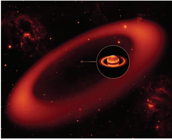
Fig. 10.30 Saturn's enormous infrared ring This artist's conception illustrates the infrared glow of cold dust particles in Saturn's largest ring, discovered using the Spitzer Space Telescope in 2009. The very tenuous collection of ice and dust particles is spread out in an enormous belt at the far reaches of Saturn's system, with an orbit tilted 27 degrees from the main ring plane. The bulk of its material starts about 6 million kilometers away from the planet, and extends outward another 12 million kilometers. The ring's diameter is equivalent to roughly 300 times the diameter of Saturn. The planet appears as just a small dot in the middle of this portrayal. The inset shows an enlarged image of Saturn, as seen by the W. M. Keck Observatory at Mauna Kea, Hawaii, in infrared light. Saturn's retrograde moon Phoebe circles within the newfound ring, and is likely to be the source of its material. Dark material dislodged from Phoebe may also be the source of the dark side of Saturn's next innermost moon, two-faced Iapetus. (Courtesy of NASA/JPL-Caltech/Keck.)
