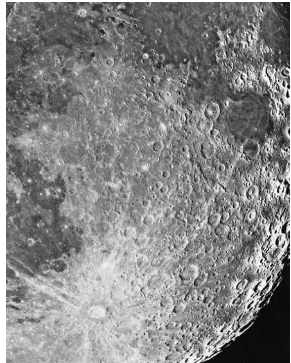
Fig. 5.14 Lunar rays White rays splash out across the Moon from crater Tycho ( bottom center of this image ). Tycho is a large, young crater with a diameter of 85 kilometers and an age of 108 million years. Only relatively recent craters retain their white rays, for those of older craters are darkened and worn away by continued meteorite impact. The dark, flat circular feature in the upper right is Mare Nectaris (Sea of Nectar). This clear image was produced using the unsharp masking technique that permits high contrast and fine resolution. (Anglo-Australian Telescope © 1976. Photo prepared by David F. Malin.)
