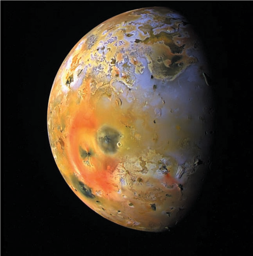
Fig. 2.33 Volcanic activity on Io Massive eruptions continuously disfigure the surface of Jupiter's satellite Io, the most volcanically active body in the solar system. As shown in this color-enhanced image, taken from the Galileo spacecraft on 19 September 1997, Io's surface is continuously being covered by lava flowing from its volcanoes, erasing any impact craters. A bright red ring surrounds the volcano Pele, marking the site of sulfur compounds deposited by its volcanic plumes. A dark circular area, about 400 kilometers in diameter, intersects the upper-right part of the red ring and surrounds another volcanic center named Pillan Patera. Deposits of sulfur dioxide frost appear white and gray in this image, while other sulfurous materials probably cause the yellow and brown shades. Pele is the Hawaiian goddess of the volcano, and Pillan Patera is named for the Araucanian thunder, fire and volcano god. (Courtesy of NASA/JPL/U. Arizona.)
