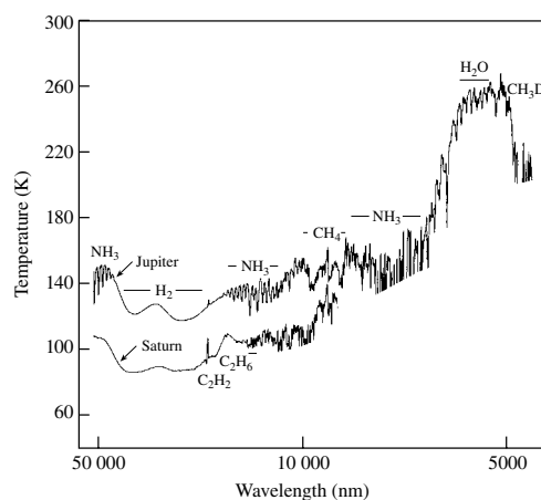
Fig. 3.5 Molecules in the atmospheres of Jupiter and Saturn
