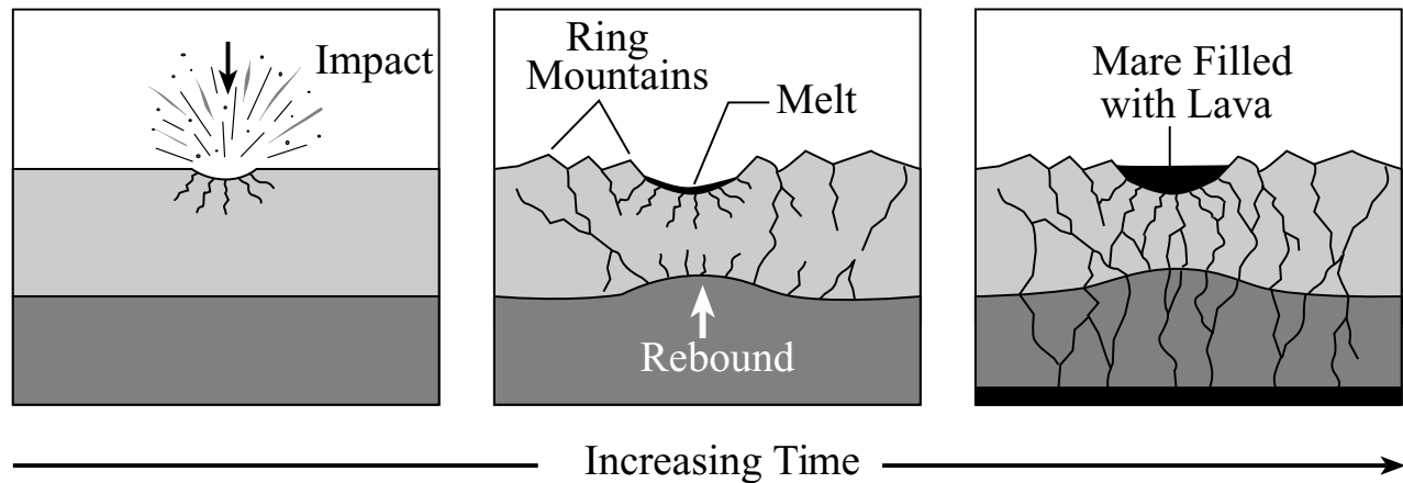
Fig. 5.28 Mare formation on the Moon Disintegrating and vaporizing as it strikes, a meteorite blasts a huge impact basin out of the lunar surface ( left ), while the associated shock waves create fractures in the rock beneath the basin. The blast hurls up mountain ranges around the basin ( middle ), and the underlying rock adjusts to the loss of mass above it by rebounding upward. The uplifted mantle causes additional fractures in the rock, while a pool of shock-melted rock solidifies in the basin. All the major impact basins on the Moon were created in this way between 4.3 and 3.9 billion years ago. Later, interior heat from radioactivity caused partial melting inside the Moon, and magma rose along the fractures, filling the basin with lava to form a dark mare ( right ). The lunar maria were filled by this volcanic outpouring between 3.9 and 3.1 billion years ago.
