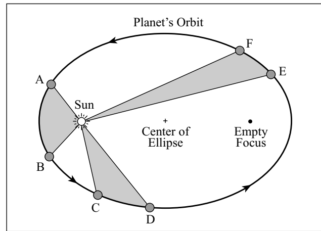
Fig. 1.12 Kepler's first and second laws Kepler's first law states that the orbit of a planet about the Sun is an ellipse with the Sun at one focus. The other focus of the ellipse is empty. According to Kepler's second law, the line joining a planet to the Sun sweeps out equal areas in equal times. This is also known as the law of equal areas. It is represented by the equality of the three shaded areas ABS, CDS and EFS. It takes as long to travel from A to B as from C to D and from E to F. A planet moves most rapidly when it is nearest the Sun (at perihelion); a planet's slowest motion occurs when it is farthest from the Sun (at aphelion).
