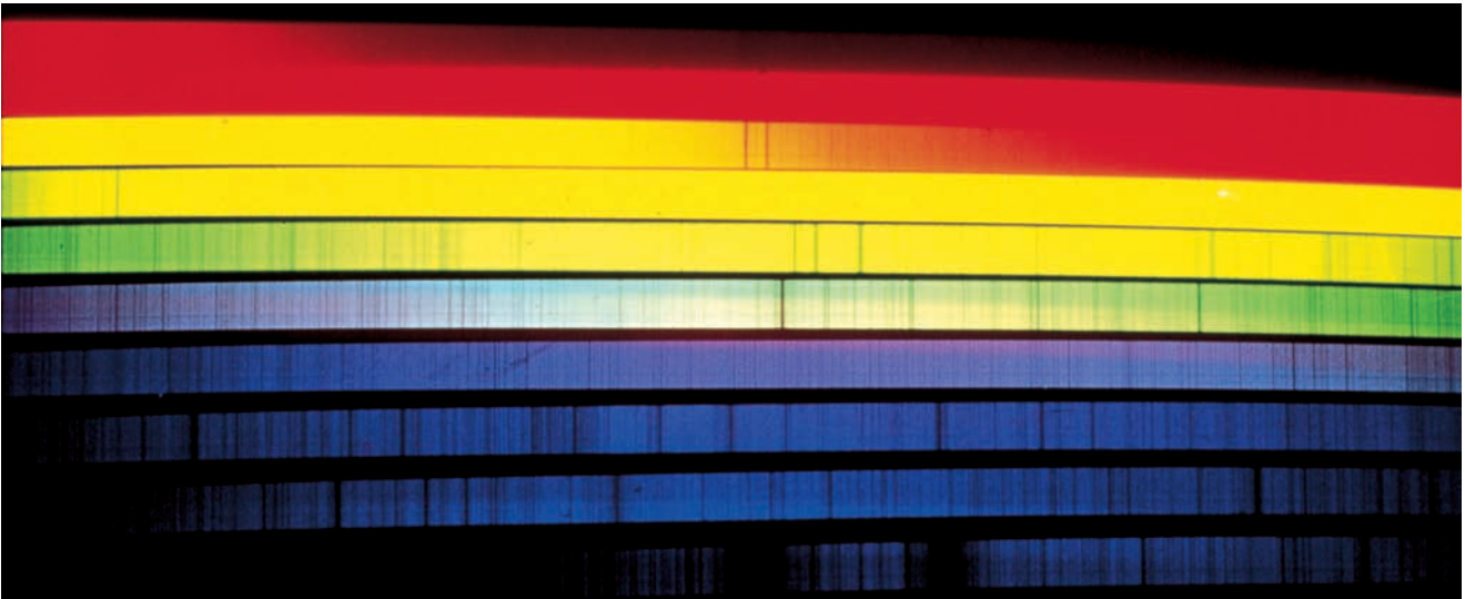
Fig. 1.21 Visible solar spectrum A spectrograph has spread out the visible portion of the Sun's radiation into its spectral components, displaying radiation intensity as a function of wavelength. When we pass from long wavelengths to shortest ones ( left to right and top to bottom ), the spectrum ranges from red through orange, yellow, green, blue and violet. Dark gaps in the spectrum, called Fraunhofer absorption lines, represent absorption by atoms or ions in the Sun. The wavelengths of these absorption lines can be used to identify the elements in the Sun, and the relative darkness of the lines helps establish the relative abundance of these elements. (Courtesy of NSO/NOAO.)
