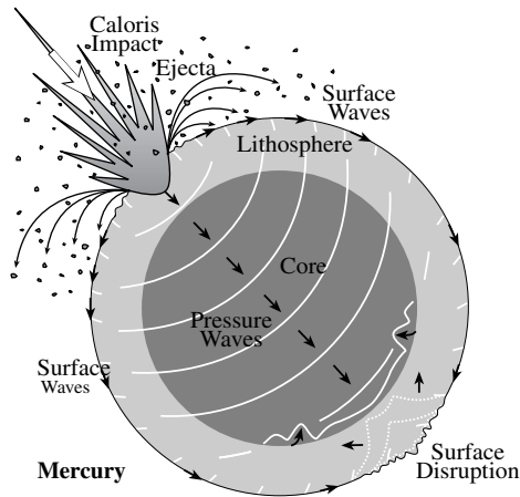
Fig. 2.23 Explosive impact on Mercury When an exceptionally large meteorite hit Mercury an estimated 3.85 billion years ago, it sent intense waves around the planet and through its core. They came to a focus on the opposite side of Mercury, disrupting the surface and producing hilly and lineated terrain there. The Caloris Basin was excavated at the impact site (also see Fig. 2.22), and it now exhibits concentric waves that froze in place after the impact.
