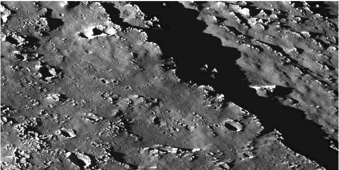
Fig. 9.26 Structures within the Valhalla impact basin on Jupiter's moon Callisto This mosaic of two images shows an area within the Valhalla region on Jupiter's outermost large moon, Callisto. Numerous impact craters, ranging in size from 155 meters to 2.5 kilometers across, are seen in the mosaic, which is approximately 33 kilometers wide. There is an unexpected absence of small craters and the ragged rims of the existing craters suggest an erosion process, which is believed to be due to sublimation of volatiles from the surface ice. A prominent dark fault scarp, or cliff, and smaller parallel ridges are also pictured ( top right ). These images were obtained on 4 November 1996 from the Galileo spacecraft. (Courtesy of NASA/JPL/ASU.)
