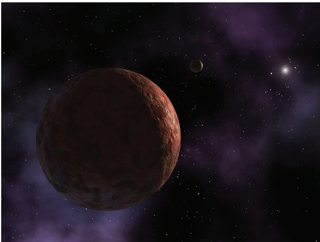
Fig. 15.7 Trans-Neptunian object In this artist's visualization, a small, cold trans-Neptunian object dubbed Sedna is shown where it resides at the outer edges of our solar system, beyond the orbit of Neptune. The object is so far away that the Sun appears as an extremely bright star instead of the large, warm disk observed from Earth. A distant, hypothetical small moon is shown above the object and nearly in the direction of the Sun. (Courtesy of NASA/JPL.)
