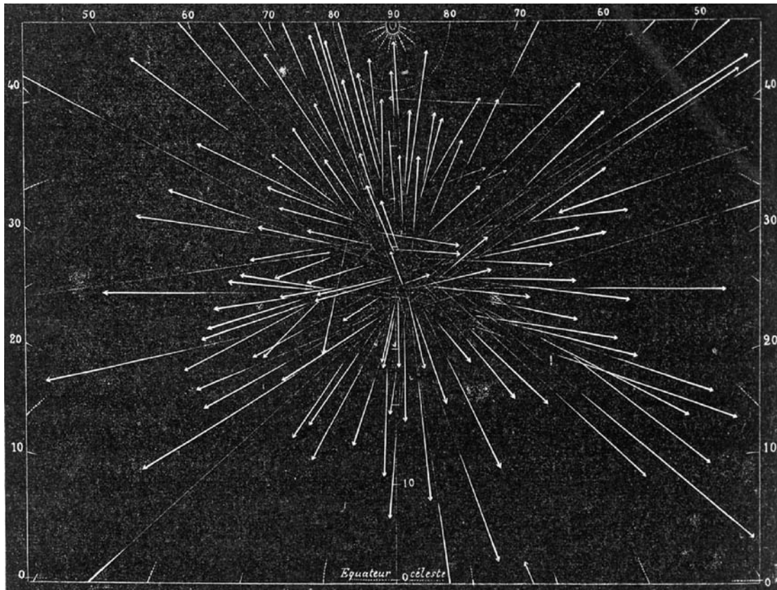
Fig. 14.28 Radiant meteors The apparent paths of shooting stars on 27 November 1872. Meteor showers are named after the constellation in which their radiant appears. This meteor shower is called the Andromedids meteor shower because its radiant appears in the constellation Andromeda. The shower occurs every November when the Earth intersects the debris that has been scattered along the orbit of Biela's comet. [Adapted from Amedee Guillemin's Le Ciel , Librairie Hachette, Paris (1877).]
