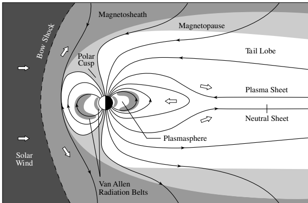
Fig. 3.14 Earth's magnetosphere The Earth, its auroras, atmosphere and ionosphere, and the two Van Allen radiation belts all lie within the Earth's magnetosphere. Similar magnetic cavities are found around other magnetized planets. Electrons and protons in the solar wind are deflected at the bow shock ( left ), and flow along the magnetopause into the magnetic tail ( right ). Electrified particles can be injected back toward the Earth and Sun within the plasma sheet ( center ).
