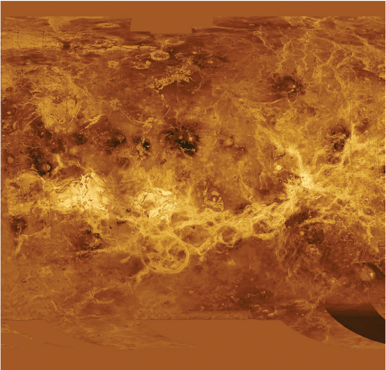
Fig. 7.10 Surface terrain of Venus The cloud-penetrating radar system aboard the Magellan spacecraft lifted the perpetual veil of thick clouds on Venus, revealing its surface features in high resolution of 120 meters in the early 1990s. The eastern half of the planet's surface is portrayed in this cylindrical map, extending between 52 and 240 degrees east longitude (left side to right side) and from 90 degrees north latitude to 90 degrees south latitude (top to bottom). (Courtesy of NASA/JPL)
