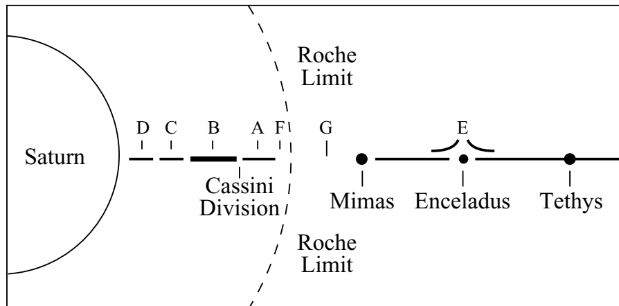
Fig. 10.12 Cross-section of rings and satellites All of Saturn's main rings lie inside the Roche limit (dashed curve) within which the planet's gravity will tear a large satellite apart. The A and B rings have been observed for centuries. The more tenuous C ring was discovered in the 19th century, and definite observations of the transparent D ring awaited the arrival of the Voyager 1 spacecraft on 12 November 1980. The icy satellite Enceladus feeds the tenuous E ring, also revealed from Voyager 1 , as well as from the Cassini spacecraft. For clarity, the thickness of the rings has been exaggerated.
