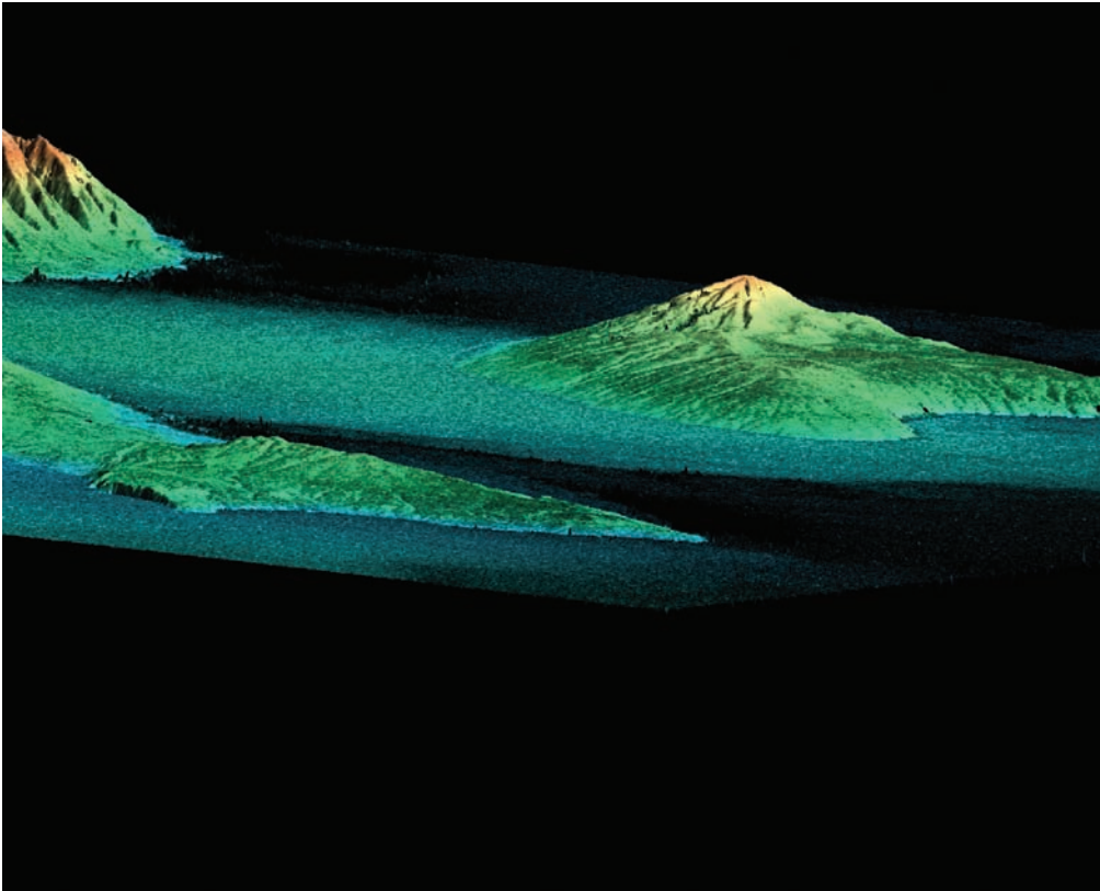
Fig. 2.26 Hawaiian Islands Molokai ( left ), Lanai ( right ), and the northwest tip of Maui ( upper left ) are shown in this radar image obtained from the Space Shuttle . These islands are now extinct volcanoes, destined to eventually erode away into sunken islands known as seamounts. (Courtesy of NASA/JPL/NIMA.)
