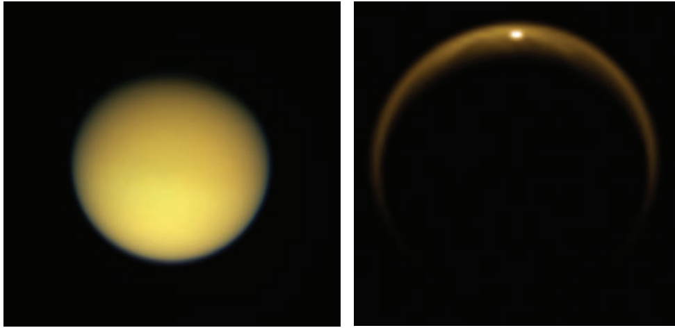
Fig. 3.8 Titan's dense, smoggy atmosphere The surface of Saturn's moon Titan is hidden from view by a hazy layer of smog, giving it a fuzzy, tennis-ball appearance in a Cassini natural-color view (left) taken on 15 February 2005. When illuminated from behind, the dense atmosphere forms a crescent. By observing radiation at infrared wavelengths, on 8 July 2009, a Cassini instrument was able to penetrate through the moon's atmosphere and catch the glint of sunlight reflected off a huge lake in the northern hemisphere of Titan (right), which is probably filled with liquid methane and ethane. The lake is named Kraken Mare. [Courtesy of NASA/JPL/SSI (left) and NASA/JPL/University of Arizona/DLR (right).]
