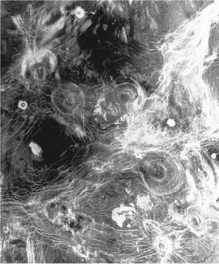
Fig. 7.18 Bereghinya Planitia This high-resolution Magellan mosaic shows an area in the low-lying plain Bereghinya Planitia, named for the Slavic water spirit. The image is 1840 kilometers wide, and centered at 45 degrees north latitude and 11 degrees east longitude. The plain's fractured surface is attributed to plumes of magma that rise from inside Venus, pushing against the planet's crust. The most prominent features are the circular and oval structures that are sometimes called arachnoids for the spider-web-like appearance of their fractures (also see Fig. 7.20). Also visible are lava flows, impact craters and volcanic domes. (Courtesy of NASA.)
