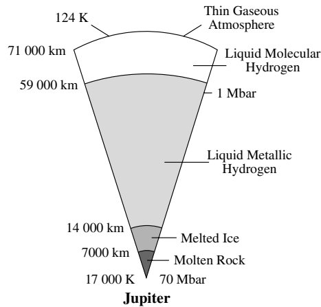
Fig. 9.8 Inside Jupiter Giant Jupiter has a thin gaseous atmosphere covering a vast global ocean of liquid hydrogen. At the enormous pressures within Jupiter's interior, the abundant hydrogen is compressed into an outer shell of liquid molecular hydrogen and an inner shell of fluid metallic hydrogen. The giant planet probably has a relatively small core of melted ice and rock.
