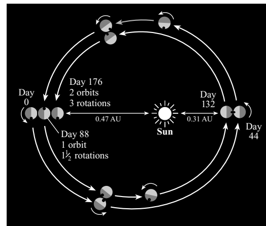
Fig. 6.5 The days are long on Mercury Because of its spin-orbit coupling, Mercury rotates once every 58.6 Earth days, and orbits the Sun in 88.0 Earth days. After two orbits the planet has rotated three times, but from Mercury's surface the Sun appears to have moved only once around the planet. So sunrise is repeated at a given point on the planet's surface (black dot) every two orbits, and a solar day on Mercury lasts two of the planet's years and 176 Earth days. The labels on this figure refer to Earth days.
