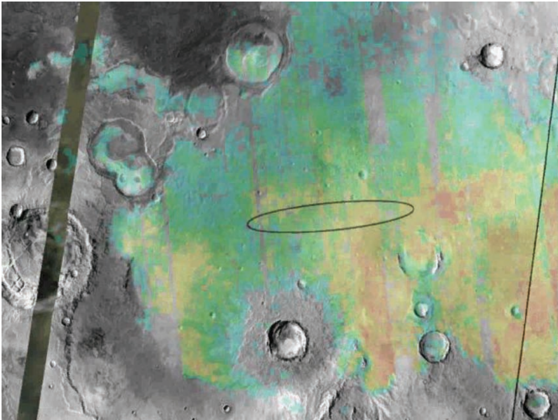
Fig. 8.21 Targeting water-containing minerals on Mars This image shows the abundances and locations of the mineral gray hematite at the landing site of the Mars Exploration Rover, Opportunity , in Meridiani Planum. It was targeted to land within the oval, which is about 71 kilometers long. A colored map from an instrument aboard the Mars Global Surveyor orbiter displays high (red and yellow) and low (green and blue) concentrations of hematite, an iron-oxide mineral that typically forms in the presence of liquid water. The underlying surface image that includes the adjacent craters is from the 2001 Mars Odyssey orbiter. The Opportunity rover found abundant evidence near its landing site for flowing water in the ancient past, about 3.7 billion years ago, including microscopic spherules dubbed “blueberries”, which are rich in hematite (see Fig. 8.24). (Courtesy of NASA/JPL/ASU.)
