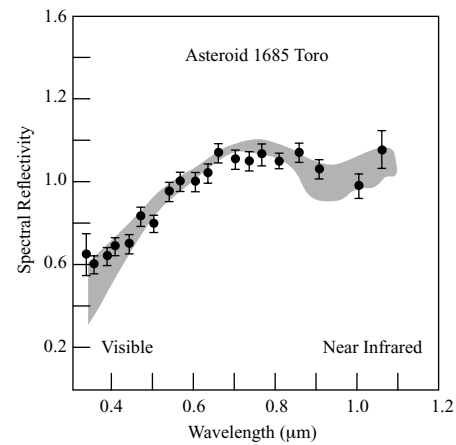
Fig. 12.7 Finding the composition of asteroids A prominent silicate absorption feature is present in the spectrum of sunlight reflected from the S-type asteroid 1685 Toro ( dark dots with error bars ). Asteroids like Toro may be the source of the stony meteorites recovered on Earth. The shaded spectrum is the reflection spectrum of a stony-chondrite meteorite. The wavelength is in units of micrometers ( \mu\text{m} ), or 10^{-6} meters.
