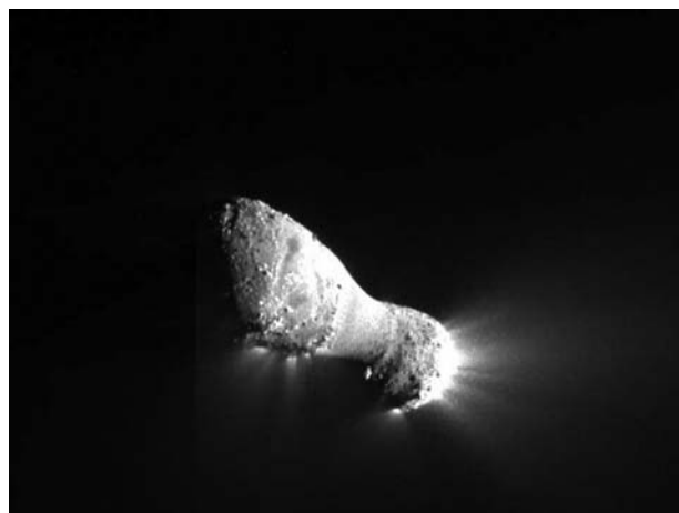
Fig. 14.19 The nucleus of comet Hartley 2 Jets stream out of the sunlit side ( right ) of the nucleus of the small, active comet Hartley 2, whose long axis spans about 2 kilometers. A narrower, smooth waist joins rough areas at both ends of the elongated nucleus. (Courtesy of NASA/JPL-Caltech/UMD.)
