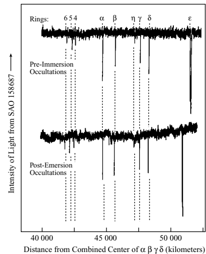
Fig. 11.7 Discovery of the thin rings of Uranus Astronomers recording the light of a star that was expected to disappear behind Uranus, on 10 March 1977, unexpectedly recorded short dips in the starlight before the star passed behind the planet ( top ). The same pattern was repeated when the star reappeared ( bottom ), indicating that narrow rings briefly block out the starlight at the same distance on opposite sides of the planet. The strong and abrupt absorption of starlight indicates that the narrow rings are quite opaque and have well-defined edges. These observations were taken from high above the Indian Ocean aboard the Kuiper Airborne Observatory. (Courtesy of James L. Elliot.)
