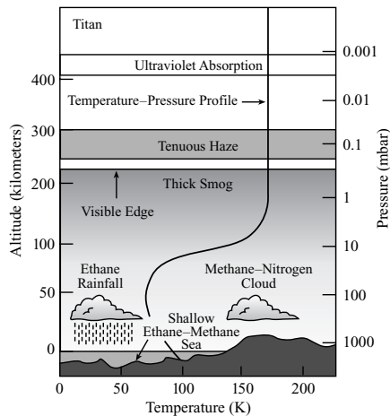
Fig. 10.25 Model of Titan's atmosphere A study of the bending and fading of homebound radio signals when the Voyager 1 spacecraft passed behind Titan led to this plot of the temperature and pressure in the satellite's atmosphere. The temperature ( bottom axis ) decreases with height until about 40 kilometers altitude, and then increases rapidly at higher altitudes ( left axis ). The entire atmosphere is well below the freezing temperature of water, at 273 kelvin, but the lower atmosphere is just warm enough to allow the condensation of liquid nitrogen. The high-altitude smog on Titan covers clouds of methane, and liquid ethane and methane probably rain down to the surface. The pressure ( right axis ) is given in units of millibars or 0.001 bars, and it reaches 1500 millibars or 1.5 bar near the surface of Titan. The air pressure at sea level on Earth is 1.0 bar. The pressure axis is logarithmic, which means that the numbers on the altitude axis are not uniformly spaced.
