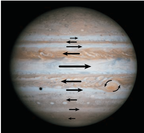
Fig. 3.6 Jupiter's counter-flowing winds The rapid rotation of Jupiter has pulled its winds into bands that flow east to west and west to east, shown in this image taken from the Cassini spacecraft on 7 December 2001. The windswept clouds move in alternating light-colored, high-pressure zones and dark-colored, low-pressure belts. The arrows point in the direction of wind flow, and their length corresponds to the wind velocity, which can reach 180 meters per second in the equatorial regions (see Fig. 3.7). The Great Red Spot swirls in the counter-clockwise direction ( curved arrows ), like a high-pressure anticyclone in the Earth's southern hemisphere, but it has lasted for more than 300 years, much longer than terrestrial storms. Jupiter's moon Europa casts a shadow on the planet. (Courtesy of NASA/JPL)
