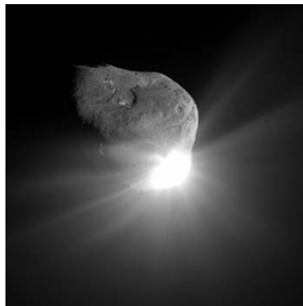
Fig. 14.18 Impact with nucleus of comet Tempel 1 The initial material ejected when the Deep Impact probe collided with the nucleus of comet Tempel 1 on 4 July 2005. The dark, cratered nucleus is an oblong body between 4.9 and 7.6 kilometers in size. Spectroscopic examination of the ejected material showed that the comet nucleus is mainly composed of water ice and dust. (Courtesy of NASA/JPL-Caltech/UMD.)
