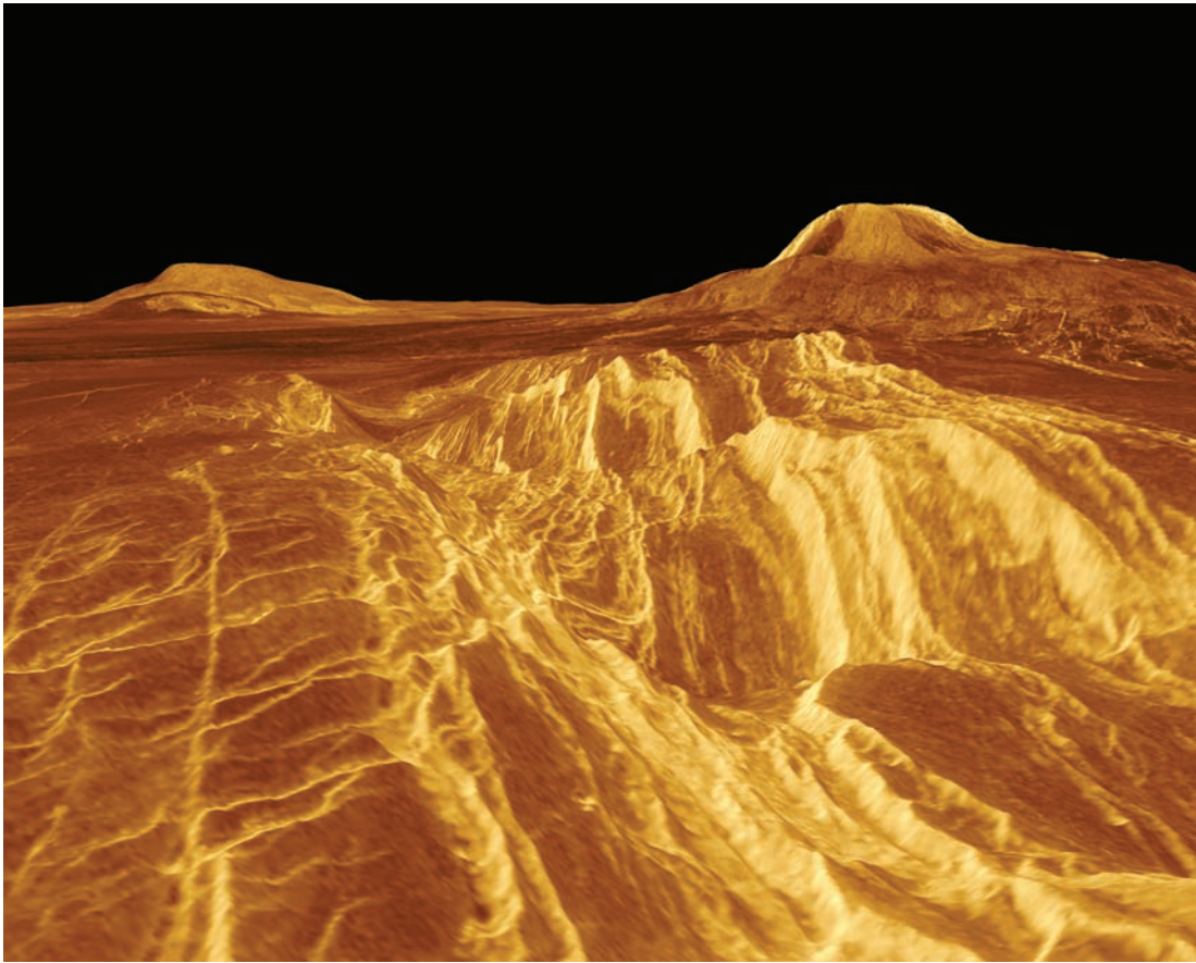
Fig. 7.15 Sif Mons and Gula Mons Two volcanoes are located at the horizon of this three-dimensional Magellan radar view of the western Eistia Regio in the central part of Venus' surface, near the equator and zero degrees east longitude. In this computer-generated image, the vertical scale has been exaggerated to show the edge of a rift valley in the foreground. It extends all the way to Gula Mons, the volcano on the right horizon, which stands 3 kilometers high and is located 700 kilometers away. The volcano on the left horizon, called Sif Mons, has a height of about 2 kilometers and a diameter of about 300 kilometers. Eistia is a Norse giantess, Gula is the name of a Babylonian earth-mother and creative force, and Sif is the name of a Teutonic goddess and Thor's wife. The artificial tints are based on color images from the Venera 13 and 14 landers, simulating the color of sunlight that filters through the thick atmosphere. (Courtesy of NASA/JPL)
