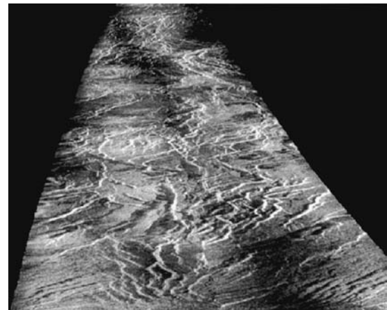
Fig. 7.13 Lava flows This Magellan image shows a lava-filled canyon produced when Venus' crust was pulled apart and magma rose within the gap. The lowland plains have many similar canyon systems; typically about 10 kilometers wide and up to 1000 kilometers long, and apparently containing solidified lava flow. This region, located near the equator between Asteria Regio and Phoebe Regio, is about 10 kilometers wide and stretches 600 kilometers to the north (top). (Courtesy of NASA/JPL)
