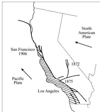
Fig. 4.13 Los Angeles is moving The Pacific Plate is moving northwestward at the rate of 0.048 meters per year, or about 5 meters every century, slowly carrying Los Angeles towards San Francisco. The North American and Pacific Plates strike and rub against each other like immense grindstones, producing earthquakes along their boundary known as the San Andreas Fault. The dated circles denote places where very major earthquakes have occurred with magnitudes of 8 and over on the Richter scale.
