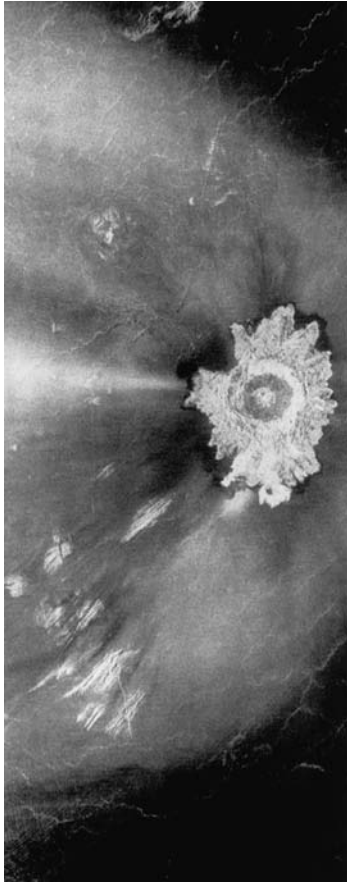
Fig. 7.5 Winds blow material ejected from a crater on Venus A radar image of Avidar Crater is surrounded by streamlined, horseshoe or parabolic shapes ( top and bottom right ) and a bright, jet-like streak ( center left ) that extends over the surrounding plains. These unusual features, seen only on Venus, are believed to result from the interaction of ejected debris and high-speed winds in the upper atmosphere, blowing from the east ( right ). The crater is 30 kilometers in diameter, and is named for the Turkish educator and author Halide Adivar (1883–1964); it is located at 9 degrees north latitude and 76 degrees east longitude, just north of the western Aphrodite highland. (Courtesy of NASA/JPL.)
