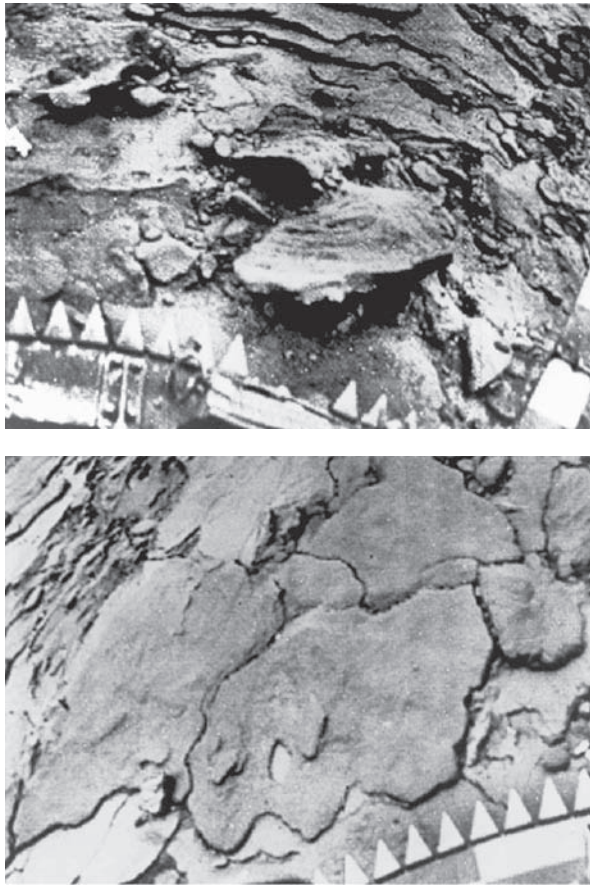
Fig. 7.3 Surface rocks on Venus On 5 March 1982 the Venera 14 lander touched down on Venus at 13 degrees south latitude and 310 degrees east longitude, where it survived for just one hour before succumbing to the planet's heat. That was long enough to radio back these photographs of the surface of Venus, which include part of the lander and a mechanical arm at the bottom. The thin, plate-like slabs of rock could be due to molten lava that cooled and cracked. The composition and texture of these rocks is similar to terrestrial basaltic lava. (Courtesy of Iosif Shklovskii.)
