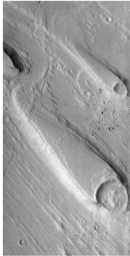
Fig. 2.41 Streamlined islands on Mars An image of the Mangala Vallis region on Mars, taken with an instrument aboard the 2001 Mars Odyssey orbiter. The scoured floors and teardrop-shaped islands were probably created by powerful, ancient flows of liquid water. The flowing water ran from the heavily cratered southern highlands to the northern lowland plains. The name Mangala is the word for Mars in Sanskrit. (Courtesy of NASA/JPL/ASU.)
