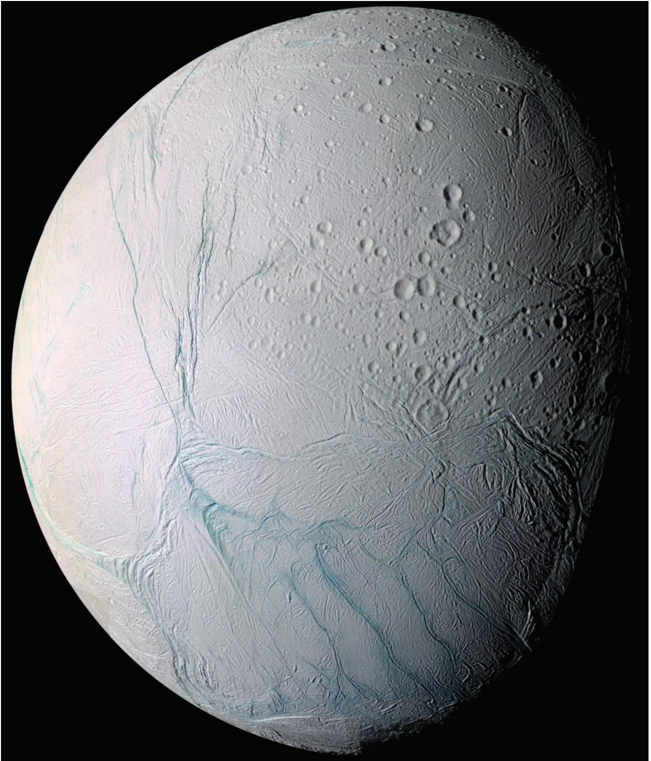
Fig. 10.21 Tiger stripes on Enceladus Saturn's enigmatic moon Enceladus is a jumbled world of fresh snow plains ( middle ), old cratered terrains ( top ), and prominent tiger-stripe fractures ( bottom, false color blue ). The fissures spray ice particles, water vapor and organic compounds outward, some of them forming Saturn's E ring and others falling back on the moon. In the mosaic shown here, three prominent tiger stripes extend from the bottom center upwards toward the center. From left to right, they are named Alexandria Sulcus, Cairo Sulcus, and Baghdad Sulcus, the longest tiger stripe. Across the middle of the image, near the northern end of the tiger stripes, 90-degree bends curve along similar paths, starting in a direction parallel to each tiger stripe and then turning perpendicular. Changes in tectonic stresses most likely cause the bends and narrow ridges. This mosaic of images was obtained in visible light from the Cassini spacecraft on 21 November 2009. (Courtesy of NASA/JPL/SSI.)
