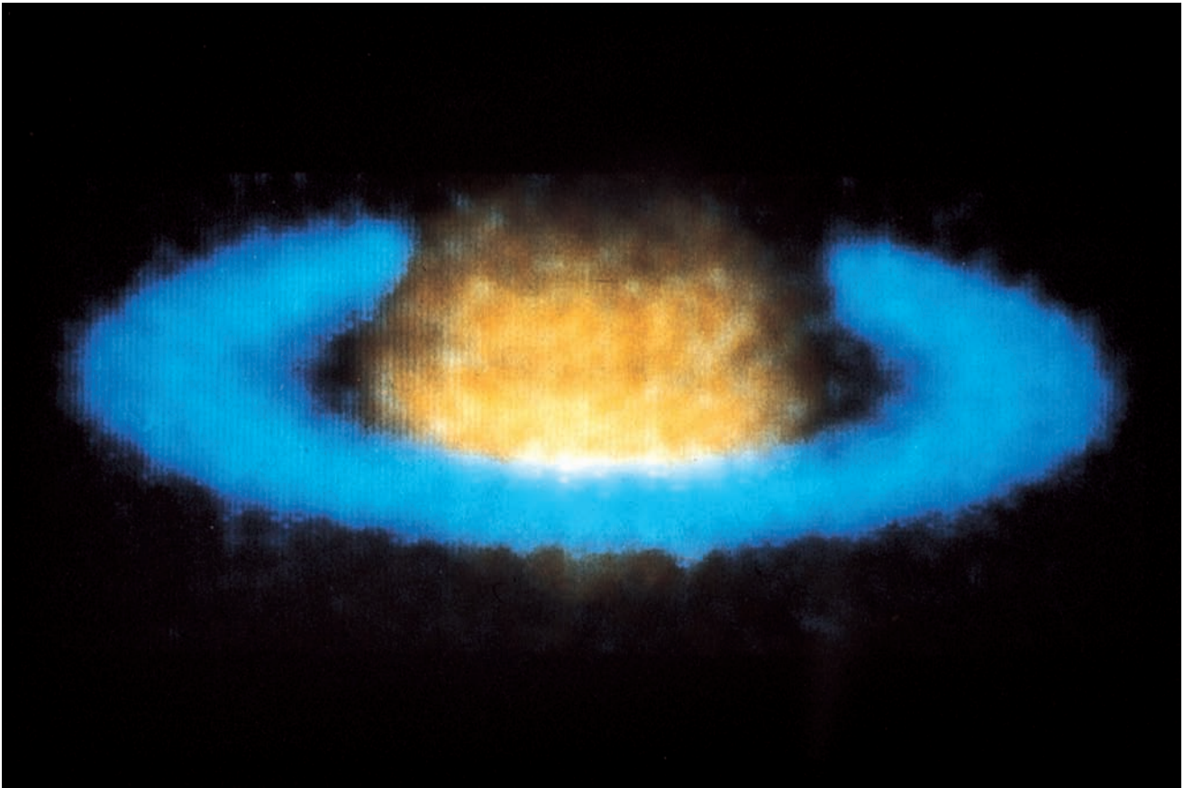
Fig. 10.7 Saturn and its rings at infrared wavelengths Because Saturn's rings are made of water-ice, they reflect relatively large amounts of sunlight at an infrared wavelength of 3.8 micrometers ( blue ). Methane in Saturn's outer atmosphere absorbs radiation at this wavelength, but the incandescent globe has its own internal source of heat that makes it shine brightly at the longer infrared wavelength of 4.8 micrometers ( orange ). The heat welling up from within Saturn is partly due to helium raining inside of the planet. (Courtesy of David Allen, Anglo-Australian Telescope Board © 1983.)
