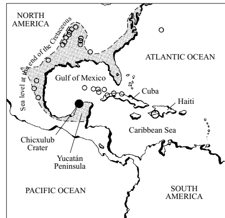
Fig. 13.11 Site of impact that wiped out the dinosaurs The long-sought site of the scar left by a killer asteroid has been found near Chicxulub (filled circle), a small village at the tip of the Yucatán Peninsula. Material from the submerged crater has been dated at about 65 million years ago, coinciding with a blast that triggered the eradication of most life on Earth. Thick sedimentary deposits laid down 65 million years ago in Haiti (big open circle) contain exceptionally large amounts of iridium, shocked quartz and glassy debris that are thought to be part of the impact across the Caribbean, almost 2000 kilometers away. The small open circles mark the sites of marine wave deposits associated with the same impact. [Adapted from Alan R. Hildebrand and William V. Boynton, Natural History 6 47–53 (1991).]
