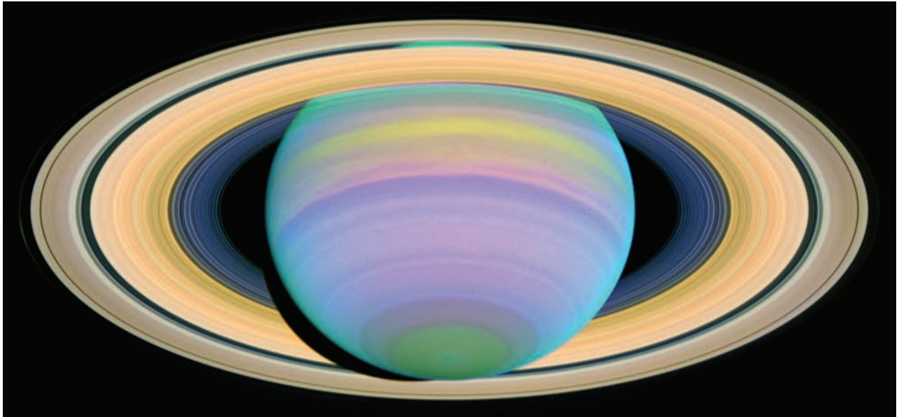
Fig. 10.3 Saturn at ultraviolet wavelengths The southern hemisphere of Saturn reaches its maximum 27-degree tilt toward Earth, revealing the planet's banded clouds as well as its rings. Particles in Saturn's atmosphere and rings reflect different wavelengths of radiation in different ways, as indicated in this ultraviolet image that reveals smaller particles that do not absorb or scatter radiation at the longer visible or infrared wavelengths. Saturn's counter-flowing east-west winds have aligned the cloud particles, believed to be ammonia ice crystals, within fixed latitude bands. The rings are made up of particles of water-ice. This view of Saturn was recorded from the Hubble Space Telescope on 7 March 2003. (Courtesy of NASA/E. Karkoschka, U. Arizona.)
