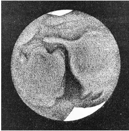
Fig. 8.3 Polar cap of Mars and its Syrtis Major The English amateur astronomer Warren De La Rue (1815–1889) made this drawing of Mars on 20 April 1856, using a 0.33-meter (13-inch) reflector telescope. It shows bright polar caps and a dark, triangular feature now known as Syrtis Major Planitia (Gulf of Sirte Plains). The Dutch astronomer Christiaan Huygens (1629–1695) first sketched this feature in 1659. From his observations of Syrtis Major, Huygens concluded that the rotation period of Mars is about 24 hours. This drawing is reproduced from Camille Flammarion’s (1842–1925) book La Planete Mars et ses Conditions d’Habitabilité , published in 1892.
