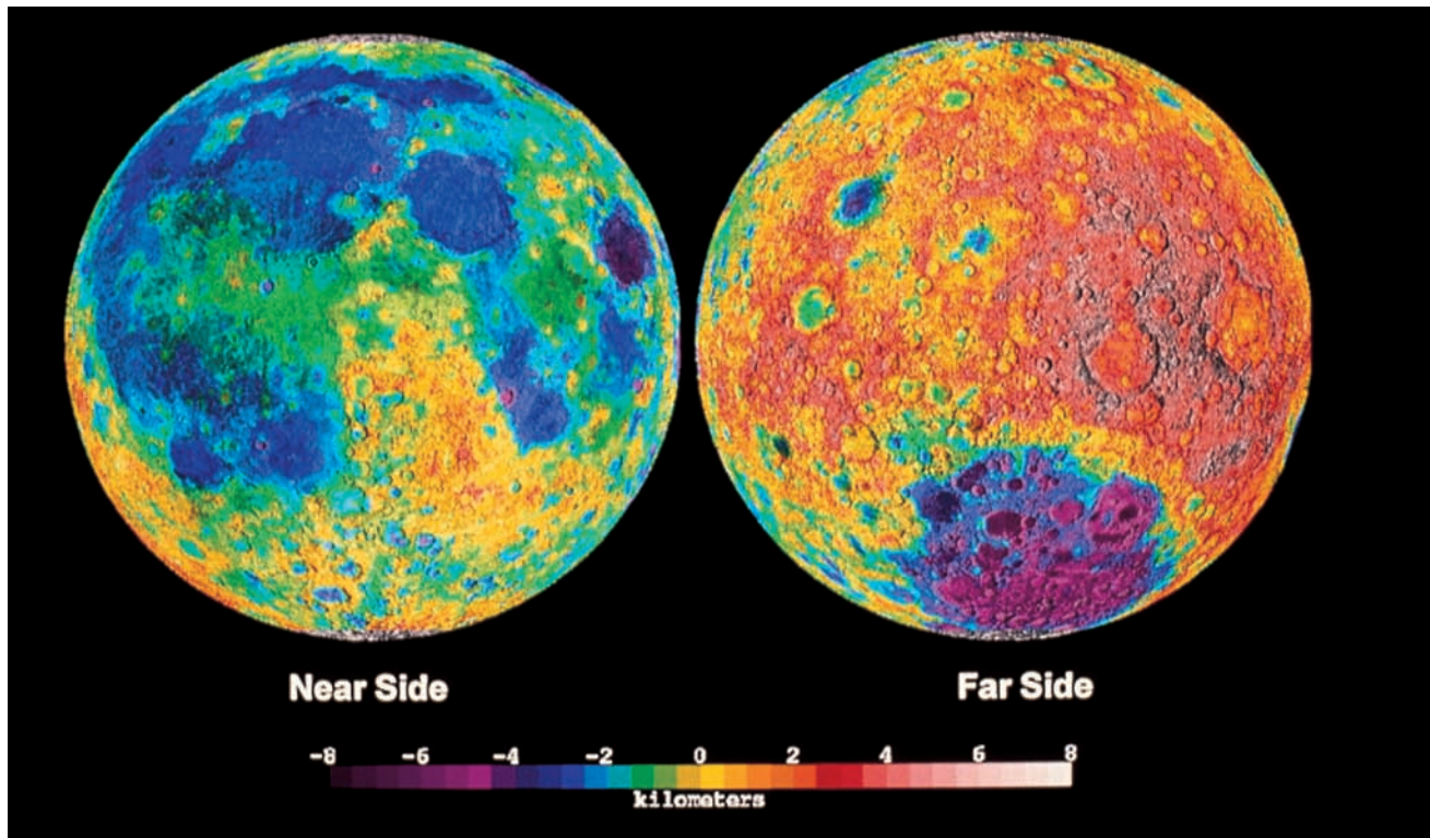
Fig. 5.25 Lunar topography The laser altimeter on Clementine provided the first comprehensive topographic map of the Moon. The contour interval is 500 meters, and the altitude in kilometers is coded by color from blue to red ( bottom ). The near side ( left ) is relatively smooth and low ( blue and purple ), primarily because of the prominent impact basins, including Imbrium, Crisium and Nectaris, which are at least partly filled with mare basalt. In contrast, the far side ( right ) shows high relief ( red ) and extreme topographic variation comparable to that of the Earth. The Moon's wide altitude range is attributed to ancient impact basins that have been preserved for about 3.9 billion years, while the Earth's wide range stems from ongoing mountain building by colliding tectonic plates. The large circular feature on the southern far side ( right bottom ) is the South Pole – Aitken basin, 2600 kilometers in diameter and 12 kilometers deep. (Courtesy of Paul D. Spudis, Lunar and Planetary Institute.)
