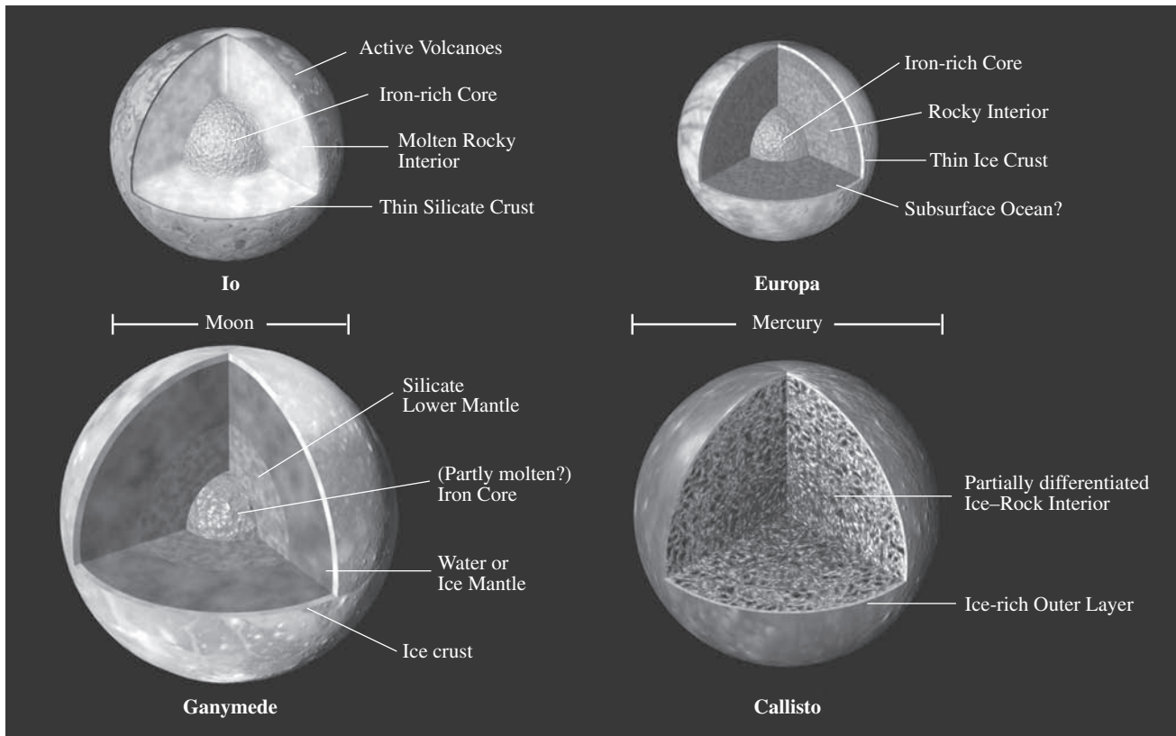
Fig. 9.10 Inside the Galilean satellites Cutaway views of the possible internal structures of the Galilean satellites. Ganymede is at the lower left, Callisto at the lower right, Io on the upper left, and Europa on the upper right. The surfaces of the satellites are mosaics of images obtained in 1979 by the Voyager 1 or 2 spacecraft, and the interior characteristics are inferred from gravity field and magnetic field measurements from the Galileo spacecraft. With the exception of Callisto, all the satellites have iron-nickel cores surrounded by rock shells. Io's rock or silicate shell extends to the surface, while the rock layers of Ganymede and Europa are surrounded by shells of water ice or liquid water. Callisto seems to be a relatively uniform mixture of comparable amounts of ice and rock. Galileo images of Europa suggest that a liquid water ocean might now underlie a surface layer of water ice. (Courtesy of NASA/JPL.)
