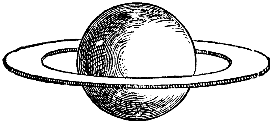
Fig. 1.18 Saturn's ring In 1659 Christiaan Huygens (1629–1695) published this drawing of Saturn and its ring in his monograph Systemia Saturnium . Huygens recognized that a detached ring would explain the planet's ever-changing appearance, and announced his discovery in the form of an anagram, a succession of scrambled letters. The drawing shown here was accompanied by the deciphered anagram “Saturn is girdled by a thin flat ring, nowhere touching it, and inclined to the ecliptic.”
