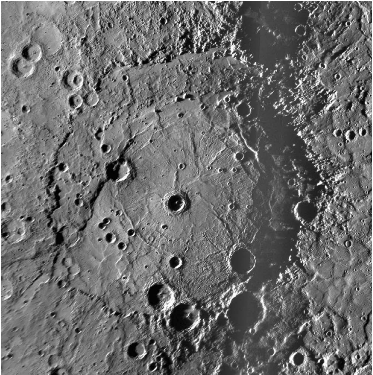
Fig. 6.14 Rembrandt impact basin This well-preserved impact basin was discovered in images taken from the MESSENGER spacecraft. Named Rembrandt, after the Dutch painter, it is about 715 kilometers in diameter. Scientists estimate that it was formed about 3.9 billion years ago, near the end of the period of heavy bombardment of the inner solar system. Although ancient, the distributions of smaller craters on its surface indicate that Rembrandt is younger than many other impact basins on Mercury. The basin and some of the small craters have also been flooded by effusive volcanic flows with a smooth appearance. Multi-colored images of the crater floor indicate areas with unusually high amounts of iron and titanium. (Courtesy of NASA/JHUAPL/SSI/CIW.)
