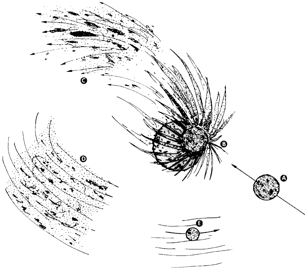
Fig. 5.33 Giant impact hypothesis for the origin of the Earth's Moon According to the giant impact hypothesis, a massive projectile (A), about the size of Mars, struck the young, still-forming Earth (B) in a catastrophic, glancing blow nearly 4.6 billion years ago, resulting in a tremendous explosion and the jetting outward of both projectile and Earth mass. Some fraction of this mass remained in Earth orbit (C), while the rest escaped Earth or impacted again on Earth's surface. A proto-Moon began to form from the orbiting material (D), accreting neighboring matter, and finally became the Moon (E). It may be mostly derived from the crust and mantle of the Earth and/or the impacting object, accounting for the Moon's relatively low mean mass density and lack of iron when compared with the Earth. The Moon accumulated so rapidly that the outer crust was molten, helping to account for the relative lack of water and other volatile elements. Then, as the crust cooled, the newborn Moon swept up the remaining objects nearby, blasting out impact basins and pockmarking the surface with numerous craters. (Courtesy of Alan P. Boss, Carnegie Institution of Washington.)
