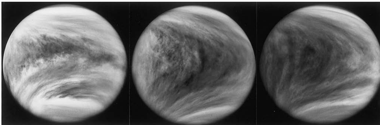
Fig. 3.4 Raging winds on Venus A high-velocity wind whips the upper layer of Venus's cloud deck around the planet's equator once every four Earth days, moving at speeds of up to 100 meters per second. These photographs taken at ultraviolet wavelengths on consecutive days by the Pioneer Venus spacecraft in 1979 illustrate this. The Y-shaped clouds move towards the west (left). A zonal east-to-west circulation dominates the winds of Venus. The low atmosphere and the planet's surface also rotate westward, but with the much slower period of 243 Earth days. (Courtesy of NASA/Larry Travis.)
