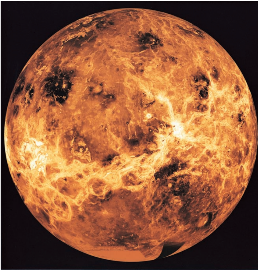
Fig. 2.9 Venus unveiled with radar A cloud-penetrating radar system on board the Magellan spacecraft has mapped the global landforms and features on Venus with a resolution of 120 meters, more completely than any planet including Earth. This hemisphere, centered at 180 degrees east longitude, shows the bright, planet-wide, equatorial highlands that contain towering volcanoes, long lava flows and deep faults and fractures. They run from lower left to upper right through Aphrodite Terra ( left of center ), a continent-sized highland, and the bright highland Atla Regio ( just right of center ) to Beta Regio ( far right and north ). Dark areas correspond to terrain that is smooth on the scale of the radar wavelength (0.13 meters); bright areas are rough. The orange tint, based on color images taken by the Venera 13 and 14 landers, simulates the color of sunlight at ground level after being filtered through the planet's thick atmosphere and clouds. (Courtesy of NASA/JPL.)
