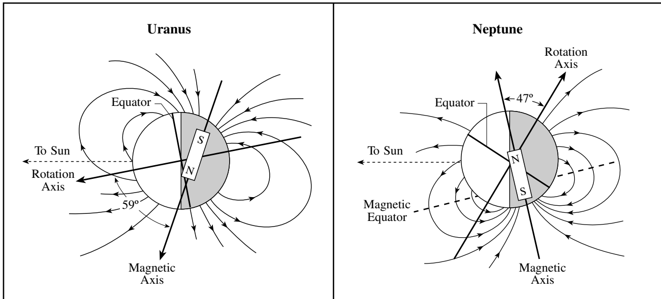
Fig. 3.19 Tilted magnetic fields The magnetic fields of Uranus and Neptune can be represented by a simple bar magnet, or dipole, embedded in the planet, but with a magnetic axis that is tilted with respect to the rotation axis. For Uranus the tilt is about 59 degrees; Neptune has a tilt of 47 degrees. In contrast, the magnetic axes of Jupiter, Saturn and Earth are much more nearly aligned with their rotation axes. The arrow of the rotation axis points from the geographic south towards geographic north, and the magnetic axis similarly points from magnetic south to magnetic north. On Uranus and Neptune a terrestrial compass would point toward the southern hemisphere of the planet, while on Earth it points toward the geographic north pole. In addition to the dipole part of their magnetic field, Uranus and Neptune have a large additional component known as the quadrupole. A method of visualizing this is to imagine that the dipole has a magnetic center that is offset from the center of the planet. As shown here, the equivalent offset for Uranus is almost a third of the planet's radius, and there is a larger offset for Neptune of nearly half its radius. But such off-center dipoles are only useful as a picture of what the external field looks like and do not help in understanding how it is produced deep down.
