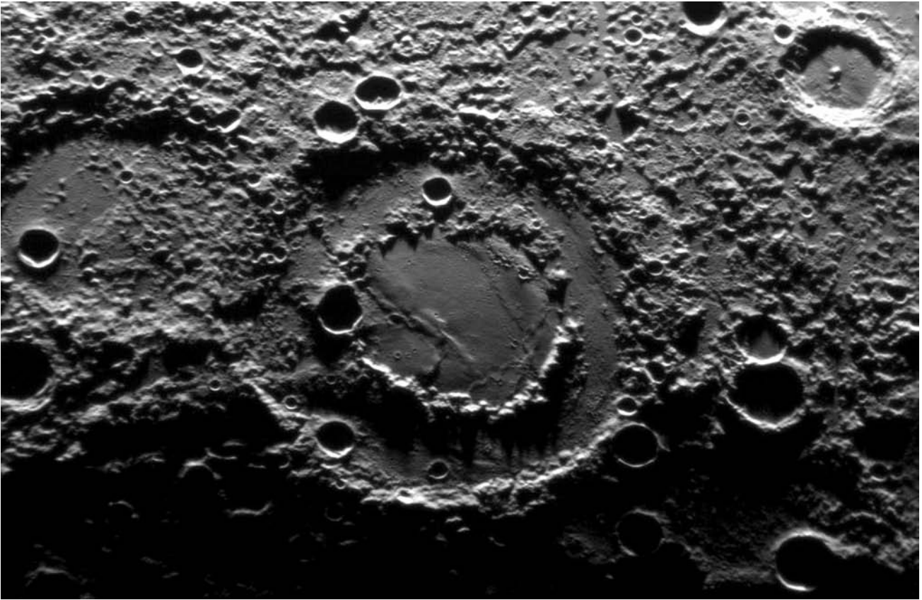
Fig. 2.29 Volcanic activity on Mercury This double-ringed impact basin on Mercury has a smooth inner floor attributed to lava flows that partially flooded the basin some time after impact. The basin is approximately 60 kilometers in diameter. This image was acquired from the MESSENGER spacecraft on 29 September 2009. (Courtesy of NASA/JHUAPL/CIW.)
