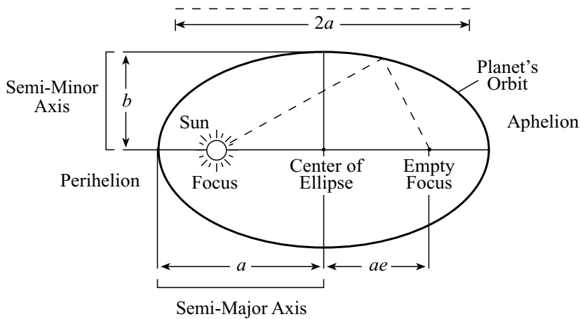
Fig. 1.11 Elliptical orbit Each planet moves in an ellipse with the Sun at one focus. The length of a line drawn from the Sun, to a planet and then to the empty focus, denoted by the dashed line, is always 2a , or twice the semi-major axis, a . The eccentricity, or elongation, of the planetary ellipse has been greatly overdone in this figure; planetary orbits look much more like a circle.
