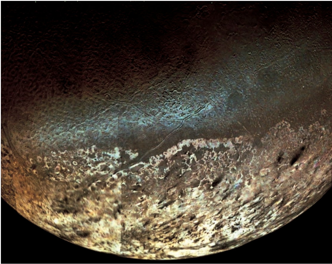
Fig. 11.14 Triton, the largest moon of Neptune A mosaic of the south polar cap of Triton, the largest satellite of Neptune, taken in August 1989 from the Voyager 2 spacecraft. At the time of this flyby, Triton was the coldest measured object in the solar system with a surface temperature of 37.5 kelvin. It is so cold that most of Triton's thin nitrogen atmosphere is condensed as frost, making it the only satellite in the solar system known to have a surface coated with deposits of solid nitrogen ice. Small admixtures of highly reflective methane ice are also present on the surface; they have been reddened and darkened by the action of energetic radiation. Dark plumes and streaks probably mark vents of ice volcanoes, where nitrogen gas has been driven outward in geyser-like eruptions from beneath the surface and carried by the winds into elongated streaks. (Courtesy of NASA/JPL)
