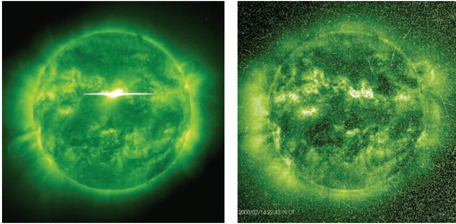
Fig. 4.28 Solar flare produces threatening space storm of energetic particles A powerful solar flare ( left ), occurring at 10 hours 24 minutes Universal Time on Bastille day, 14 July 2000, unleashed high-energy protons that began striking the SOHO spacecraft near Earth about 8 minutes later, continuing for many hours ( right ). Both images were taken from the Extreme-ultraviolet Imaging Telescope (EIT) on the SOLar and Heliospheric Observatory (SOHO) . (Courtesy of the SOHO EIT consortium. SOHO is a project of international cooperation between ESA and NASA.)
