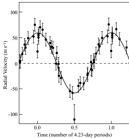
Fig. 16.8 Unseen planet orbits the star 51 Pegasi Discovery data for the first planet found orbiting a normal star other than the Sun. The giant, unseen planet is revolving around the solar-type star 51 Pegasi, located 50.9 light-years away. The radial velocity of the star, in units of meters per second, has been measured from the Doppler shift of the star's spectral lines. The velocity exhibits a sinusoidal variation with a 4.23-day period, caused by the invisible planetary companion that orbits 51 Pegasi with this period. The observational data ( solid dots ) are fit with the solid line, whose amplitude implies that the mass of the companion is roughly 0.46 times the mass of Jupiter. The 4.23-day period indicates that the unseen planet is orbiting 51 Pegasi at a distance of 0.05 AU, where 1.00 AU is the mean distance between the Earth and the Sun. [Adapted from Michael Mayor and Didier Queloz, "A Jupiter-mass companion to a solar-type star", Nature 378 , 355–359 (1995).]
