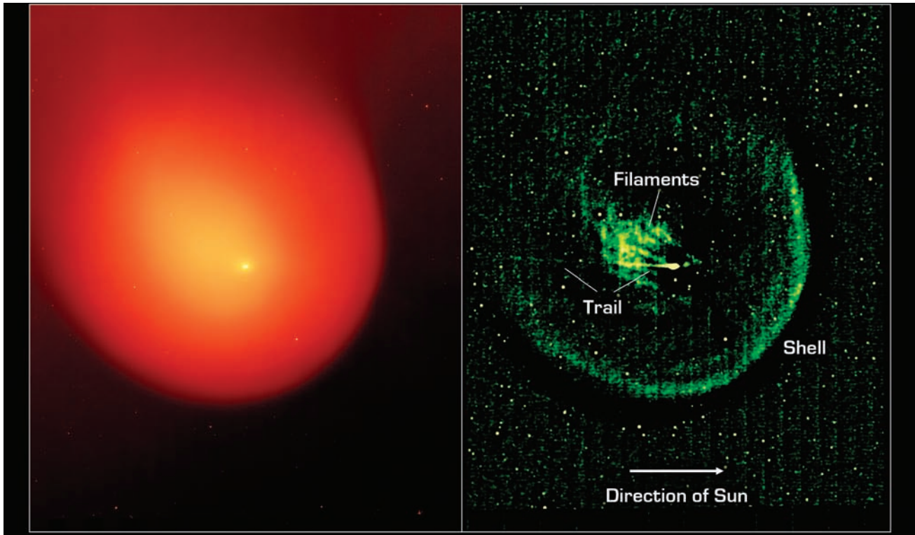
Fig. 14.23 Comet explosion Comet Holmes has exploded just twice in 118 years, in November 1892 and October 2007, while approaching the asteroid belt and moving from the vicinity of Jupiter toward the Sun. This infrared image was obtained from the Spitzer Space Telescope in March 2008; five months after the comet suddenly erupted and brightened a million-fold overnight. The infrared picture ( left ) reveals dust particles that make up the outer shell, which envelops solid particles ( yellow ) blown from the exploding comet and the comet nucleus ( white center ). The contrast-enhanced image ( right ) shows the outer shell and filaments or streamers of dust. (Courtesy of NSA/JPL-Caltech.)
