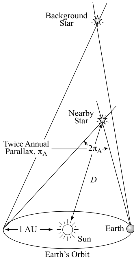
Fig. 1.20 Annual parallax When a distant and nearby star are observed at six-month intervals, on opposite sides of the Earth's orbit around the Sun, astronomers measure the angular displacement between the two stars. It is twice the annual parallax, designated by \pi_A , which can be used to determine the distance D of the nearby star. The German astronomer Friedrich Wilhelm Bessel (1784–1846) announced the first reliable measurement of the annual parallax of a star in 1838.
