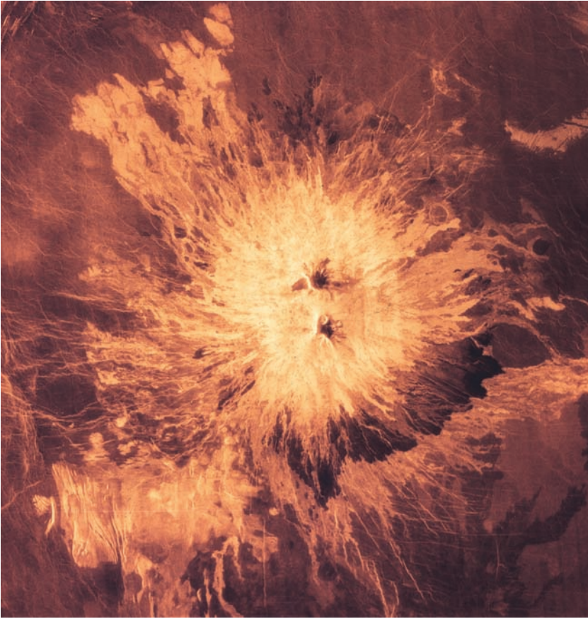
Fig. 7.16 Sapas Mons Located in an equatorial highland called Atla Regio, the volcano Sapas Mons is about 400 kilometers in diameter and 1.5 kilometers high; it is named after a Phoenician goddess. The sides of the volcano are composed of numerous overlapping lava flows from flank eruptions similar to terrestrial volcanoes such as the Hawaiian shield volcanoes. The summit contains two smooth, radar-dark mesas, as well as groups of pits, some as large as 1 kilometer across. They may have formed when underground chambers of magma were drained, causing the surface to collapse above them. A 20-kilometer-diameter impact crater northeast ( upper right ) of the volcano is partly buried in lava flows. (Courtesy of NASA/JPL.)
