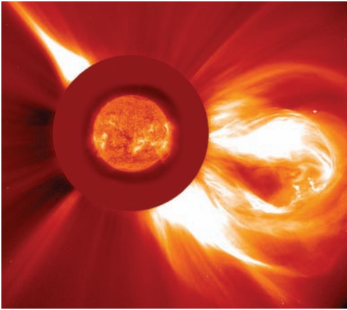
Fig. 4.26 Mass ejection from the Sun A huge coronal mass ejection is seen in this coronagraph image, taken on 5 December 2003 with the Large Angle Spectrometric Coronagraph (LASCO) on the Solar and Heliospheric Observatory (SOHO). The solid red circle corresponds to the occulting disk of the coronagraph that blocks intense sunlight and permits the corona to be seen. An image of the singly ionized helium, denoted He II, emission of the Sun, taken at about the same time, has been appropriately scaled and superimposed at the center of the LASCO image. The full disk helium image was taken at a wavelength of 30.4 nanometers, corresponding to a temperature of about 60 000 kelvin, using the Extreme-ultraviolet Imaging Telescope, or EIT for short, aboard SOHO. (Courtesy of the SOHO LASCO and EIT consortia. SOHO is a project of international cooperation between ESA and NASA.)
