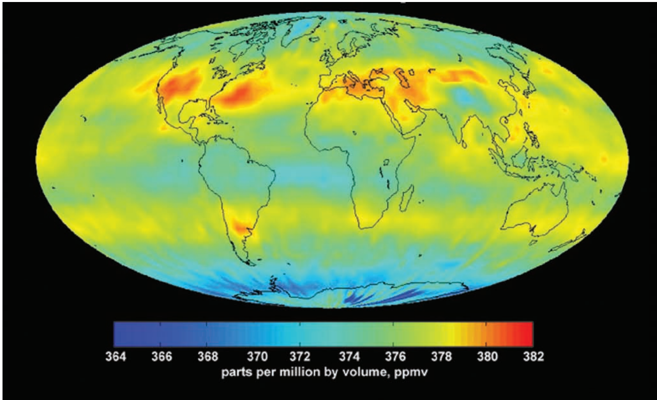
Fig. 4.23 Carbon dioxide in the Earth's troposphere The concentration of carbon dioxide about 8 kilometers above the Earth's surface in July 2003. The regional distribution can still be seen by the time that the gases reach this height in the mid-troposphere, with large concentrations above parts of the United States and China. This image was acquired from the Atmospheric Infrared Sounder Experiment aboard the Aqua spacecraft. (Courtesy of NASA/JPL.)
