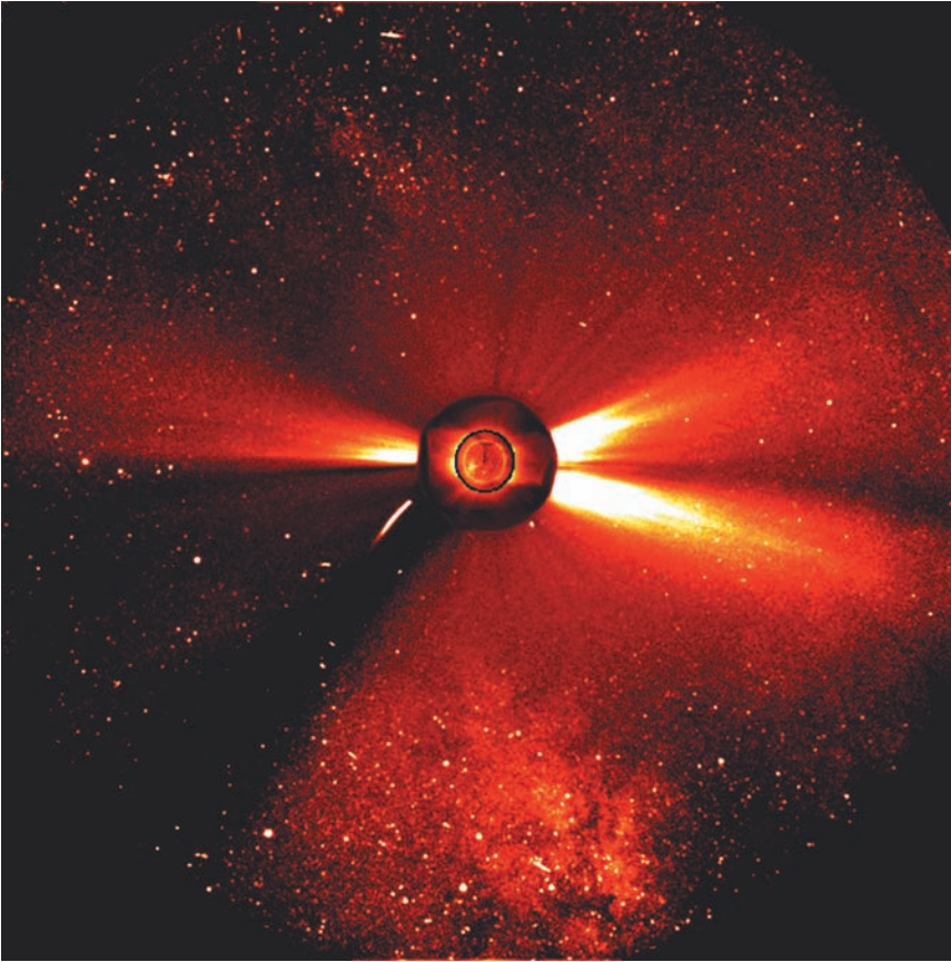
Fig. 13.4 Fatal impact of a comet into the Sun This composite image records a comet plunging into the Sun on 23 December 1996. The innermost image ( center ) records the bottom of the million-degree solar atmosphere, known as the corona. The electrically charged coronal gas is seen blowing away from the Sun just outside the inner dark circle, which marks the edge of one instrumental occulting disk. Another instrument records the comet ( lower left ), as well as the coronal streamers at more distant regions and the stars of the Milky Way. (Courtesy of the SOHO EIT, UVCS and LASCO consortia. SOHO is a project of international collaboration between ESA and NASA.)
