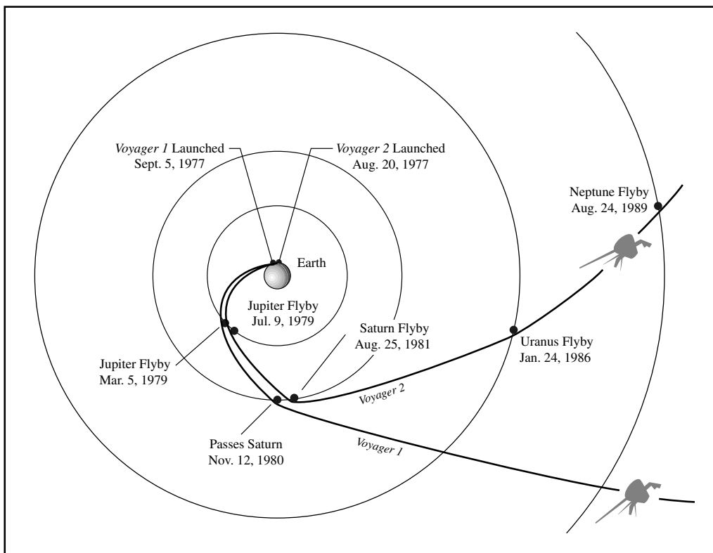
Fig. 2.3 Grand tour of Voyager 1 and 2 The flights of the two Voyager spacecraft through the solar system. Both spacecraft were launched in 1977 and flew past Jupiter in 1979, transmitting remarkable details of the giant planet's weather and the surfaces of its four largest satellites. Voyager 1 and 2 used the gravity of Jupiter to accelerate them on toward Saturn, providing close-up images of its rings and satellites in 1980–81. Saturn provided another gravity assist to propel Voyager 2 on to Uranus, in 1986, and then on to Neptune in 1989. Voyager 1 was targeted differently at Saturn, sacrificing its grand tour for close views of the satellite Titan. Both spacecraft have now crossed the termination shock of the solar wind, marking its outer boundary.
