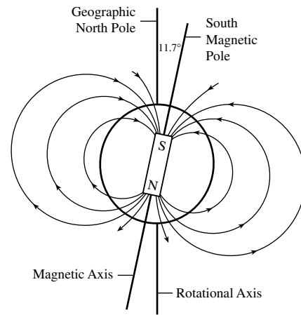
Fig. 3.12 Earth's magnetic dipole The Earth's magnetic field looks like that which would be produced by a bar magnet at the center of the Earth, with the north magnetic pole corresponding to the south geographic pole and vice versa. The Earth's magnetic dipole originates in swirling currents of molten iron deep in the Earth's liquid outer core, and extends more than 10 Earth radii, or 63.7 thousand kilometers, out into space on the side facing the Sun, and all the way to the Moon's orbit at 384 000 kilometers on the opposite side. Magnetic field lines loop out of the north magnetic pole and into the south magnetic pole. The lines are close together near the magnetic poles where the magnetic force is strong, and spread out where it is relatively weak. The magnetic axis is tilted at an angle of 11.7 degrees with respect to the Earth's rotational axis. This dipolar (two poles) configuration applies near the surface of the Earth, but further out the magnetic field is distorted by the solar wind.
