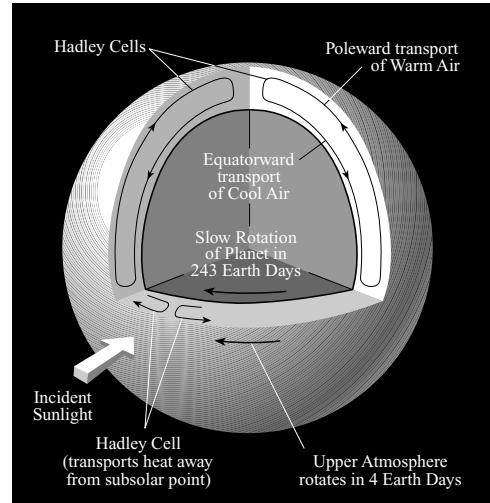
Fig. 7.6 Hadley cells in the atmosphere of Venus Incident solar energy drives a Hadley-cell circulation of the atmosphere, which keeps heat from building up at any one location. Air rises in warm regions near the equator on the sunlit side of Venus, where the planet is heated most by the Sun. Some of the warm air flows towards cooler zones near the poles, and sinks and returns to warm equatorial regions again. Strong winds also blow around the planet in the direction that Venus rotates, from east to west.
