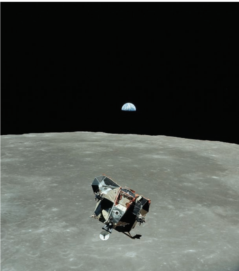
Fig. 5.16 Going home from the Moon
