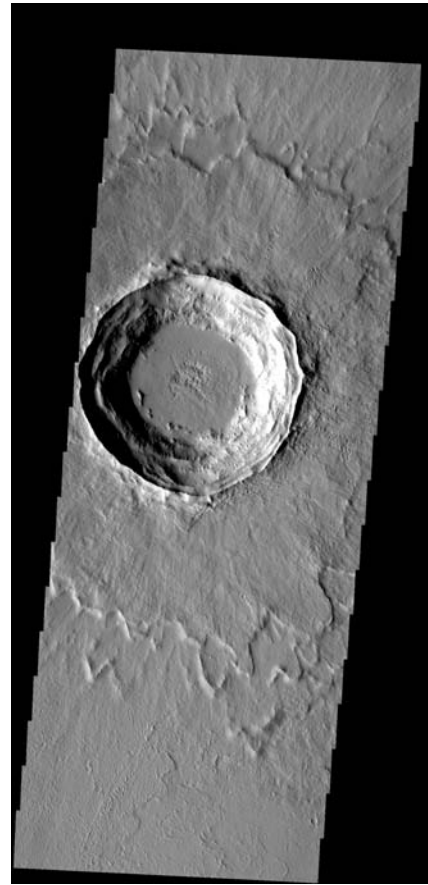
Fig. 2.24 Material ejected from impacts on Mars Some Martian craters are surrounded by discrete lobes of fresh-appearing flows, each surrounded by a low ridge or rampart and sometimes layered. The unique pattern of ejected material can be attributed to melting of water ice by the heat of impact. An instrument aboard the 2001 Mars Odyssey orbiter took this image. (Courtesy NASA/JPL/ASU.)
