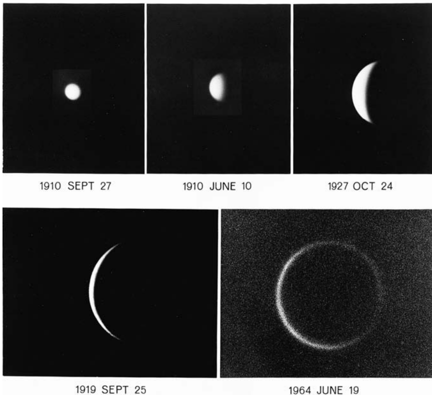
Fig. 7.1 The phases of Venus When fully illuminated, Venus looks small and far away; its apparent size is about seven times larger when the crescents are narrowest and Venus is nearest the Earth. After observing similar phases with his small telescope in 1610, Galileo wrote “ Cynthiae figuras aemulatur mater amorum ”, or “The mother of love (Venus) emulates the figure of Cynthia (Moon)”. The phases and variation in the apparent size of Venus provided important early evidence that the planets revolve around the Sun rather than the Earth. (Lowell Observatory photographs.)
