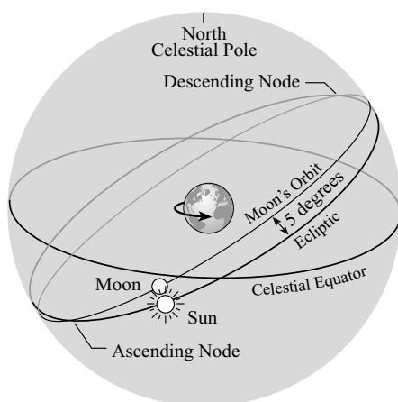
Fig 5.4 Celestial paths of the Moon and Sun The orbit of the Earth's Moon is tilted 5 degrees to the Sun's route across the sky, the ecliptic, allowing these paths to cross at two nodes. These are the only points at which eclipses can occur. During a lunar eclipse the Moon and Sun are located at opposing nodes, so that the Moon can move into the Earth's shadow cast by the Sun. A solar eclipse occurs when the Moon and Sun cross paths at the same node.
