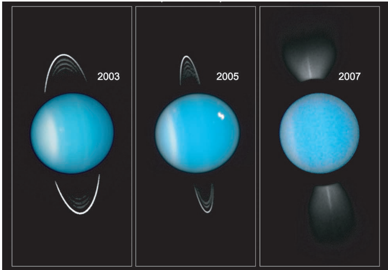
Fig. 11.10 Rings on edge These images were taken from the Hubble Space Telescope over a four-year period, from 2003 to 2007 (left to right), as Uranus moved along one-twentieth of its 84-year journey around the Sun. As viewed from the Earth, the rings are always nearly perpendicular to the planet's orbital plane, but they gradually close up from partly open to edge on. When tiled edge-on to Earth, on 14 August 2007, the rings appeared as spikes above and below the planet, within a fan-shaped glare – an image artifact. The fainter outer rings appear in the 2003 image, but were not noticed until they were seen in the 2005 image. Uranus has a total of 13 dusty rings. (Courtesy of NASA/ESA/M. Showalter, SETI Institute.)
