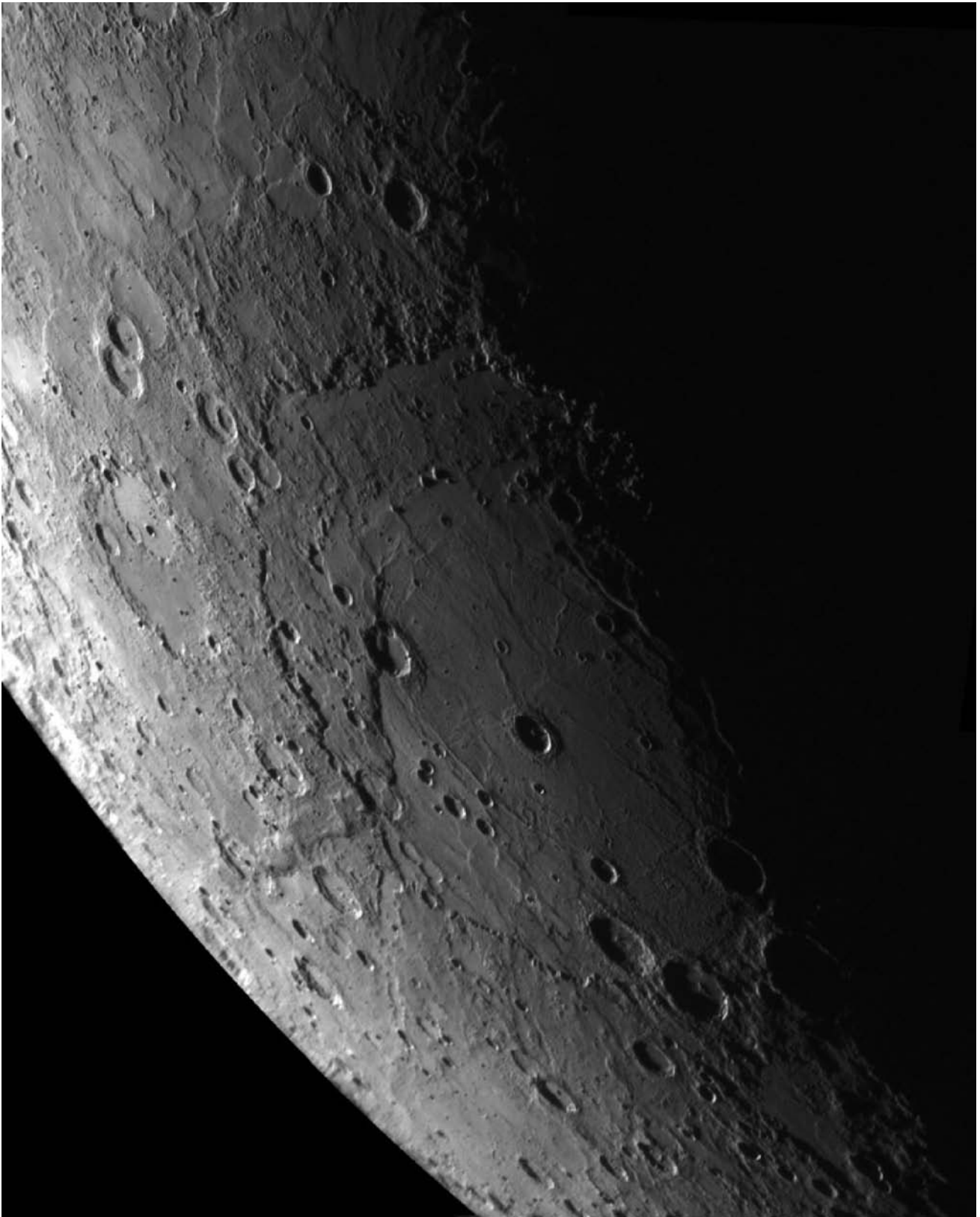
Fig. 6.8 Previously unseen side of Mercury A mosaic of images collected as the MESSENGER spacecraft viewed Mercury obliquely on its second approach on 6 October 2008. The Rembrandt impact basin, 715 kilometers in diameter and also shown in Fig. 6.14, is seen at the center as night was falling across the planet's eastern (right) edge. (Courtesy of NASA/JHUAPL/CIW.)
