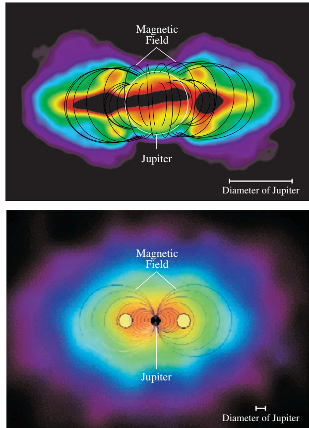
Fig. 3.17 Jupiter's magnetosphere High-speed electrons that are trapped in Jupiter's magnetosphere emit steady radio radiation (top) by the synchrotron process; it is detected by ground-based radio telescopes such as the Very Large Array. An instrument aboard the Cassini spacecraft measured energetic atoms (bottom) created when fast-moving ions within the magnetosphere picked up electrons to become neutral atoms. The two open circles denote Io's orbital position on each side of the planet; the central black disk denotes Jupiter. [Courtesy of Imke de Pater, U. C. Berkeley (top) and NASA/JPL/JHUAPL (bottom).]
