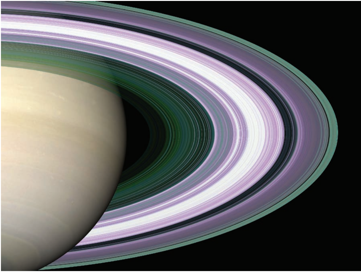
Fig. 10.11 Particles in Saturn's rings When the Cassini spacecraft passed behind the rings of Saturn, it sent three simultaneous radio signals, at 0.94, 3.6 and 13 centimeter wavelength, through the rings to Earth. The observed changes of each signal as the spacecraft moved behind the rings provided a profile of the distribution of ring material as a function of distance from Saturn, or an optical-depth profile. The image shown here was constructed from these profiles, depicting the observed ring structure at about 10 kilometers in resolution. Color is used to present information about the presence or absence of small ring particles in different regions based on the measured effects of the three radio signals. Purple color indicates regions where there is a lack of particles of size less than 5 centimeters. Green and blue shades indicate regions where there are particles smaller than 5 centimeters and 1 centimeter, respectively. The saturated broad white band is the densest region of the B ring, which blocked two of the three radio signals. From other evidence in the radio observations, all ring regions appear to be populated by a broad range of particle sizes that extend to several meters across. (Courtesy of NASA/JPL)
