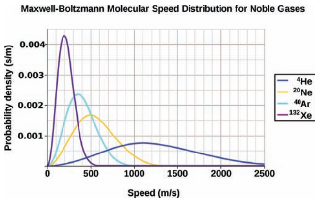
Fig. 3.1 Maxwell-Boltzmann speed distribution The probability distribution of speed density ( vertical axis ) at different speeds, v ( horizontal axis ) for a temperature of T = 218.85 kelvin and four noble gases, helium ( blue ), neon ( yellow ), argon ( turquoise ) and xenon ( purple ). The peak of each curve occurs at the most probable speed, v_p = (2kT/m)^{1/2} , where Boltzmann's constant is k = 1.38 \times 10^{-23} joule per kelvin, T is the temperature, and m is the element's mass. This distribution was first derived by the Scottish scientist James Clerk Maxwell (1831–1879) in 1866. As indicated in this plot, the peak shifts to higher speeds at lower mass provided the temperature is unchanged, because less massive elements tend to move at faster speeds. A similar change occurs at higher temperatures for a given mass. Ninety-nine percent of all molecules have speeds greater than the average molecular speed, given by v_{\text{avg}} = (3kT/m)^{1/2} , for every curve has a high-velocity tail which is most evident in the purple line. The equation for the distribution f(v) is: f(v) = 4\pi [m/(2\pi kT)]^{3/2} v^2 \exp[-mv^2/(2kT)] .
