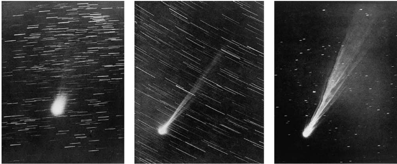
Fig. 14.10 Three kinds of comet shapes Comet Perrine (1902 III) shows a transparent coma and tail ( left ), comet Finsler (1937 V) exhibits a coma and tail that are asymmetrical ( center ), and comet Morehouse (1908 III) is remarkable for the rapid variations in the structure of its tail ( right ). When a telescope follows a comet, stars move across the field of view, producing numerous short star trails. [Courtesy of the Royal Observatory Greenwich ( left and right ) and the Norman Lockyer Observatory ( center ).]
