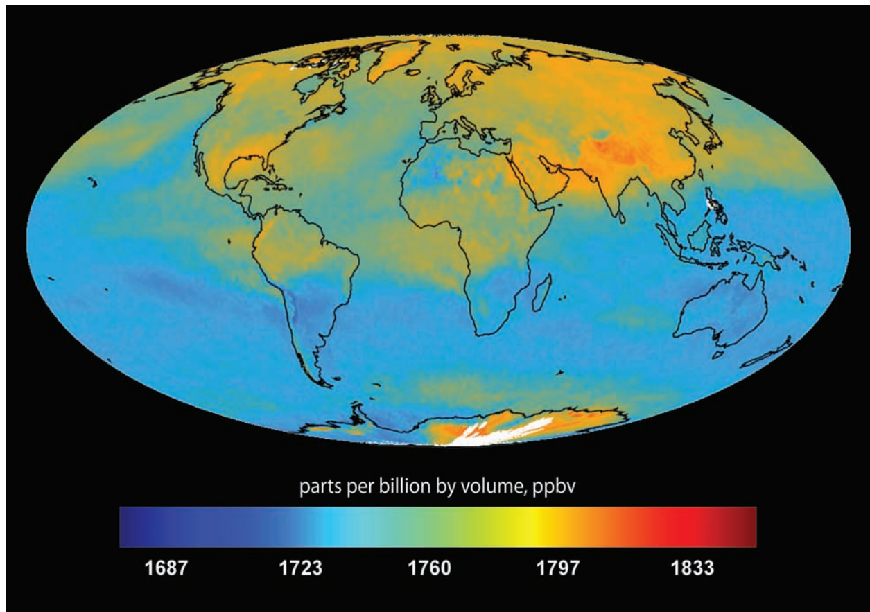
Fig. 4.24 Methane in the Earth's troposphere The global distribution of methane in the lower parts of the Earth's atmosphere, known as the troposphere. This image was taken from the Atmospheric Infrared Sounder Experiment aboard the Aqua spacecraft in August 2005. Such images will help identify sources of this heat-trapping greenhouse gas, as well as its seasonal and multi-year variation and its transport around the globe. (Courtesy of NASA/JPL.)
