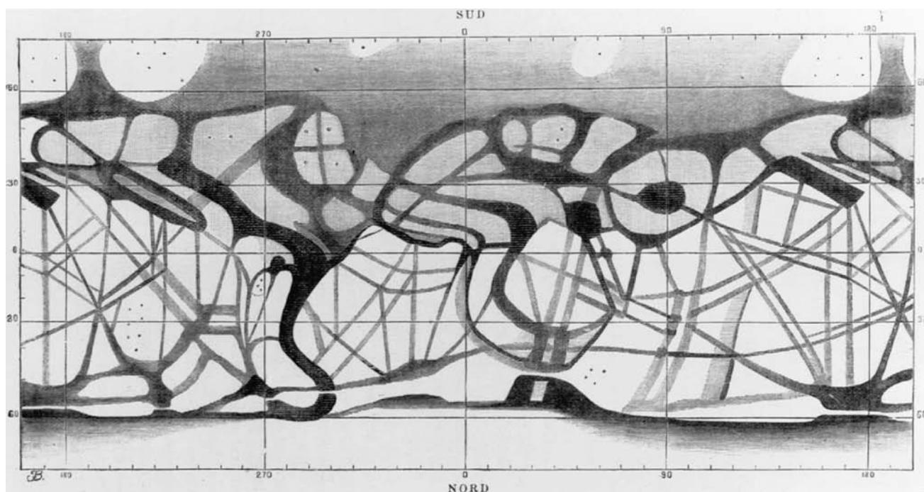
Fig. 8.5 Martian canals During the opposition of 1877, the Italian astronomer Giovanni Schiaparelli (1835–1910) mapped features he thought he saw on Mars, including a vast network of long, thin, straight lines criss-crossing the planet's surface. Some of the canals have apparently doubled, or divided in two, in this Mercator projection drawn by Schiaparelli during the opposition of 1881 using an 8.6-inch (22-centimeter) refractor. At this time, the apparent diameter of Mars was only 16 seconds of arc. Schiaparelli named these features canali , and they were likened to man-made water canals by subsequent observers, including Camille Flammarion (1842–1925) and Percival Lowell (1855–1916). Nevertheless, most astronomers failed to see the canals, and spacecraft have not detected them.
