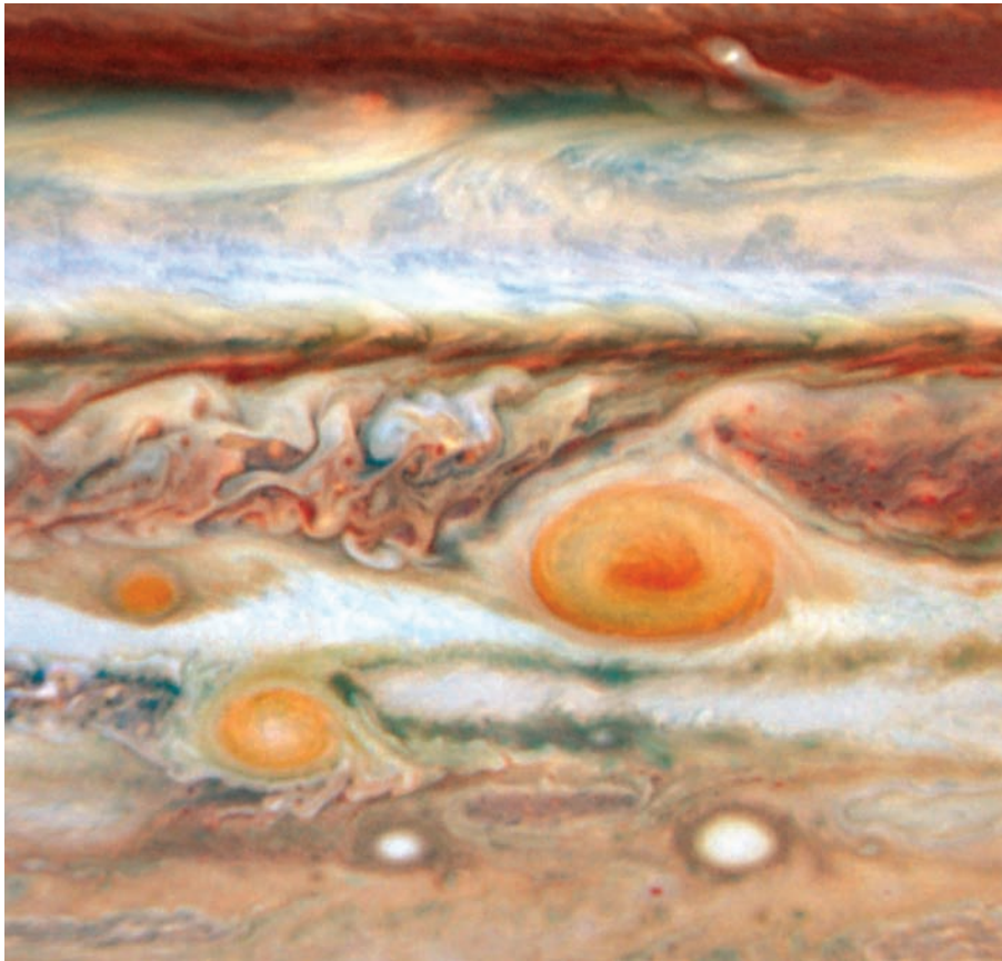
Fig. 9.3 New red spots on Jupiter Some of the turbulent eddies in Jupiter's atmosphere move from west to east ( left to right ) above Jupiter's Great Red Spot ( center ), a giant high-pressure anticyclone that swirls in the opposite counter-clockwise direction. Some small eddies are sucked into the great red vortex, helping to sustain it, while other eddies roll around the perimeter, probably reinforcing the storm's circulation. Although the Great Red Spot has been observed for at least three centuries, a new red spot appeared in the spring of 2006, and in 2008 a white oval-shaped storm turned into a third, smaller red spot. The small red oval ( left ) will either be absorbed or repelled by the Great Red Spot when it moves into it, but the other, lower latitude red spot, which lies between the other two, will most likely pass the Great Red Spot unhindered. This visible-light image was taken on 9–10 May 2008 from the Hubble Space Telescope . (Courtesy of NASA/ESA/Mike Wong and Imke de Pater, U. C. Berkeley.)
