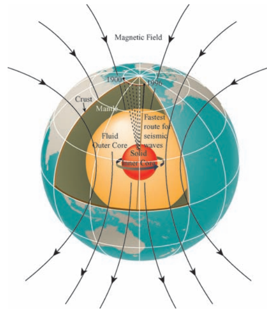
Fig. 4.4 The Earth's double core The mantle and part of the crust have been cut away here to show the relative sizes of the Earth's fluid and solid cores. The outer fluid core is about 55 percent of the radius of the Earth, and the inner solid core is slightly smaller than the Earth's Moon. The Earth's magnetic field is thought to be generated and sustained by moving currents in the planet's electrically conducting, fluid outer core, which is composed of molten iron. Geophysicists have discovered that the route of the rapid polar (north–south) waves through the Earth's interior is gradually shifting eastward because the inner core is rotating slightly faster than the rest of the planet. The fast rotation of the inner solid core may help explain how Earth's magnetic field reverses polarity. (Courtesy of Paul Richards, Lamont-Doherty Earth Observatory.)
