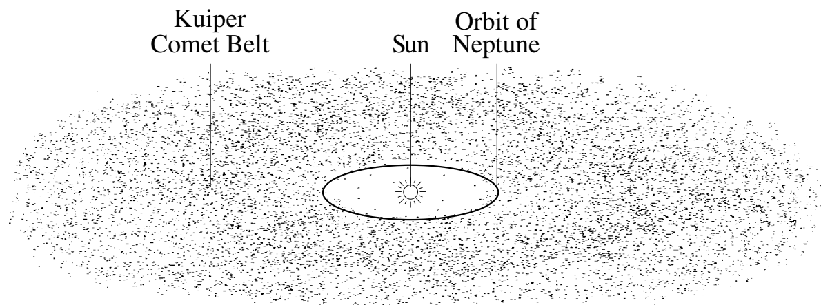
Fig. 14.9 The Kuiper belt of comets A repository of frozen, comet-sized worlds resides in the outer precincts of the planetary system, just beyond the orbit of Neptune and near the orbital plane of the planets. Known as the Kuiper belt, it is thought to contain 100 million to 10 billion comets. Many Jupiter-family comets are tossed into the inner solar system from the Kuiper belt. It is named after the Dutch-American astronomer Gerard Kuiper (1905–1973).
