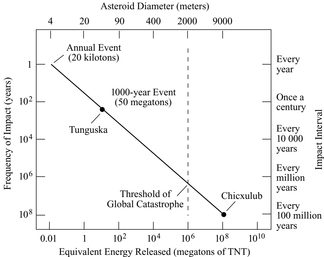
Fig. 13.12 Cosmic impact probabilities A hail of cosmic objects continually pelts the Earth from space. This plot shows the likelihood ( vertical axis ) that a member of the current population of Earth-crossing asteroids will hit our planet. An object two kilometers in diameter, capable of producing certain worldwide damage, hits the Earth every million years on average. An impact like the one that wiped out the dinosaurs, giving rise to the Chicxulub crater, is estimated to occur every 100 million years. Since smaller asteroids are much more numerous than larger ones, the smaller objects strike our planet more often. An impact like the Tunguska event, which occurred on 30 June 1908, might occur every 1000 years or so. The explosive energy of the impact is also given ( horizontal axis ) in units of megatons of exploded TNT. One hundred megatons ( 10^{11} kilograms) of TNT is equivalent to about 4 \times 10^{17} joules of energy, the amount released by a typical nuclear bomb on Earth.
