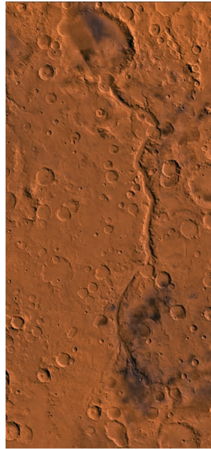
Fig. 8.23 Mars' Ma'adim Vallis and Gusev Crater A mosaic of Viking images reveals the branching, winding valley network named Ma'adim Vallis, which is about 800 kilometers long. It drains from the heavily cratered terrain in the south ( bottom ) and breaches the southern rim of the Gusev Crater ( top ), which formed earlier and is about 150 kilometers in diameter. The smooth flat crater floor suggested it was filled with water and sediments, but the Mars Exploration Rover , Spirit , failed to find any water-related sediments in the hypothetical crater lake, perhaps because they have been covered by volcanic flows. (Courtesy of NASA/JPL/USGS.)
