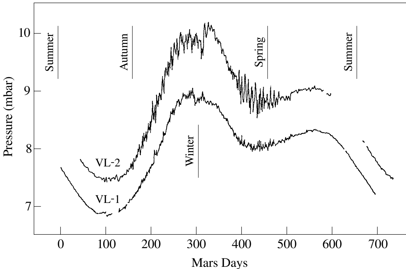
Fig. 8.7 Martian surface pressure Daily mean surface pressures at the two Viking Lander (VL) sites recorded for one Martian year, showing that the red planet periodically removes and replaces large amounts of carbon dioxide in its atmosphere. The seasons are for the northern hemisphere, and the pressure is given in millibars (mb), where 1 mb = 0.001 bar and 1 bar is the sea-level pressure of the Earth's atmosphere. At the Viking 1 site ( bottom curve ), the pressure ranged from 6.7 mb during the northern summer to 8.89 mb at the commencement of northern winter. At the Viking 2 site ( top curve ) the equivalent data were 7.4 mb and 10 mb. The higher values are probably due to the lower elevation; there was an approximate 1.1-kilometer difference in the elevation of the two landing sites. Dust storms are thought to produce some of the smaller non-seasonal pressure variations. The seasonal pressure differences seem to be dominated by the southern polar cap, which is larger than the northern one. In the southern winter, and northern summer, carbon dioxide is condensed out of the atmosphere, enlarging the southern polar cap and reducing the total surface pressure of the planet. In southern summer, and northern winter, the carbon dioxide has been released back into the atmosphere, with an increase in the total surface pressure.
