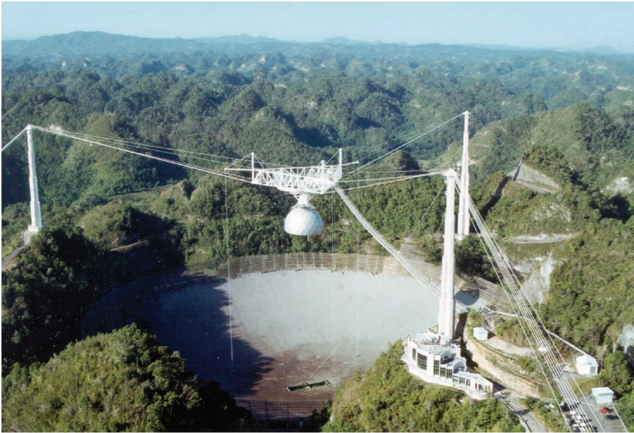
Fig. 6.2 Arecibo Observatory The world's largest radio telescope is nestled into the hills near Arecibo, Puerto Rico. Its metal reflecting surface has a spherical shape with a diameter of 305 meters. The reflected radio signals are focused to detectors suspended on the triangular structure hanging from the three towers. The facility can also transmit powerful radio pulses, sending them off the metal surface into space. Such pulses, sent and received from this giant telescope, first measured Mercury's rotation period in 1965. Until then it had been wrongly thought that Mercury kept one side permanently facing the Sun, with a rotation period equal to its orbital period.
