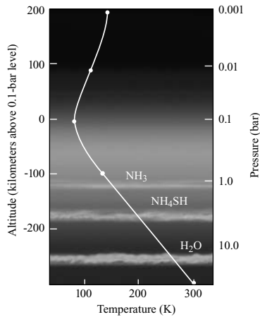
Fig. 10.5 Temperature and pressure at Saturn's cloud levels
