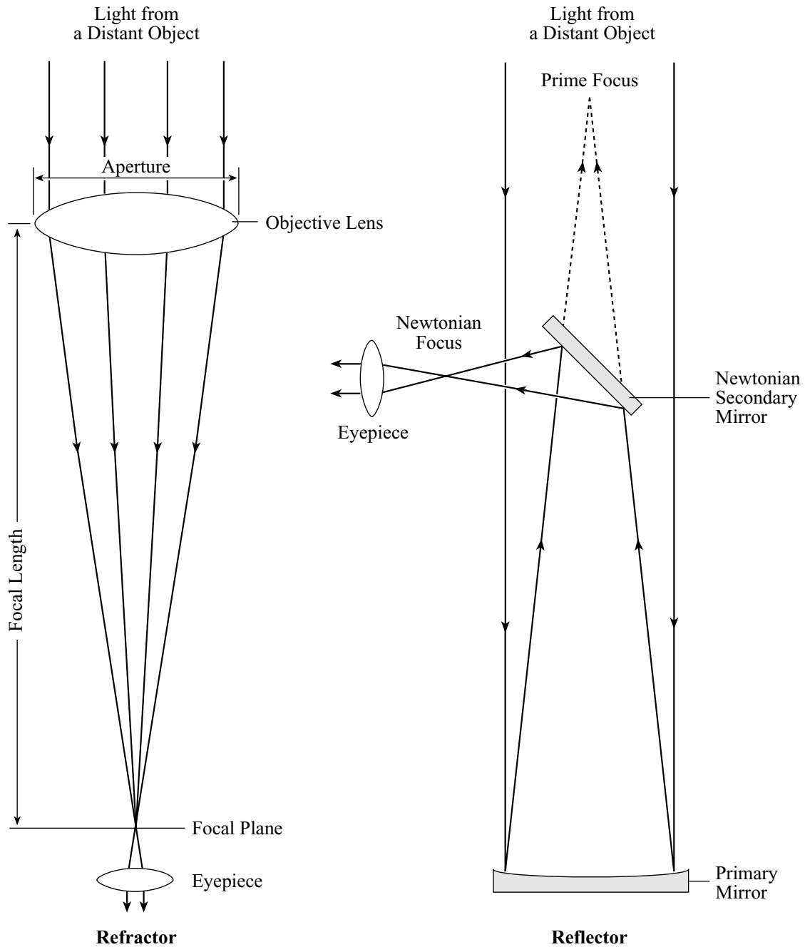
Fig. 1.17 Refractor and reflector Two kinds of optical telescopes, the refractor and the reflector, are used to gather and concentrate light at visible wavelengths. Light waves that fall on the Earth from a distant object are parallel to one another, and are focused to a point by the lens or mirror of a telescope. The earliest telescopes were refractors ( left ). The curved surfaces of the convex objective lens bend the incoming parallel light rays by refraction, and bring them to a focus at the center of the focal plane, where the light rays meet and an image is created. A second, smaller lens, called the eyepiece, was used to magnify the image in the early refractors; later versions placed photographic or electronic detectors at the focal plane. The reflecting telescope ( right ) uses a large, concave, or parabolic, primary mirror to collect and focus light. A small, flat secondary mirror, inclined at an angle of 45 degrees to the telescope axis, reflects the light sideways, at a place now known as the Newtonian focus. Other light-deflecting mirror arrangements can be used to obtain any desired focal length, which varies with the curvature and position of small convex mirrors.
