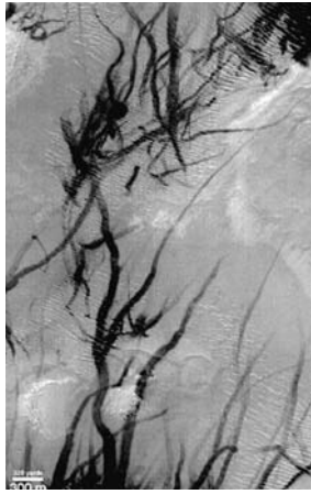
Fig. 8.9 Twisted paths of dust devils on Mars Spinning columns of warm air, called dust devils, rise above the Sun-heated surface of Mars. Each tornado-like vortex picks up light-colored dust, exposing the darker surface underneath. Dust devils have created this wild pattern of criss-crossing dark streaks in the rippled flats of Argyre Planitia, covering an area 3 by 5 kilometers at latitude of 51 degrees south. This image was taken from the Mars Global Surveyor in March 2000. (Courtesy of NASA/JPL/MSSS.)
