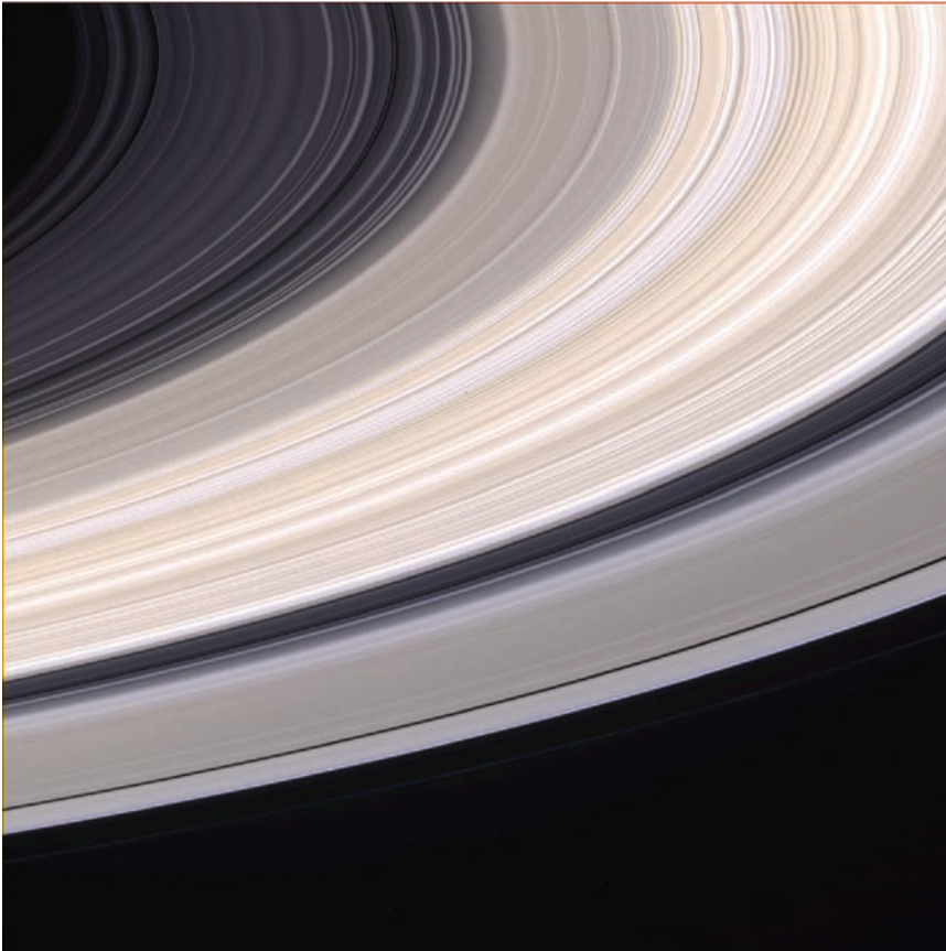
Fig. 10.9 Saturn's rings of ice The narrow-angle camera aboard the Cassini spacecraft took this image from beneath Saturn's ring plane on 21 June 2004. The brightest part of the ring system, extending from the upper right to the lower left, is the central B ring. It is separated from the outermost A ring by the wide, dark Cassini Division, discovered in 1675 by the Italian-born French astronomer Giovanni (Gian) Domenico (Jean Dominique) Cassini (1625–1712). Below the B ring, closer to the planet, is the C ring. All three rings are composed of innumerable particles of water-ice. The different shades of the rings are attributed to different amounts of contamination by other materials such as rock or carbon compounds. When viewed close up, the broad icy rings break up into thousands of individual wave-like ringlets. (Courtesy of NASA/JPL/SSI.)
