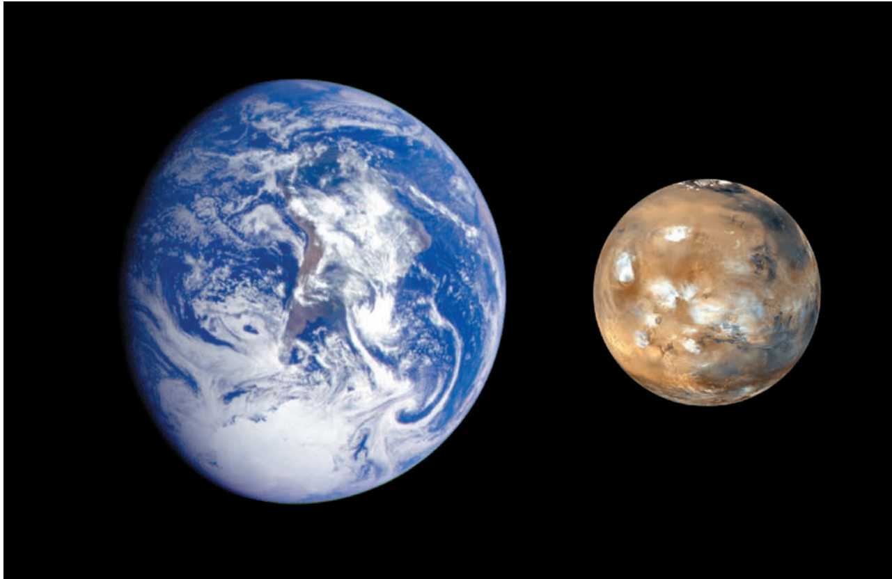
Fig. 8.1 Earth and Mars This composite image demonstrates the relative size, similarities and main difference of Earth ( left ) and Mars ( right ). Mars is about half the size of the Earth. Both planets exhibit clouds and polar caps. Bluish-white clouds of water ice hang above volcanoes on Mars ( right – center left ) and large dark areas extend across its red surface ( right – top right ). The residual north polar cap on Mars ( right top ) is made of water ice, and is circled by dark dunes of sand and dust. The Earth also has clouds and polar caps composed of water ice. However, about 75 percent of the Earth is covered with oceans, while liquid water cannot now exist for long times on the surface of Mars. The Earth image was taken from the Galileo spacecraft in December 1990, and the Mars Global Surveyor acquired the Mars image in April 1999. (Courtesy of NASA/JPL/MSSS.)
