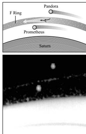
Fig. 10.13 Saturn's shepherd satellites Two shepherd satellites confine Saturn's narrow F ring. The outer shepherd gravitationally deflects ring particles inward, and the inner shepherd deflects ring particles outward. (Courtesy of NASA/JPL.)
