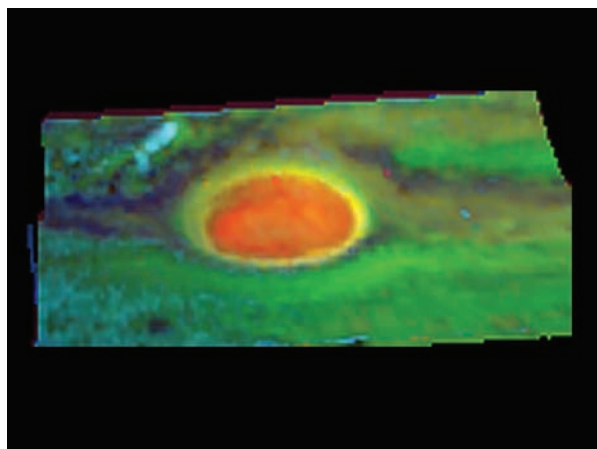
Fig. 9.5 Ammonia ice near Jupiter's Great Red Spot A cloud of ammonia ice (light blue) is shown at the northwest (upper left) of the Great Red Spot (middle), inside its turbulent wake. The cloud was most likely produced by powerful updrafts of ammonia-laden air from deep within Jupiter's atmosphere. Reddish-orange areas show high-level clouds, yellow regions depict mid-level clouds, and green areas correspond to lower-level clouds. Darker areas are cloud-free regions. Light blue depicts regions of middle-to-high altitude ammonia ice clouds. This near-infrared image was taken on 26 June 1996 from the Galileo spacecraft. (Courtesy of NASA/JPL.)
