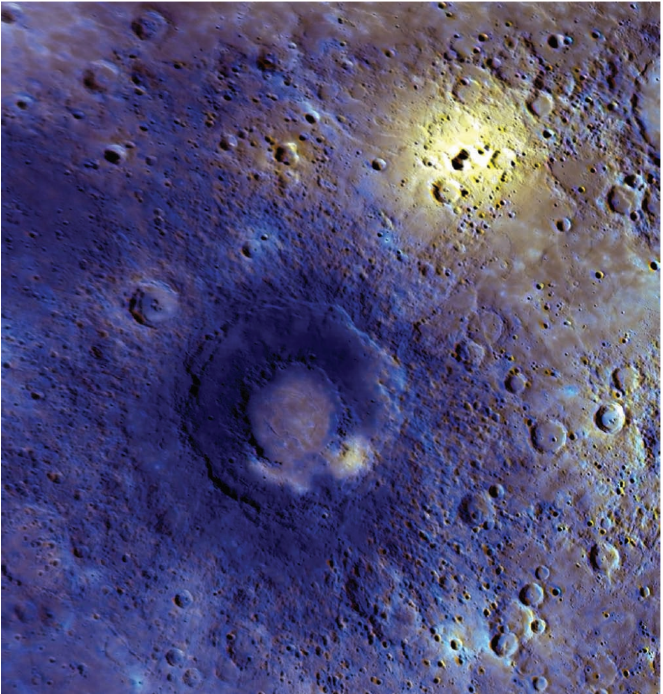
Fig. 6.15 Volcanic activity on Mercury This enhanced-color view, taken during the third flyby of Mercury by the MESSENGER spacecraft, enhances compositional differences in the features observed. The bright yellow area near the top right is centered on an irregular depression that is possibly an explosive volcanic vent. The double-ring basin in the center of this image may be filled by the flow of effusive volcanic lava; the basin is 290 kilometers in diameter. Smooth plains, thought to be the result of volcanic activity at earlier episodes than the others shown here, are located in much of the surrounding area. (Courtesy of NASA/JHUAPL/CIW.)
