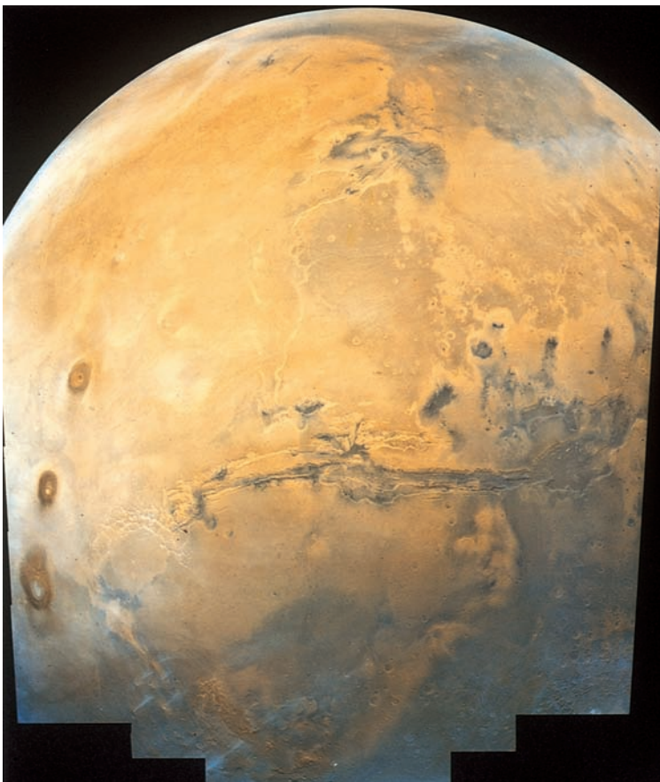
Fig. 2.8 Mosaic of Mars This computer-generated mosaic of Viking 1 and 2 orbiter images of Mars shows three volcanoes as dark spots to the west ( left ), while the bottom center of the scene shows the entire Valles Marineris canyon system, from Noctis Labyrinthus ( left ) to the chaotic terrain ( right ). Outflow channels are found in the north ( top ), and a variety of clouds and hazes are also visible, especially near the planet's edge. (Courtesy of NASA/USGS.)
