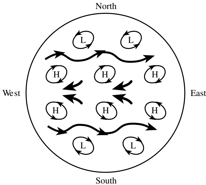
Fig. 3.3 Earth's weather patterns Trade winds blow from east to west along the Earth's equatorial regions, in the same direction that the planet rotates. At higher latitudes, there are high-altitude jet streams that move at speeds of up to 40 meters per second in the opposite direction to the trade winds. In the northern hemisphere there are high-pressure cyclones, denoted by H, and low-pressure anti-cyclones, L, rotating in the clockwise and counter-clockwise directions, respectively; in the southern hemisphere the cyclones and anti-cyclones rotate in the opposite direction. The prevailing winds are given in Annie Dillard's poem, "the windy planet".
