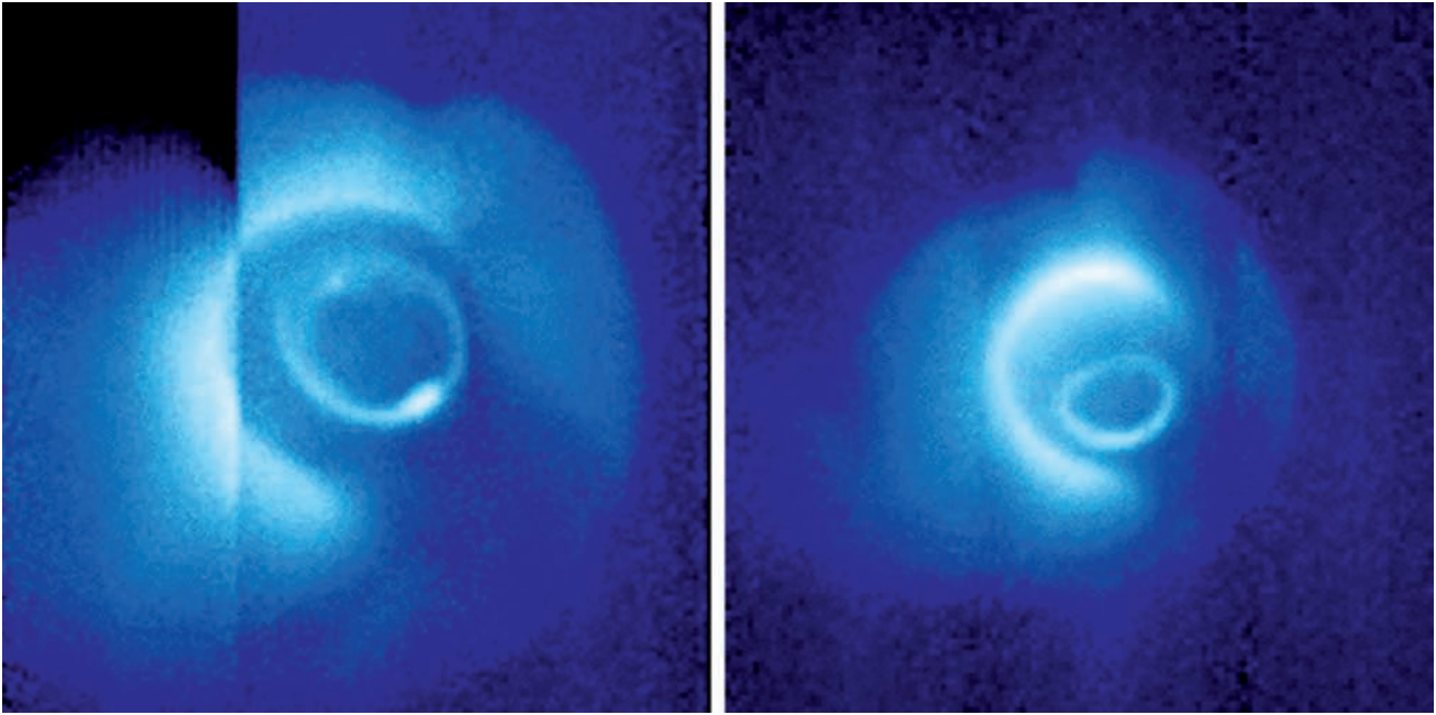
Fig. 3.16 Plasmasphere The Earth is surrounded by a layer of plasma, located in an inner part of the magnetosphere and just outside the ionosphere, which is at the top of the Earth's atmosphere. This plasmasphere is created by energetic sunlight ionizing molecules and atoms in the Earth's upper atmosphere, and it is contained by the Earth's magnetic field. Plasma is an electrically neutral collection of electrons, protons and other ions. These images were obtained on 24 May 2000 in ultraviolet light from the IMAGE spacecraft. The Earth is at the center of the images, and the Sun is to the upper left. The view is toward Earth's north pole. The emission of the plasmasphere is brightest on the side pointing toward the Sun. The oval shape of the Earth's northern aurora is detected inside the arc of the plasmasphere. (Courtesy of NASA/EUV IMAGE science team.)
