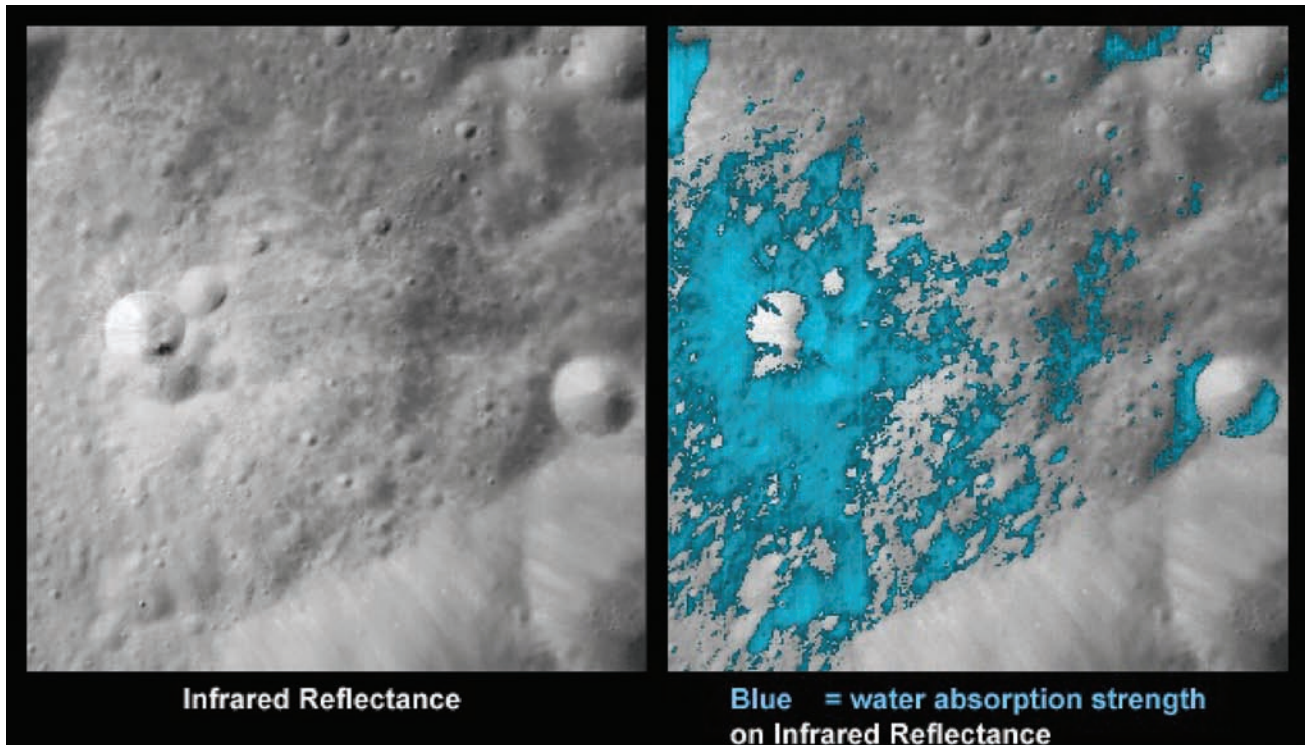
Fig. 5.27 Water around a fresh crater on the Moon These images show a very young crater or the side of the Moon that faces away from the Earth, as viewed from NASA's Moon Mineralogy Mapper instrument aboard the Indian Space Research Organization's Chandrayaan-1 lunar-orbiter spacecraft. Sunlight reflected at infrared wavelengths ( left ) shows a very young, fresh crater on the far side of the Moon. On the right, the distribution of water-rich minerals, seen in absorption at a specific infrared wavelength ( false-color blue ), is shown around the crater. Small amounts of both water and hydroxyl-rich material were found to be associated with material ejected from the crater, but the amount of water is very small. (Courtesy of ISRO, NASA, JPL-Caltech/USGS/Brown University.)
