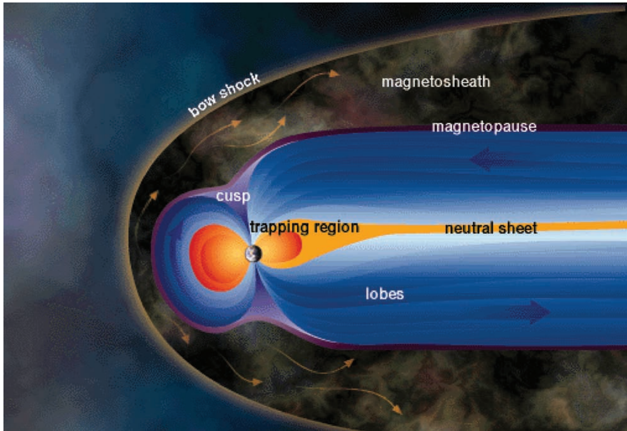
Fig. 3.13 Asymmetric magnetosphere The Earth's magnetic field carves out a hollow in the solar wind, creating a protective cavity called the magnetosphere (blue). It is sculpted into an asymmetric shape by the solar wind, with a bow shock that forms at about 10 Earth radii on the sunlit, dayside facing the Sun (left). The location of the bow shock is highly variable since it is pushed in and out by the gusty solar wind. The magnetopause marks the outer boundary of the magnetosphere, at the place where the solar wind takes control of the motions of charged particles. The solar wind is deflected around the Earth, pulling the terrestrial magnetic field into a long magnetotail on the nightside (right). The red regions in the inner magnetosphere contain the plasmasphere, the ring current and the outer Van Allen belt, where electrons, protons and other ions are trapped in closed paths. (Courtesy of ESA.)
