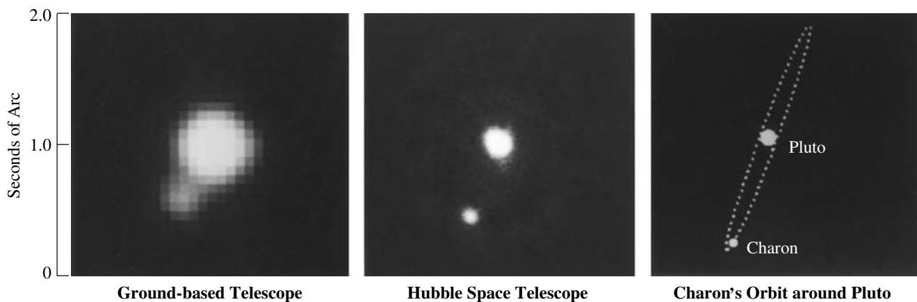
Fig. 15.3 A double object The Hubble Space Telescope (HST) distinguishes between Pluto, the bright object at the middle of the central image, and its companion Charon, which is the fainter object in the lower left of the central image. Observations from telescopes on Earth (left) were unable to clearly resolve the pair because of atmospheric distortions. At the time of the HST photograph, Charon's orbit around Pluto (right) was seen nearly edge-on, and Charon was near its maximum angular separation from Pluto, a mere 0.9 seconds of arc. Pluto's mean radius is 1153 kilometers, Charon is half that size, and the two objects are just 19 640 kilometers apart. The HST's ability to distinguish Pluto's disk at its distance of 4.4 billion kilometers is equivalent to seeing a baseball at a distance of about 100 kilometers. (Courtesy of NASA.)
