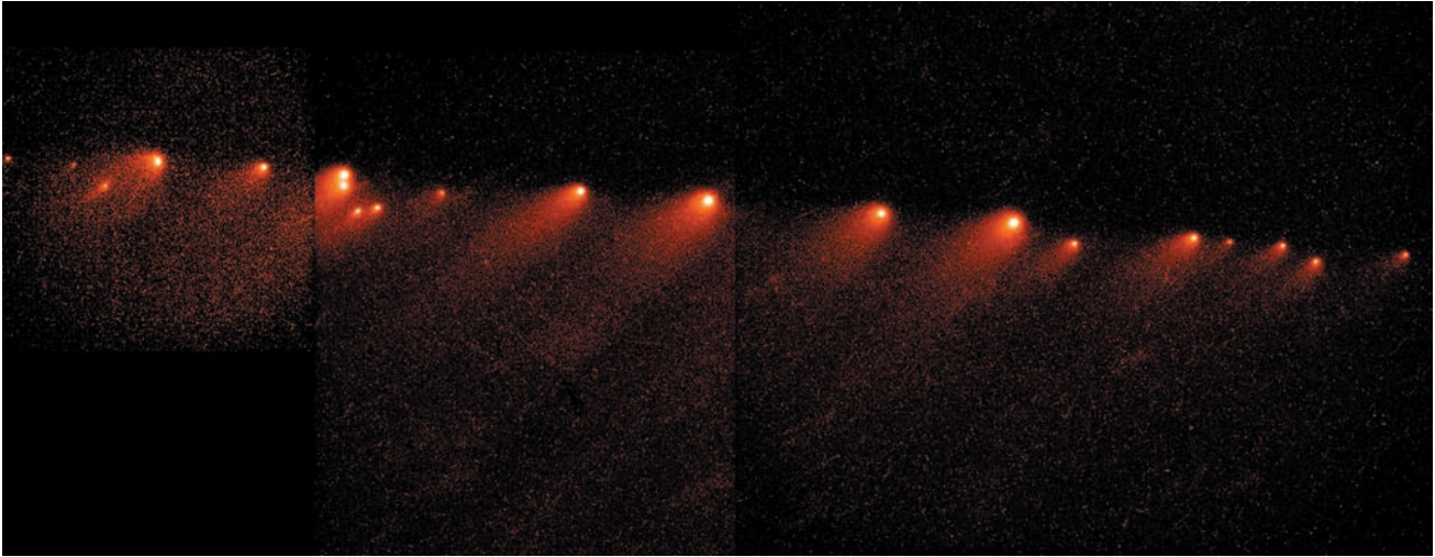
Fig. 13.1 Fragments of comet Shoemaker-Levy 9 In July 1992, this comet passed so close to Jupiter that the icy material of its nucleus was torn apart by the differential gravitational forces of the giant planet. This panoramic image of the comet fragments was taken from the Hubble Space Telescope in January 1994, eight months after they were discovered and six months before they dived into the atmosphere of Jupiter. The length of the string of comet pieces is about 1.1 million kilometers, three times the distance from the Earth to the Moon. The largest of the fragments in the string is about two kilometers across. Each fragment mimics a larger comet with a round coma and a dusty tail. (Courtesy of NASA/STScI.)
