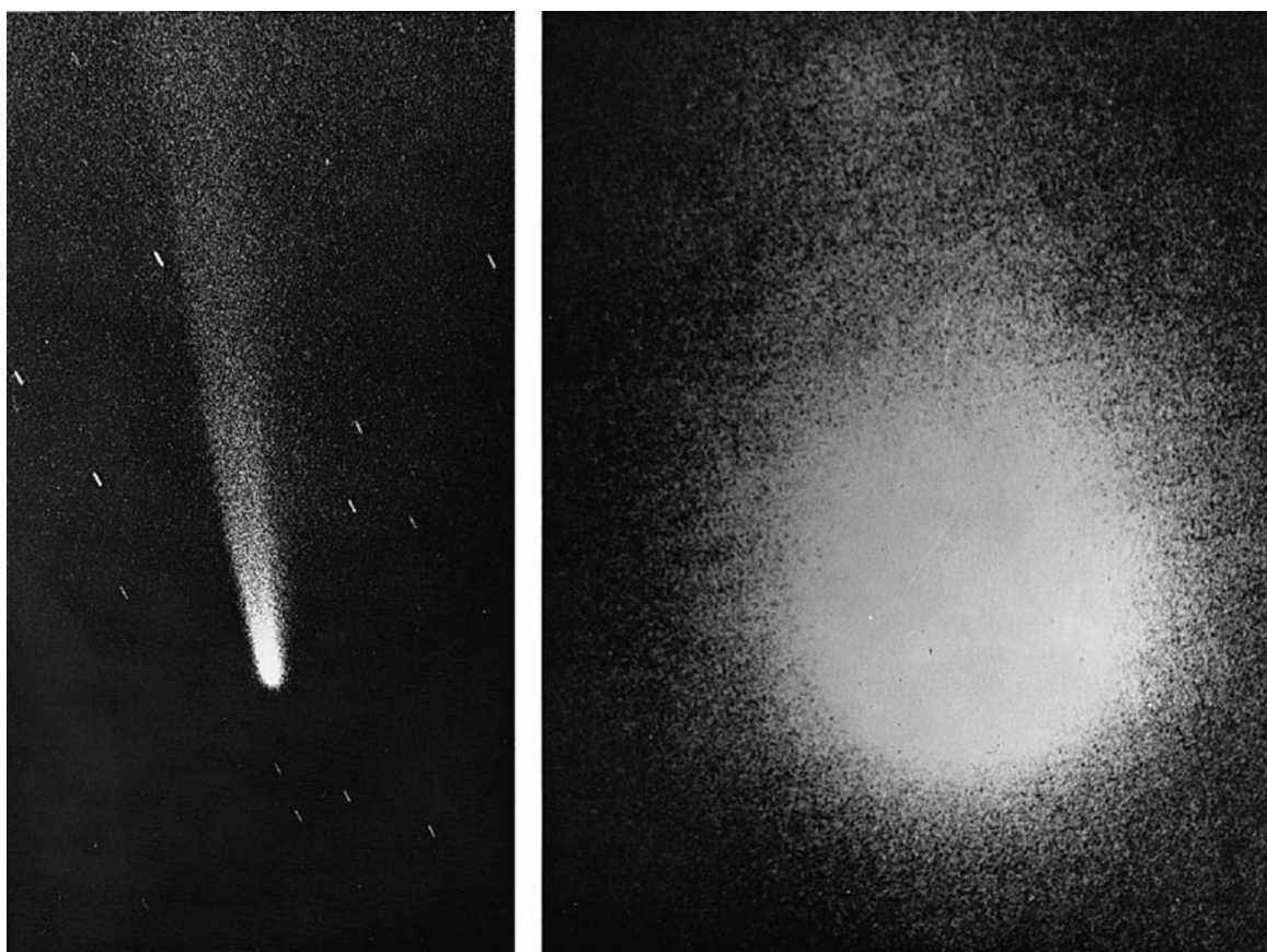
Fig. 14.12 Hydrogen cloud of a comet A comparison of the visible image ( left ) of comet Kohoutek with a far ultraviolet image ( right ) on the same scale, taken from Aerobee rocket flights on 4 and 7 January 1974. The ultraviolet image shows a gigantic cloud of hydrogen nearly 10 million kilometers in size, or about 10 times bigger than the Sun. It is being fed by the comet nucleus at the rate of 500 billion billion billion, or 5 \times 10^{29} , atoms of hydrogen every second. The large size of the hydrogen cloud is due to the fact that hydrogen atoms are much lighter, and move into space faster, than the other atoms, ions, molecules and dust particles, which produce the visible light of the coma. (Courtesy of Chet B. Opal, NRL.)
