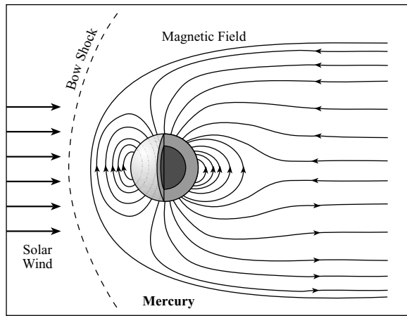
Fig. 6.18 Mercury's magnetic field and large core The magnetic field of Mercury is a miniature version of Earth's magnetic field, complete with bow shock, magnetosphere and magnetotail. Mercury's magnetic axis is closely aligned with its rotation axis, and its polarity is the same as the Earth's, with magnetic south corresponding to geographic north. This magnetic field is probably generated within the planet's large iron core, but the exact mechanism for creating the field remains a mystery. The electrified solar wind compresses the magnetic field into a bow shock on the sunlit side and draws it out into a tail on the opposite side.
