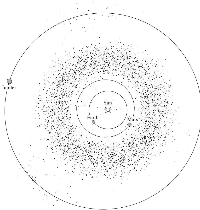
Fig. 1.16 Asteroid belt The exact locations of 5000 flying rocks, called asteroids or minor planets, whose orbits are accurately known. The vast majority of the asteroids orbit the Sun in the main belt located between the orbits of Mars and Jupiter. A few of them pass inside the orbit of Earth, while others move about 60 degrees ahead of and behind Jupiter in similar orbits. (Courtesy of Jeff Bytof, University of California at San Diego.)
