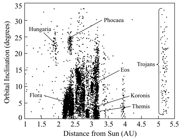
Fig. 12.5 Asteroid families The orbital parameters of many asteroids are very similar, as shown in this diagram of orbital inclination ( vertical axis ) plotted as a function of orbital distance from the Sun ( horizontal axis ). Three families with common orbital elements are the Koronis, Eos and Themis families. The Flora family is sometimes subdivided into several separate ones. The Hungaria and Phocaea group of asteroids at high inclinations are separated from the main belt by secular resonance with Jupiter, that clears asteroids out of certain locations, and they are not true families. The Kirkwood gaps, also cleared by resonance, are noticeable by vertical white spaces; the one at 2.5 AU corresponds to an orbital period of 4 years and the 3 : 1 resonance. Another sharp break is present at 3.3 AU, corresponding to a period of 6 years and the 2 : 1 resonance. [Adapted from Charles T. Kowal's Asteroids (New York: John Wiley, 1996).]
