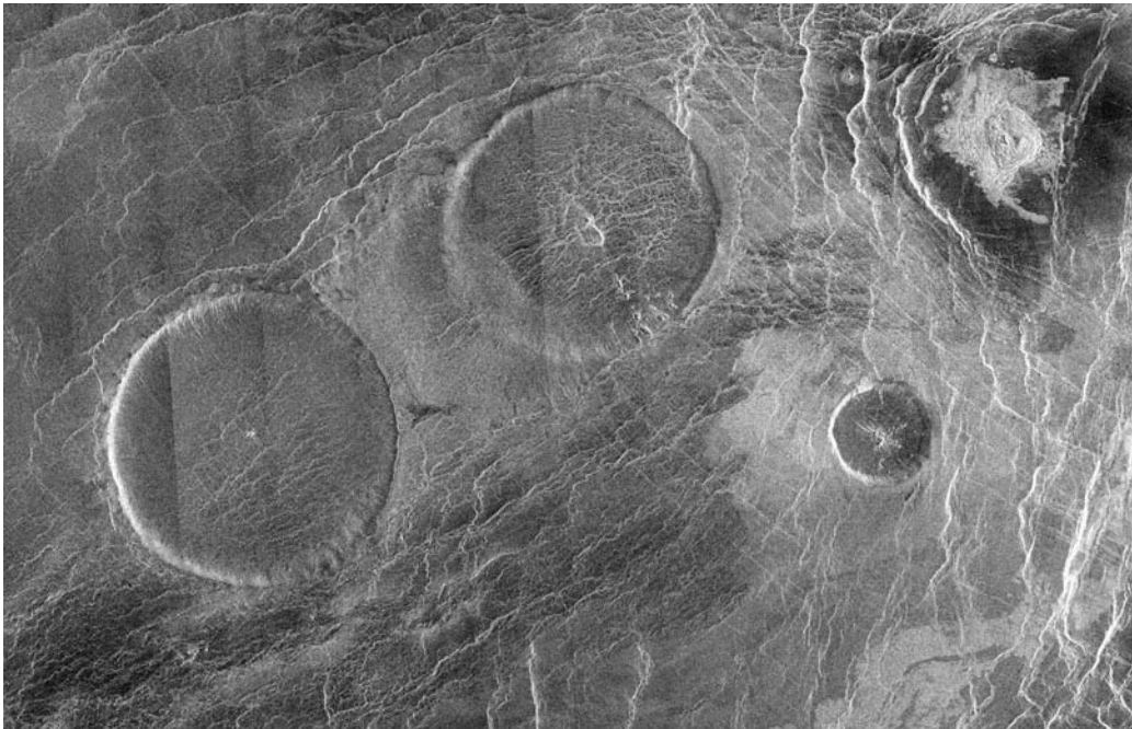
Fig. 7.22 Volcanic pancake domes This Magellan radar image, centered in the Eistia Regio at 12.3 degrees north latitude and 8.6 degrees east longitude, shows an area 250 kilometers wide. The prominent circular features are volcanic pancake domes, each about 65 kilometers across, with broad, flat tops less than one kilometer in height. They are formed from viscous, or sticky, lava, and include cracks and pits that result from cooling and withdrawal of the lava. (Courtesy of NASA/JPL.)
