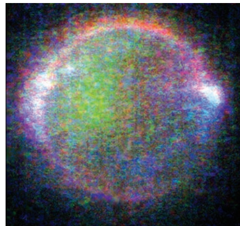
Fig. 9.17 Aurora on Jupiter's moon Io The ghostly glow of aurora are detected in the atmosphere of Io when the satellite is in Jupiter's shadow. The aurora is produced by energetic particles, which are trapped in Jupiter's magnetic field and collide with Io's atmospheric gases, creating a red and green glow analogous to the aurora of Earth. Blue light is caused by dense volcanic plumes and may indicate regions that are electrically connected to Jupiter itself. (Courtesy of NASA/JPL/U. Arizona.)
