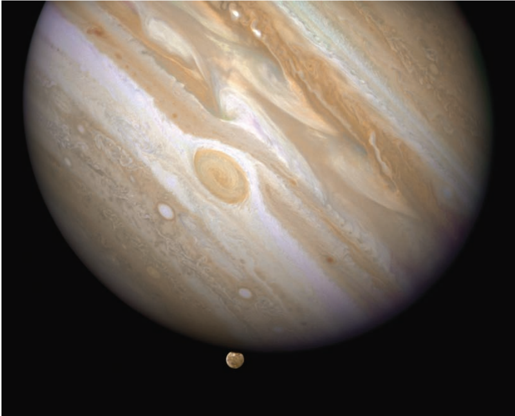
Fig. 9.1 Jupiter and its moon Ganymede The icy surface of Ganymede, Jupiter's largest moon, is seen just before it passes behind the planet ( bottom ). The giant Jupiter is portrayed in close to natural color, including its Great Red Spot ( center ), the biggest and oldest known storm in the solar system. The spot's east-west diameter is more than twice that of Earth, and one-sixth the diameter of Jupiter itself, and the red swirling vortex has been observed for at least 300 years. By watching Jupiter eclipsing its moon Ganymede, astronomers have searched for haze that causes a slight dimming at different colors. This image was taken on 9 April 2007 from the Hubble Space Telescope . (Courtesy NASA/ESA/E. Karkoschka, U. Arizona.)
