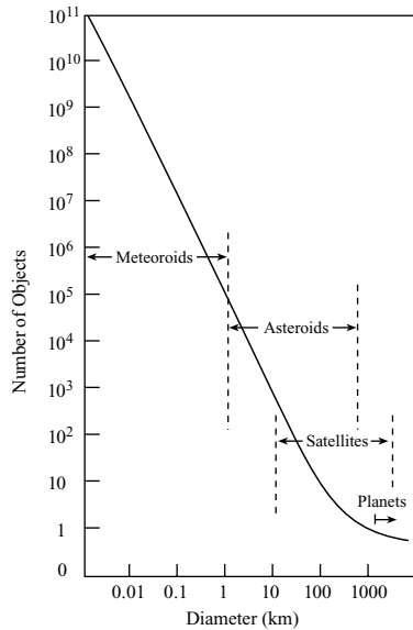
Fig. 12.25 Interplanetary objects Repetitive collisions between interplanetary objects have produced many more small meteoroids than large ones. Some of the largest asteroids are comparable in size to small moons, and ongoing collisions between asteroids have produced numerous smaller meteorites.
