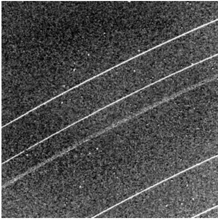
Fig. 11.8 The rings of Uranus This Voyager 2 image, taken on 23 January 1986, shows five of the nine rings of Uranus that had been previously inferred from Earth-based observations of their brief occultation of a star's light. In this view, sunlight striking the rings' particles was reflected back toward the camera, showing that the dense parts of the ring system consist of narrow rings with wide gaps. In contrast, Saturn's main rings are broad with narrow gaps. From bottom to top, the rings are designated by the Greek letters \alpha , \beta , \eta , \gamma and \delta . (Courtesy of NASA/JPL.)
