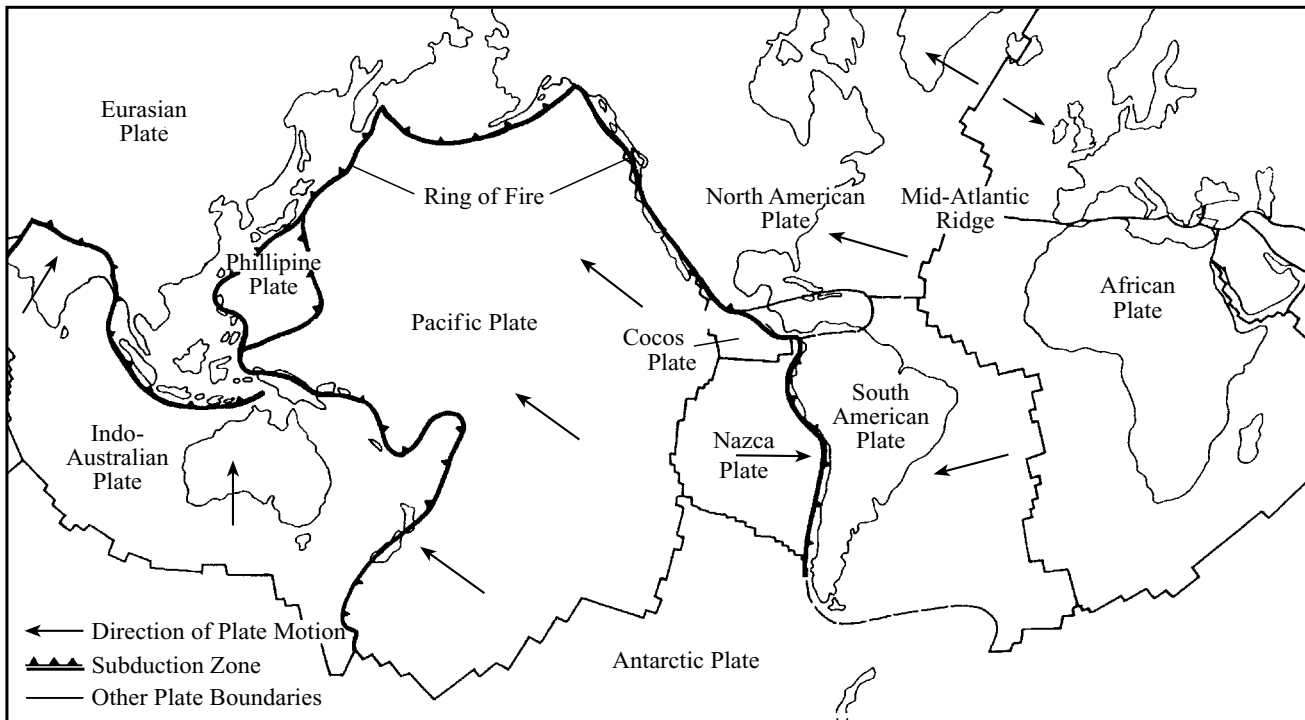
Fig. 4.12 Earth's moving plates The Earth's lithosphere is broken into numerous plates. They move in the directions shown by the arrows at rates of about a tenth of a meter per year. The lithosphere dives into the underlying asthenosphere at zones of subduction. They are denoted by the thick line with triangles, forming the famous Ring of Fire around the edge of the Pacific and Nazca Plates. Most of the Earth's earthquake and continental volcanic activity is concentrated along the subduction zones.
