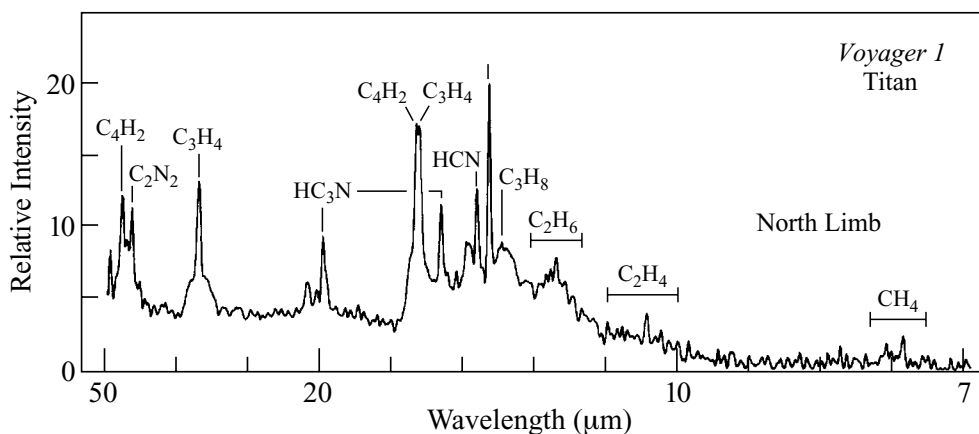
Fig. 10.24 Molecules in Titan's atmosphere Emission features in the infrared spectrum of Titan's reflected sunlight identify the molecular constituents of its atmosphere. Sharp peaks in this spectrum, acquired from the Voyager 1 spacecraft in 1980, are attributed to methane ( \text{CH}_4 ), acetylene ( \text{C}_2\text{H}_2 ), ethane ( \text{C}_2\text{H}_6 ), and more complex hydrocarbon molecules, as well as nitrogen compounds. The wavelength is given in units of microns ( \mu\text{m} ), or 10^{-6} meters.
