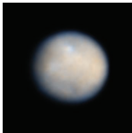
Fig. 12.6 Dwarf planet-asteroid 1 Ceres A Hubble Space Telescope image of 1 Ceres, the largest object in the asteroid belt and the first object discovered there. The round shape led to its classification in 2006 as a dwarf planet, and suggested that its interior is layered, with a rocky core, icy mantle and thin, dusty outer crust. Ceres is approximately 950 kilometers across. The differences between lighter and darker regions could be impact features or simply due to a variation in surface material. (Courtesy of NASA/ESA/J. Parker, SRI, P. Thomas, Cornell U., L. McFadden, U. Maryland, and M. Mutchler and Z. Levay, STScI.)
