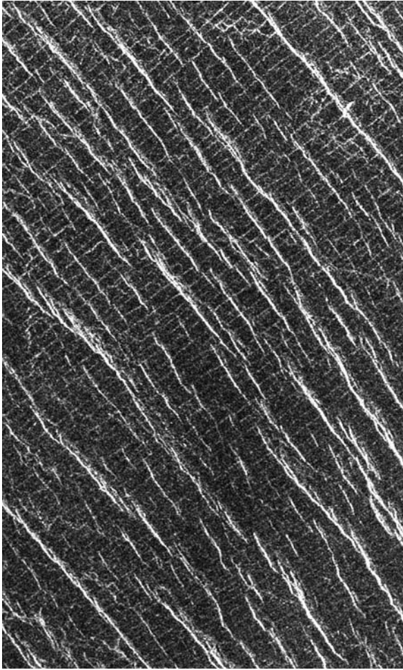
Fig. 7.23 Tesserae Because there is little soil and no vegetation or erosion to confuse us, we can see tectonic patterns on Venus much more easily than on our own planet. This region, covering an area of 37 kilometers wide by 80 kilometers long, is located at 30 degrees north latitude and 333 degrees east longitude, on the low rise separating Sedna Planitia and Guinevere Planitia. It shows a criss-crossed pattern of radar-bright lines, which appear to be faults or fractures. The orthogonal system of ridges and grooves is formed in elevated terrain (by 1 or 2 kilometers), and spaced at regular intervals of 1 to 20 kilometers. Known as tesserae , from the Latin word for “tiles”, the features suggest repeated episodes of intense surface fracturing that may be unrelated to volcanic activity. This type of terrain is not seen on any other planet. It covers about 8 percent of Venus’s surface. Sedna is an Eskimo goddess whose fingers became seals and whales, and Guinevere is the legendary Queen of the British King Arthur. (Courtesy of NASA.)
