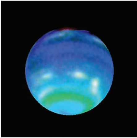
Fig. 11.4 Neptune's stormy disposition The weather on Neptune is recorded in this image, which combines simultaneous observations on 11 August 1998 with the Hubble Space Telescope and NASA's InfraRed Telescope Facility on Mauna Kea, Hawaii. The predominant blue color of the planet is a result of absorption of red and infrared light by Neptune's methane atmosphere. Clouds elevated above most of the methane absorption appear white. Neptune's powerful jet stream, where winds blow at nearly 400 meters per second, is centered at the dark blue belt near Neptune's equator. The Great Dark Spot detected when the Voyager 2 spacecraft visited Neptune in August 1989 has completely disappeared in this image, taken nine years later. (Courtesy of NASA/STSCI/IRTF.)
