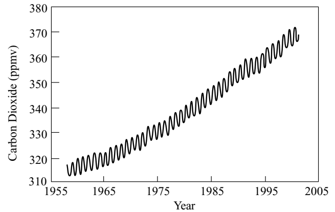
Fig. 4.21 Rise in Earth’s atmospheric carbon dioxide The average monthly concentration of atmospheric carbon dioxide (CO 2 ) in parts per million by volume (ppmv) of dry air plotted against time in years observed since 1958 at the Mauna Loa Observatory, Hawaii. It shows that atmospheric amounts of the principal waste gas of industrial societies, carbon dioxide, have risen steadily for more than forty years. The up and down fluctuations superimposed on the systematic increase reflect a seasonal rise and fall in the absorption of carbon dioxide by trees and other vegetation. Summertime lows are caused by the uptake of carbon dioxide by plants, and the winter highs occur when the plants’ leaves fall and some of the gas is returned to the air. (Courtesy of Dave Keeling and Tim Whorf, Scripps Institution of Oceanography.)
