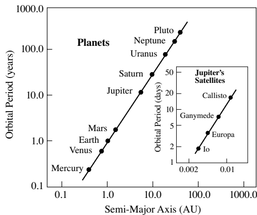
Fig. 1.13 Kepler's third law The orbital periods of the planets are plotted against their semi-major axes, using a logarithmic scale. The straight line that connects the points has a slope of 3/2 , thereby verifying Kepler's third law that states that the squares of the orbital periods increase with the cubes of the planetary distances. This type of relation applies to any set of bodies in elliptical orbits about a much larger mass, including Jupiter's four largest satellites shown in the inset.
