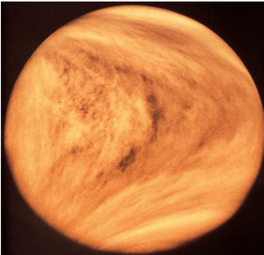
Fig. 7.2 Cloud tops of Venus Clouds of sulfuric acid permanently shroud Venus’ surface from view. The horizontal Y-shaped clouds near the equator move from east to west along with high-speed winds at velocities of up to 100 meters per second, circling the planet every four Earth days. This image was taken from the Mariner 10 spacecraft when it encountered Venus on 5 February 1974, using its gravitational influence to be flung on to Mercury. Similar features have been seen in violet or ultraviolet light from the Mariner 10 , Pioneer Venus , Galileo , and Venus Express spacecraft, as well as from the Hubble Space Telescope . (Courtesy of NASA.)
