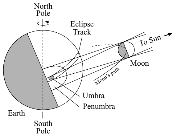
Fig. 5.5 Solar eclipse During a solar eclipse, the Moon casts its shadow upon the Earth. No portion of the Sun's photosphere can be seen from the umbra region of the Moon's shadow ( small gray spot ); but the Sun's light is only partially blocked in the penumbra region ( larger half circle ). A total solar eclipse, observable only from the umbra region, traces a narrow path across the Earth's surface.
