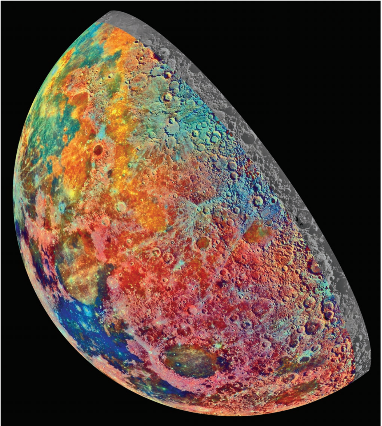
Fig. 5.23 Compositional variations on the Moon's surface This mosaic of images, taken through three spectral filters, shows exaggerated false-color differences in reflected sunlight in order to specify composition differences on the lunar surface. The image shows volcanic flows with relatively high titanium content ( blue ), volcanic flows that are low in titanium but rich in iron and magnesium ( green, yellow and light orange ), and heavily cratered highlands that are typically poor in titanium, iron and magnesium ( pink and red ). In this view, taken by Galileo on 7 December 1992, bright pink highlands surround the lava-filled Crisium impact basin ( bottom ), and the dark blue Mare Tranquillitatis ( left ) is richer in titanium than the green and orange maria above it. The youngest craters have prominent blue rays extending from them. (Courtesy of NASA/JPL.)
