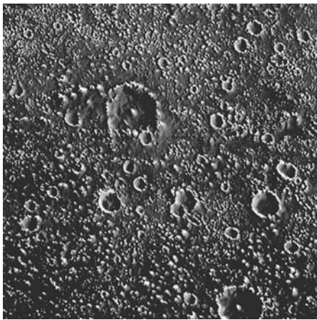
Fig. 9.25 Dark material and few small craters on Callisto A dark, mobile blanket of fine material covers Callisto's surface, sometimes collecting within crater walls. While Jupiter's moon Callisto is saturated with large impact craters, it has fewer very small craters when compared with the Earth's Moon and Mercury. One explanation is that the smaller craters have been filled by dark material that has moved down surface slopes. An alternative explanation for the paucity of little craters on Callisto is that there were fewer small impacting objects in its vicinity when compared with the amount within the inner solar system. This image, about 74 kilometers across, was taken from the Galileo spacecraft on 17 September 1997. (Courtesy of NASA/JPL.)
