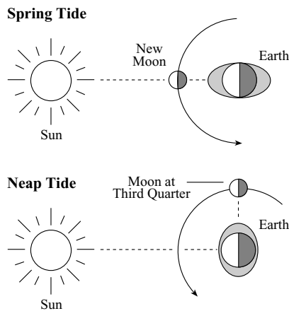
Fig. 5.30 Earth's spring and neap ocean tides The height of the tides and the phase of the Moon depend on the relative positions of the Earth, Moon and Sun. When the tide-raising forces of the Sun and Moon are in the same direction, they reinforce each other, making the highest high tides and the lowest low tides. These spring tides ( top ) occur at new or full moon. The range of tides is least when the Moon is at first or third quarter, and the tide-raising forces of the Sun and Moon are at right angles to each other. The tidal forces are then in opposition, producing the lowest high tides and the highest low tides, or the neap tides ( bottom ). The height of the tides has been greatly exaggerated in comparison to the size of the Earth.
