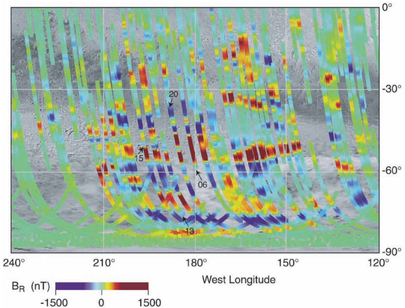
Fig. 8.2 Magnetic stripes on Mars Alternating bands of magnetic polarity are most prominent in this part of the southern highlands, near Terra Cimmeria and Terra Sirenum. The magnetic data were obtained from an instrument aboard the Mars Global Surveyor . This map is color-coded red for a positive magnetic field pointing out of the planet and blue for a negative one pointing in, with a strength up to 1500 nanotesla, or 1.5 \times 10^{-6} tesla. Stripes of alternating polarity, or direction, extend up to 2000 kilometers across the planet in the east-west direction. They are similar to the magnetic patterns seen in the Earth's crust at both sides of the mid-oceanic ridges, where the spreading crust has recorded flip-flop reversals in the Earth's dipolar magnetic field. (Courtesy of NASA/JPL/GSFC.)
