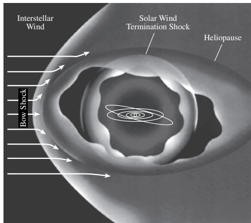
Fig. 3.11 Heliosphere With its solar wind going out in all directions, the Sun blows a huge bubble in space called the heliosphere. The heliopause is the name for the boundary between the heliosphere and the interstellar gas outside the solar system. Interstellar winds mold the heliosphere into a non-spherical shape, creating a bow shock where they first encounter it. The orbits of the planets are shown near the center of the drawing.
