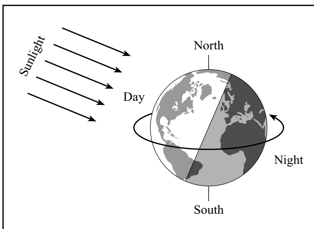
Fig. 1.7 Night and day The Earth rotates with respect to the Sun once every 24 hours, causing the sequence of night and day. Each point on the Earth's surface moves in a circular track parallel to the equator, and each track spends a different time in the Sun depending on the season. This drawing depicts summer in the northern hemisphere and winter in the southern hemisphere. Because the northern part of the Earth's rotational axis is tipped toward the Sun, circular tracks in the northern hemisphere spend a longer time in the Sun than southern ones.
