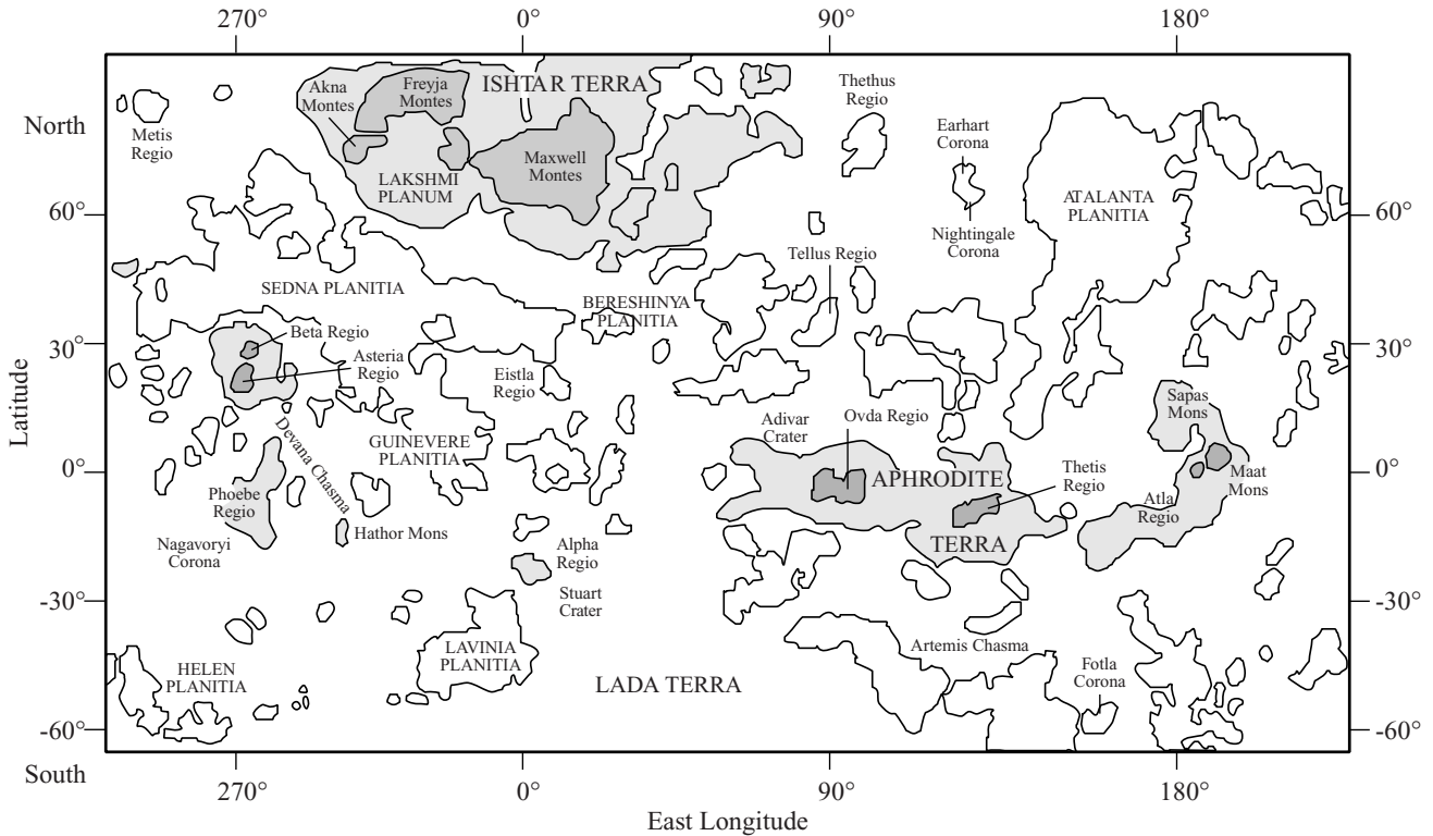
Fig. 7.12 Major surface features on Venus Most of Venus lies at roughly the same radius, in the lowland, volcanic plains ( white areas ). The highland massifs ( dark areas ) include Aphrodite Terra, an elongated feature extending along the equator between 70 degrees and 210 degrees east longitude. Many of the elevated regions near the equator mark the sites of volcanism, such as Maat Mons and Sapas Mons (see Fig. 7.16). The other main elevated region is Ishtar Terra in the north at about 0 degrees longitude ( center top ). Ishtar Terra is roughly the size of Australia. The elevated plateau in the western part of Ishtar Terra is known as Lakshmi Planum, which is bounded on three sides by mountains (see Fig. 7.17), including Maxwell Montes. This mountain's 11-kilometer height above the average radius exceeds by two kilometers the height of Mount Everest above sea level.
