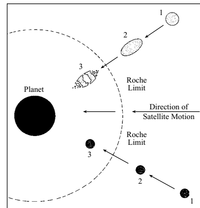
Fig. 10.17 The Roche limit A large satellite ( top ) that moves well within a planet's Roche limit ( dashed curve ) will be torn apart by the tidal force of the planet's gravity. The side of the satellite closer to the planet feels a stronger gravitational pull than the side farther away, and this difference works against the self-gravitation that holds the body together. A small solid satellite ( bottom ) can resist tidal disruption because it has significant internal cohesion in addition to self-gravitation.
