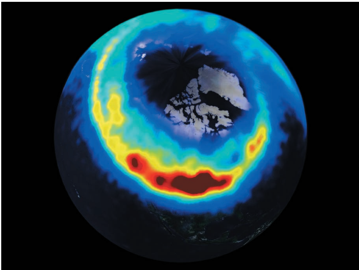
Fig. 3.23 The aurora oval The POLAR spacecraft looks down on an aurora from high above the Earth's north polar region in February 2000, showing the Northern Lights in their entirety. The glowing oval is 4500 kilometers across. The most intense aurora activity appears in bright red or yellow. (Courtesy of NASA/U. Iowa.)
