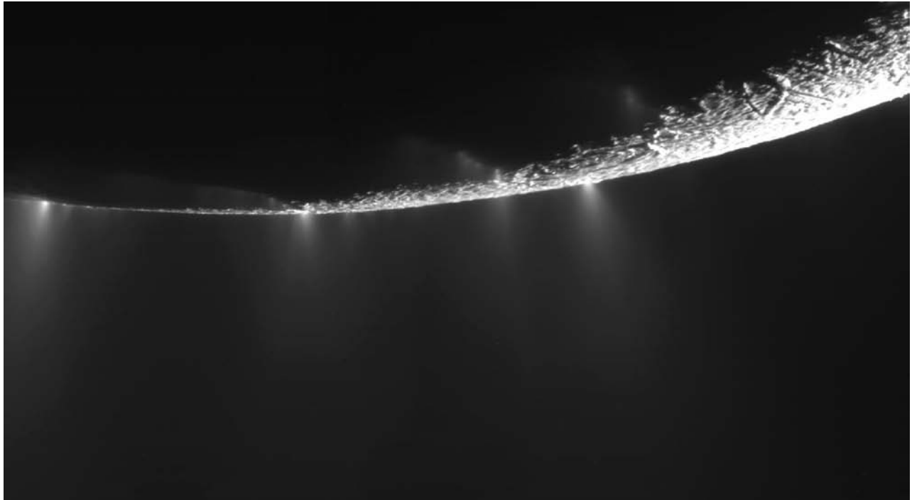
Fig. 10.22 Enceladus vents water jets Dramatic plumes, both large and small, spray out water-ice particles, water vapor and organic compounds from many locations along tiger-stripe fractures near the south pole of Saturn's moon Enceladus. More than 30 individual jets of different sizes can be seen in this image, and more than 20 of them had not been identified before. The south pole of Enceladus lies near the limb in the top left quadrant of the mosaic, near the large jet that is second from left. (Courtesy of NASA/JPL/SSI.)
