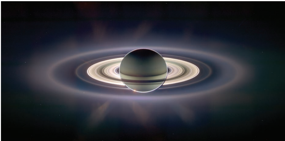
Fig. 2.13 In Saturn's shadow This marvelous panoramic view of Saturn and its rings was created from 165 images taken by a wide-angle camera aboard the Cassini spacecraft on 15 September 2006, as it drifted into the darkness of Saturn's shadow and permitted observations of the planet's tiny ring particles. The narrowly confined G-ring resides just outside the bright, inner main rings. The outer, wide E-ring encircles the entire system; icy plumes feed the E-ring from Saturn's satellite Enceladus. The exaggerated color contrast in this mosaic view can be used to infer processes that are sorting the ring particles according to their size. (Courtesy of NASA/JPL/SSI.)
