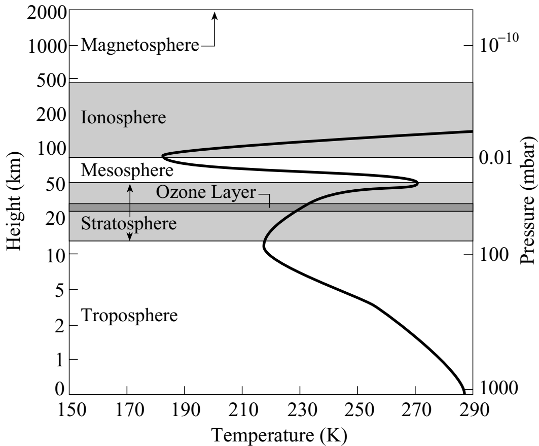
Fig. 4.19 Earth's layered atmosphere The pressure of our atmosphere ( right scale ) decreases with altitude ( left scale ; note that both the pressure and altitude scales are logarithmic). This is because fewer particles are able to overcome the Earth's gravitational pull and reach higher altitudes. The temperature ( bottom scale ) also decreases steadily with height in the ground-hugging troposphere, but the temperature increases in two higher regions that are heated by the Sun. They are the stratosphere, with its critical ozone layer, and the ionosphere. The stratosphere is mainly heated by ultraviolet radiation from the Sun, and the ionosphere is created and modulated by the Sun's X-ray and extreme ultraviolet radiation.
