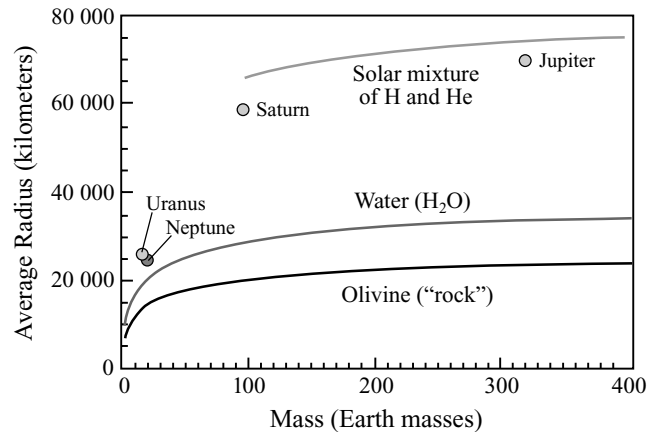
Fig. 11.5 Radius-mass relations A liquid body of solar composition describes a radius-mass relation (top) that approximates the mass and radius of Jupiter and Saturn. They consist mainly of the lightest element hydrogen (H) and next lightest abundant element helium (He). Uranus and Neptune contain little hydrogen or helium, for their radii are much too small to be consistent with a solar composition. Instead, they lie only slightly above the mass-radius relation for liquid water, so they probably contain large quantities of water. For comparison purposes, the bottom curve describes a giant planet composed of pure rock, as the Earth is but with a much smaller size.
