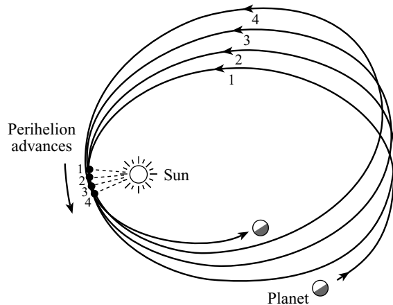
Fig. 6.19 Precession of Mercury's perihelion Instead of always tracing out the same ellipse, the orbit of Mercury pivots around the focus occupied by the Sun. The point of closest approach to the Sun, the perihelion, is slowly rotating ahead of the point predicted by Newton's theory of gravitation. This was at first explained by the gravitational tug of an unknown planet called Vulcan thought to be revolving about the Sun inside Mercury's orbit, but we now know that Vulcan does not exist. Mercury's anomalous motion was eventually explained by Einstein's new theory of gravity in which the Sun's curvature of space makes the planet move in a slowly revolving ellipse.
