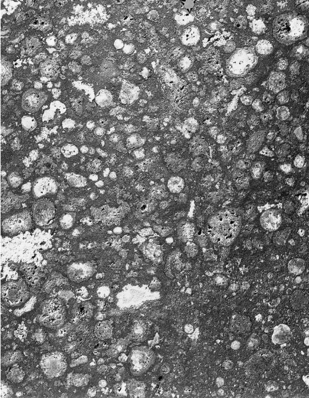
Fig. 12.21 Chondrules in Allende This photomicrograph of a thin section of the Allende meteorite shows numerous round silicate chondrules together with irregular inclusions. The meteorite section is 0.021 meters across and 0.027 meters high. (Courtesy of the Smithsonian Institution.)
