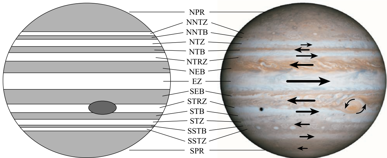
Fig. 9.2 Banded wind-blown clouds on Jupiter The traditional nomenclature of Jupiter's light and dark bands of clouds (left) is given in abbreviated form (center). The dark bands are called belts, denoted by "B", the light bands are known as zones, or "Z", and the rest of each name is based on climatic regions at the corresponding latitudes on Earth. North, letter "N" is at the top, and south, denoted by "S", is at the bottom. The equatorial, or "E", bands are in the middle, the tropical, "TR", bands on each side of the equator, and the temperate, "T", ones at mid-latitudes. Far northern latitudes are denoted by "NN", far southern latitudes by "SS", and the polar regions by "P". The image of Jupiter (right) was taken from the Cassini spacecraft on 7 December 2000, when Jupiter's moon Europa cast a shadow on the planet. The arrows point in the direction of wind flow, and their length corresponds to the wind velocity, which can reach 180 meters per second near the equator. ( Cassini image courtesy of NASA/JPL.)
