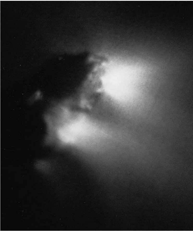
Fig. 2.7 The black heart of comet Halley
