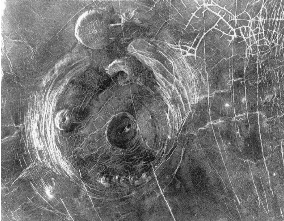
Fig. 7.21 Fotla Corona Large circular and oval structures with diameters of 200 to 1000 kilometers are called coronae. The one shown at the center of this Magellan image is known as Fotla Corona, about 200 kilometers across and named after the Celtic fertility goddess. It is located in a vast plain to the south of Aphrodite Terra, and is centered at 59 degrees south latitude and 164 degrees east longitude. Molten rock rising from the interior of the planet most likely explains the corona's circular shape, raised topography, complex fractures and associated volcanism. Just north ( top ) of this corona is a flat-topped pancake dome, about 35 kilometers in diameter, thought to have formed by the eruption of sluggish, pasty lava. Another pancake dome is located inside the western ( left ) part of the corona. There is also a smooth, flat region in the center of the corona, probably a relatively young lava flow. Complex fracture patterns like the one in the northeast ( top right ) of the image are often observed in association with coronae. (Courtesy of NASA/JPL.)
