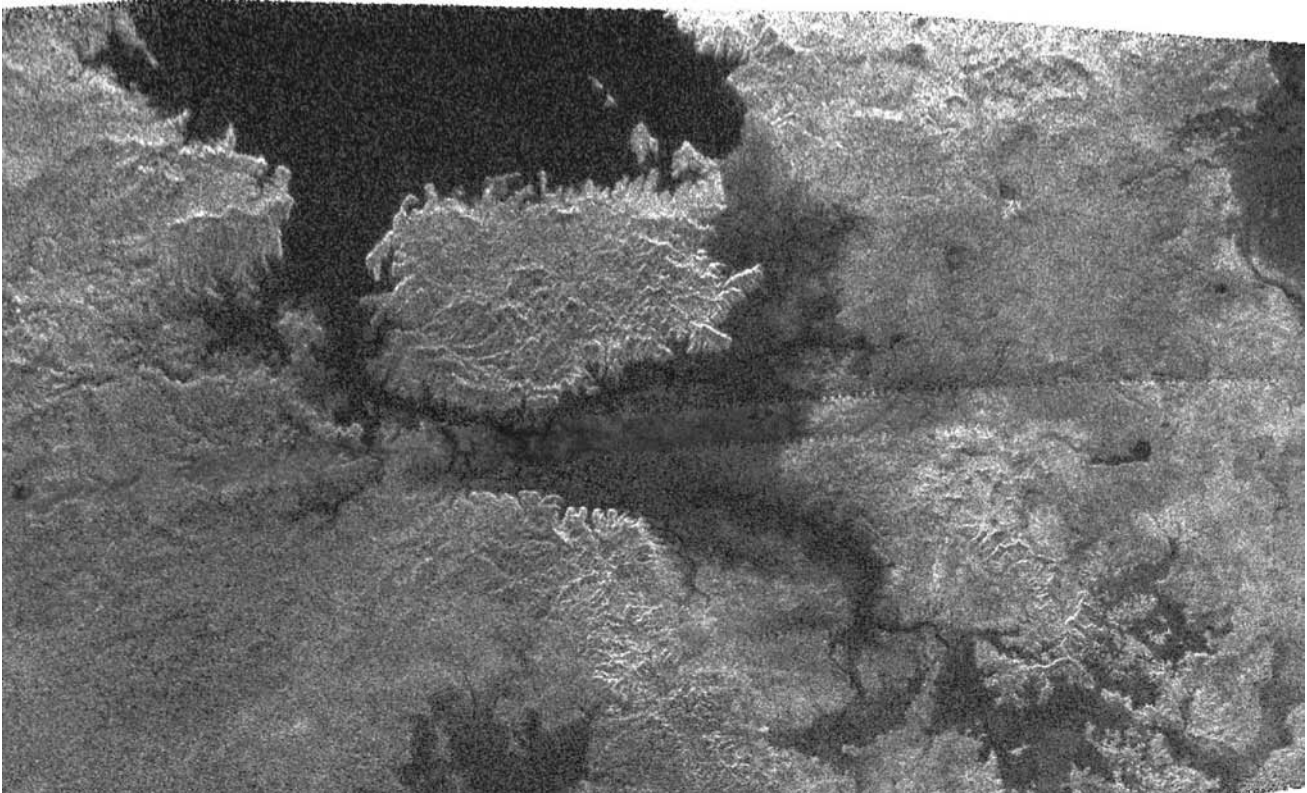
Fig. 10.26 Lakes of methane and ethane on Saturn's moon Titan A radar image shows a bright, central island in a dark, smooth lake, surrounded by a bright shoreline with numerous inlets. The island is about 90 kilometers across. This is one of many large lakes formed at high latitudes on Titan, with more in the northern polar regions than the southern ones. Seasonal rains of liquid methane and ethane probably fill these lakes. The radar instrument aboard Cassini obtained this image during a close south polar flyby on 22 February 2007. (Courtesy of NASA/JPL.)
