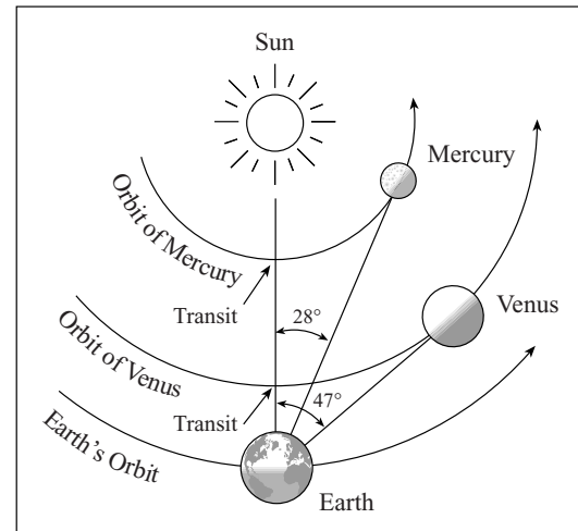
Fig. 6.1 Maximum elongation Unlike the planets that orbit the Sun beyond the Earth, Mercury and Venus can never be seen high in the sky in the dead of night. Because they are close to the Sun and inside Earth's orbit, these planets are always seen soon after sunset or shortly before sunrise, and they show phases much as the Moon does. The elongation of Mercury and Venus, or their angular distances from the Sun as viewed from the Earth, never exceeds 28 degrees and 47 degrees, respectively.
