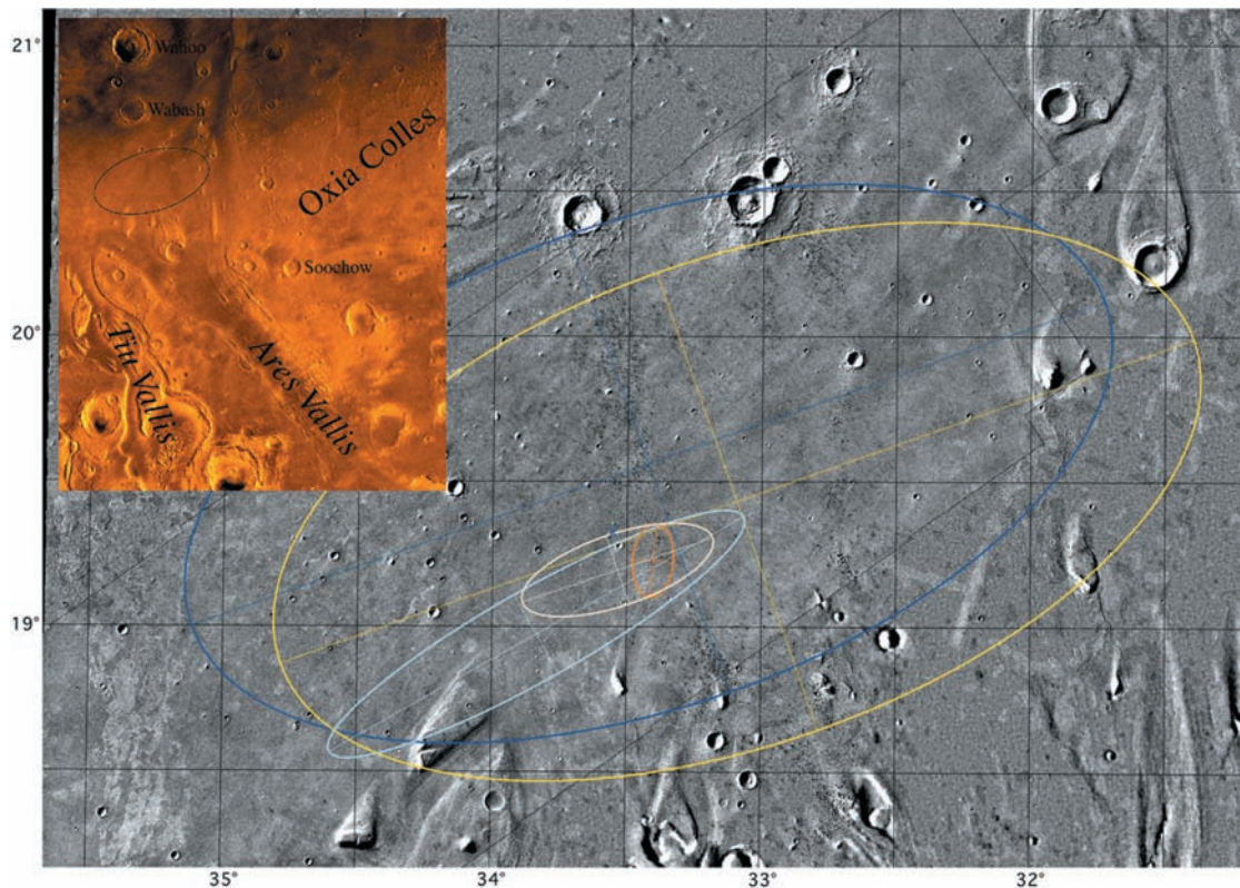
Fig. 2.14 Mars Pathfinder lands on an ancient flood plain About 3.7 billion years ago, great floods rushed out of the outflow channel, Ares Vallis, and emptied into the Chryse Planitia, or Plains of Gold, region of Mars ( color inset ). The flowing water carved out streamlined islands around craters ( top right ). This area was chosen as the Mars Pathfinder landing site for three reasons: it seemed safe, with no steep slopes or rough surfaces; it had a low elevation, which provided enough air density above the surface for a parachute to work; and it appeared to offer a variety of rock types deposited by the floods. The ellipses mark the area targeted for landing of Mars Pathfinder , as refined several times during the final approach to Mars. An X within the smallest ellipse marks the location of the lander at 19.33 degrees north and 33.55 degrees west. The site is about 850 kilometers southeast of the location of Viking 1 lander. (Courtesy of NASA/JPL.)
