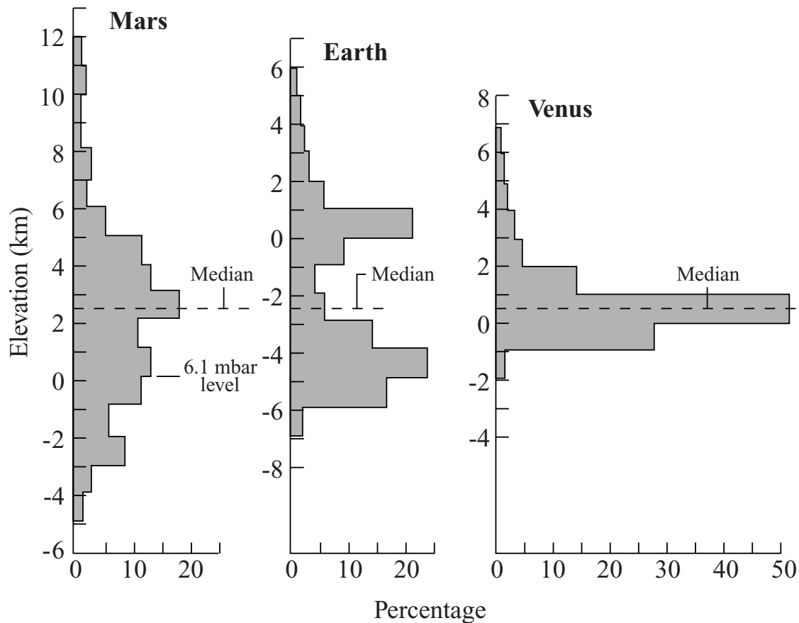
Fig. 7.11 Surface elevations for Earth, Venus and Mars Most places on Earth ( center ) stand near one of two prevailing levels, the high-standing continents or the low-lying ocean floors. In contrast, the surface of Venus ( right ) is unusually smooth and flat; about 60 percent of its terrain lies within 500 meters of the mean planetary radius of 6051.8 kilometers. A small percentage of its terrain consists of elevated highlands that are comparable in height to many continents on Earth. The surface features on Mars ( left ) are spread over a broader range of elevation than most of those on Venus; but the Martian surface elevations are not double-peaked as on Earth.
