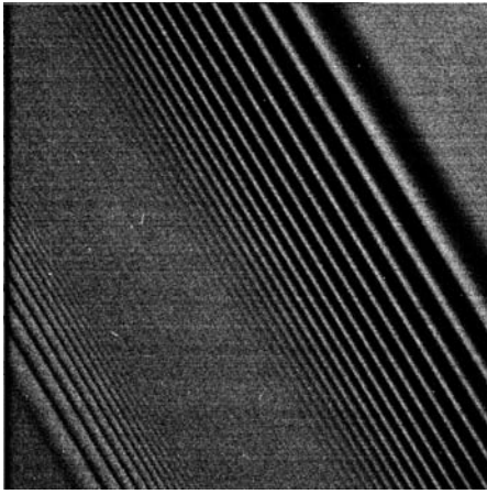
Fig. 10.15 Two waves in Saturn's rings Gaps and wave-like concentrations in ring particles are due to the gravitational influence of Saturn's moons. A small, nearby moon orbiting at varying distance from Saturn's rings is thought to produce waves of density, causing the ring particles to bunch together and disperse like the crests and troughs of ocean waves ( bottom left ). The gravity of a nearby moon can also produce a vertical wave in the ring particles, known as a bending wave ( upper right ). This image, which spans about 220 kilometers, was taken from the Cassini spacecraft on 29 October 2004. (Courtesy of NASA/JPL/SSI.)
