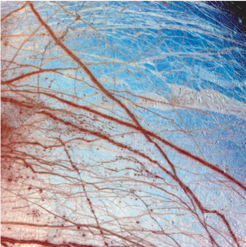
Fig. 2.36 Water oozes out from Jupiter's moon Europa A composite, color-enhanced image of the Minos Linea region of Jupiter's moon Europa, taken on 28 June 1996 by imaging cameras on Galileo . The icy plains, shown here in bluish hues, reflect different amounts of light, probably as the result of differences in the sizes of the ice grains. The long red cracks in the ice could mark the sites of liquid water oozing out from the warm interior of Europa. The area covered in this image is about 1.26 kilometers across. In Greek mythology, Minos is the son of Zeus and the king of Crete, who kept a monster named Minotaur in a labyrinth. Linea is a "dark or bright elongate marking". (Courtesy of NASA/JPL/U. Arizona.)
