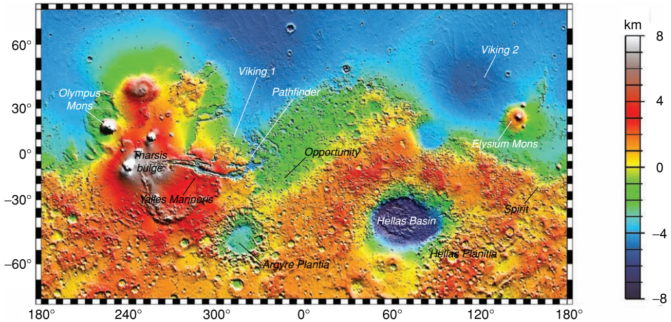
Fig. 8.13 Global topography of Mars By measuring the round-trip time of laser pulses bounced off the surface of Mars, the laser altimeter aboard the Mars Global Surveyor orbiter measured the altitude with a vertical accuracy of about 1 meter, providing this topographical map of Mars between latitudes of 65 degrees south (bottom) and 65 degrees north (top). The locations of five landing sites are labeled with the names of the landing spacecraft. This map portrays the great elevation difference between the northern, low-lying plains and the cratered southern highlands, and records the downhill direction that liquid water would flow. The red areas in the southern hemisphere are high regions, about 4 kilometers above the average surface height, and the blue regions of the northern hemisphere are low places, about 4 kilometers below the average height. The North Polar Basin, or Borealis Basin, is the large blue, low-lying area at the top of this topographical map; it covers about 40 percent of the planet. The map also shows the Tharsis bulge that lies near the Martian equator in the east longitude from 220 to 300 degrees. The bulge includes several major shield volcanoes, such as Olympus Mons. The huge Valles Marineris canyon system extends to the west of Tharsis. The giant Hellas impact basin, at 45 degrees south and 70 degrees east, is about 3000 kilometers across and lies about 9 kilometers deep. (Courtesy NASA/JPL/GSFC.)
