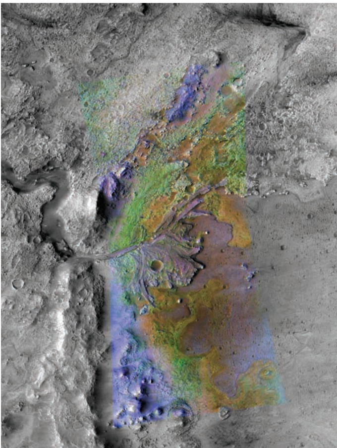
Fig. 8.22 Wet places on ancient Mars A color-enhanced image of a delta in Jezero Crater obtained from an instrument aboard the Mars Reconnaissance Orbiter (bottom), and a close-up of the central area (top). A system of river channels apparently eroded clay minerals (green) out of the highlands and concentrated them into a crater lake, forming the delta. The distribution of clays inside the ancient lakebed suggests that standing water persisted for thousands of years in this location, and that liquid water may have persisted for thousands to millions of years as the clay formed, albeit more than 3.5 billion years ago. [Courtesy of NASA/JPL/JHUAPL/MSSS/Brown University; Bethany L. Ehlmann and colleagues, Nature Geoscience 1, 355–358 (2008).]
