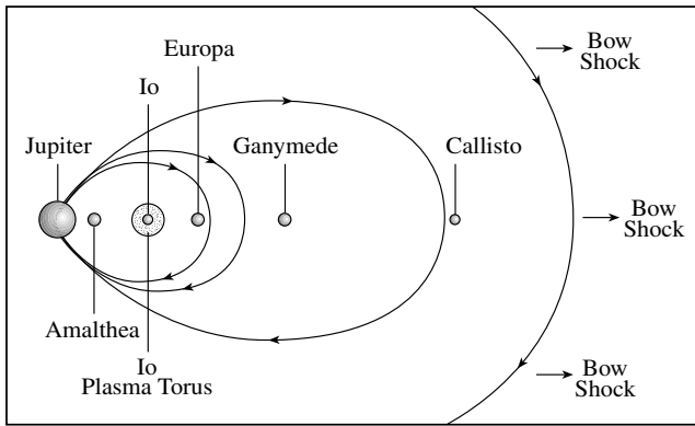
Fig. 3.18 Satellites within Jupiter's magnetic field This cross-section shows that the four Galilean satellites, Io, Europa, Ganymede and Callisto, are all embedded within Jupiter's magnetosphere. Small satellites orbit Jupiter within the orbit of Io, the innermost Galilean satellite. The outermost Galilean satellite, Callisto, orbits Jupiter near its bow shock. All of these satellites are being continuously bombarded with energetic charged particles that are trapped within Jupiter's magnetosphere. The distance from Jupiter to Callisto is 1.88 million ( 1.88 \times 10^6 ) kilometers, while the radius of the Sun is 0.696 million kilometers, so Jupiter's bow shock is bigger than the Sun.
