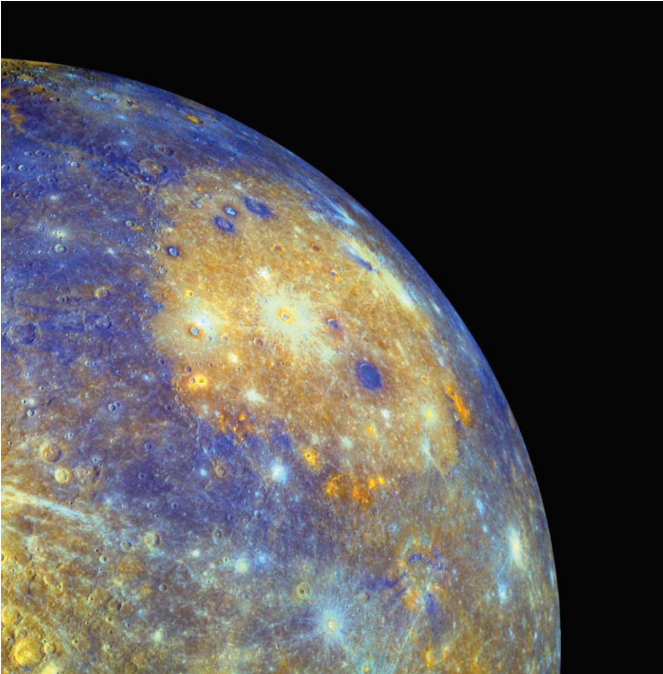
Fig. 2.22 Mercury's Caloris impact basin This false-color image shows Mercury's great Caloris impact basin as a large, circular orange feature in the center of the image. It was acquired on 14 January 2008 from the MESSENGER spacecraft. The smaller, bright orange spots just inside the rim of Caloris basin are thought to mark the location of volcanic features. The color variations in the surrounding plains indicate Mercury's variable surface composition. (Courtesy of NASA/JHUAPL/ASU/CIW/Science/AAAS.)
