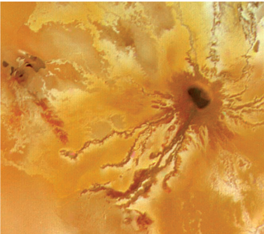
Fig. 2.34 Lava flows on Jupiter's satellite Io Numerous volcano calderas and lava flows were discovered on Jupiter's innermost large moon, Io, in 1979 using an instrument aboard the Voyager 1 spacecraft. This Voyager 1 image of Ra Patera, a large shield volcano, shows flows up to 300 kilometers long emanating from a dark volcanic vent. The diffuse reddish and orange colorations are probably surface deposits of sulfur compounds. The bright whitish patches probably consist of freshly deposited sulfur dioxide frost. Ra is an Egyptian Sun god. (Courtesy of NASA/JPL)
