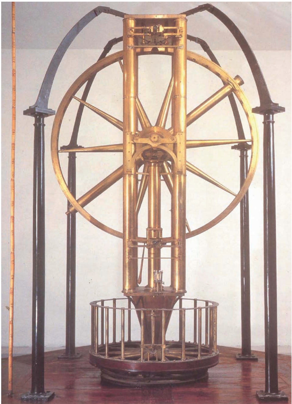
Fig. 1.15 The Palermo circle This instrument, built by Jesse Ramsden (1735–1800) of London, was used by Giuseppe Piazzi (1746–1826) to obtain precise measurements of stellar positions, with an accuracy of a few seconds of arc after observing each star for at least two nights. In the process, Piazzi unexpectedly discovered the first asteroid, 1 Ceres, in 1801. The telescope has a 7.5-cm objective lens. The altitude scale (5 feet in diameter) was read with the aid of two diametrically opposed micrometer microscopes; the azimuth scale (3 feet in diameter) was also read by means of a micrometer microscope.
