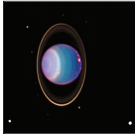
Fig. 11.1 The tilted planet Thin, spidery rings and several small moons encircle Uranus. The planet is tipped on its side, so its equator, rings and direction of rotation are almost perpendicular to the plane of the planet's orbital motion around the Sun. Storm clouds, found in the northern upper atmosphere (right) circle the planet at more than 500 kilometers per hour. The clouds are tinted pink in this false-color image to show that it was taken at infrared wavelengths, but the clouds are white in visible light. This image was taken on 8 August 1998 from the Hubble Space Telescope . (Courtesy of NASA/JPL/STSCI.)
