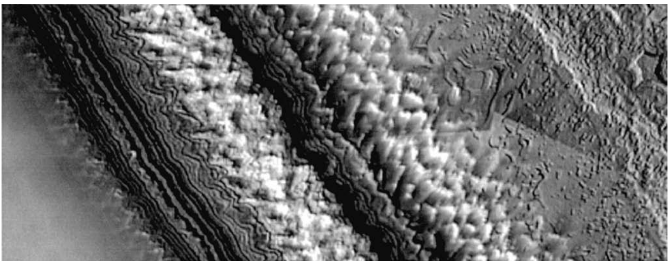
Fig. 8.12 Layered polar terrain on Mars These layers, exposed in the south polar residual cap of Mars, consist of bright ice and dark fine dust deposited over millions of years. The layered terrain in both the north and south residual caps is thought to contain detailed records of the climate history of Mars. This image covers an area of 10 by 4 kilometers. It was taken from the Mars Global Surveyor in October 1999 at 87 degrees south and 10 degrees west, near the central region of the residual south polar cap. (Courtesy of NASA/JPL/MSSS.)
