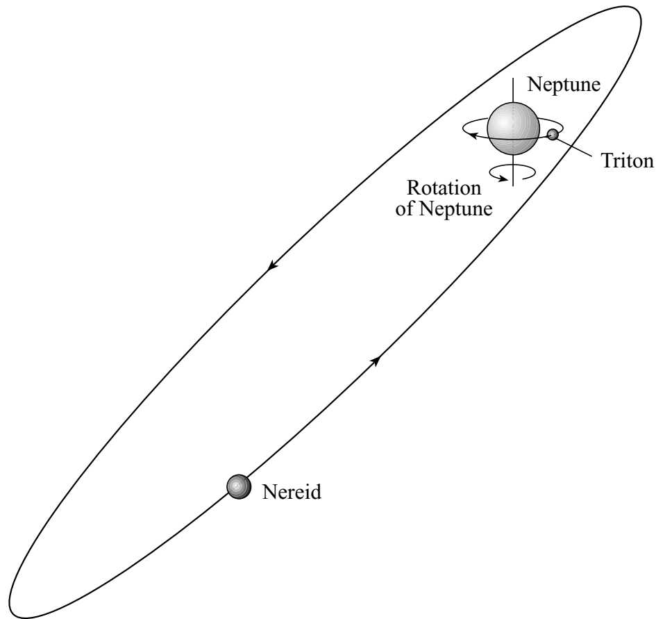
Fig. 11.13 Neptune's odd satellites Nereid, the outermost of Neptune's satellites, travels in a highly inclined, eccentric orbit, in the same direction as that of the planet's rotation. Triton, the largest satellite of Neptune, travels around Neptune in a circular orbit, but, unlike any other largest satellite of the giant planets, it travels in the opposite retrograde direction to the rotation of Neptune. In addition, careful analysis of Triton's motions shows that the satellite is in a decaying orbit and is slowly being pulled toward Neptune.
