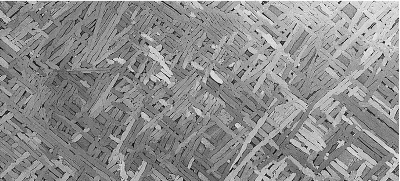
Fig. 12.24 Widmanstätten pattern When polished and etched with acid, an iron meteorite displays this distinctive Widmanstätten pattern produced by crystals of two different iron-nickel alloys. The pattern provides evidence that this meteorite was once buried within a parent body between 50 and 200 kilometers in radius. This sliced specimen is about 0.05 meters across. (Courtesy of the Smithsonian Institution.)
